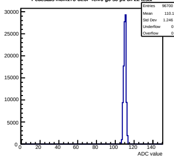
Pedestals mcm173-6E0F-refV6-g0-s0-p1 ch 22 test1
