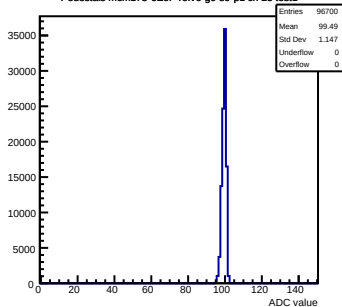
Pedestals mcm173-6E0F-refV6-g0-s0-p1 ch 25 test1
