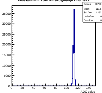
Pedestals mcm173-GEOf-refV6-g0-s0-p1 ch 82 test1
