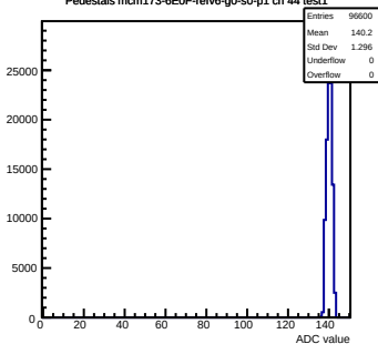
Pedestals mcm173-6E0F-refV6-g0-s0-p1 ch 44 test1
