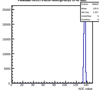
Pedestals mcm173-6E0F-refV6-g0-s0-p1 ch 42 test1
