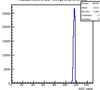
Pedestals mcm173-6E0F-refV6-g0-s0-p1 ch 21 test1
