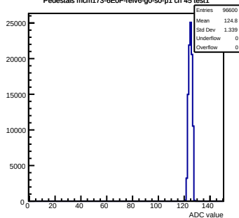
Pedestals mcm173-6E0F-refV6-g0-s0-p1 ch 45 test1
