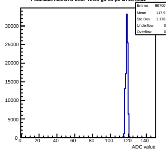
Pedestals mcm173-6E0F-refV6-g0-s0-p1 ch 23 test1
