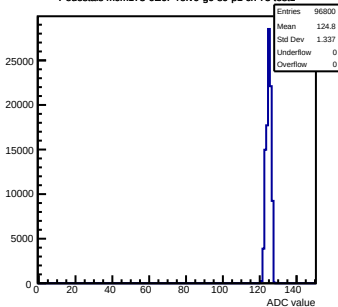
Pedestals mcm173-6E0F-refV6-g0-s0-p1 ch 75 test1
