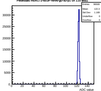
Pedestals mcm173-6E0F-rev6-g0-s0-p1 ch 115 test1
