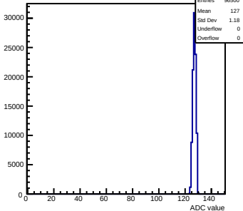
Pedestals mcm173-6E0F-rev6-g0-s0-p1 ch 126 test1
