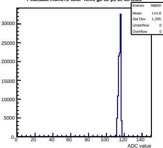
Pedestals mcm173-6E0F-refV6-g0-s0-p1 ch 65 test1
