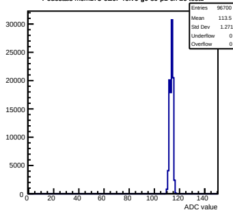
Pedestals mcm173-6E0F-refV6-g0-s0-p1 ch 26 test1
