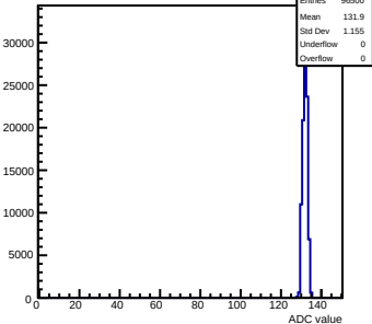
Pedestals mcm173-6E0F-rev6-g0-s0-p1 ch 125 test1
