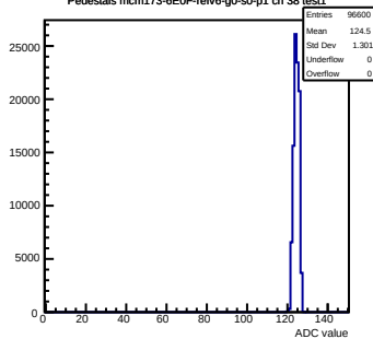
Pedestals mcm173-6E0F-refV6-g0-s0-p1 ch 38 test1
