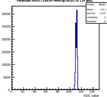
Pedestals mcm173-6E0F-rev6-g0-s0-p1 ch 114 test1
