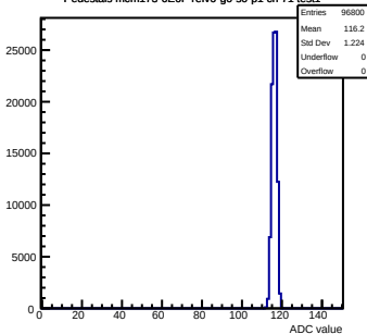
Pedestals mcm173-6E0F-refV6-g0-s0-p1 ch 71 test1
