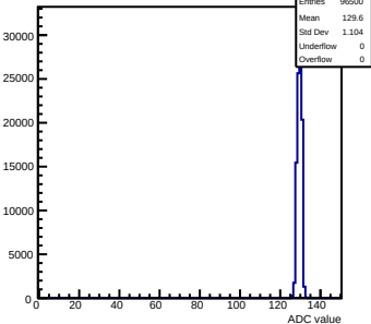
Pedestals mcm173-6E0F-rev6-g0-s0-p1 ch 121 test1
