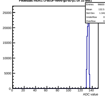
Pedestals mcm173-6E0F-refV6-g0-s0-p1 ch 33 test1
