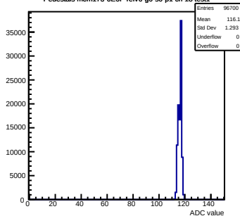
Pedestals mcm173-6E0F-refV6-g0-s0-p1 ch 18 test1
