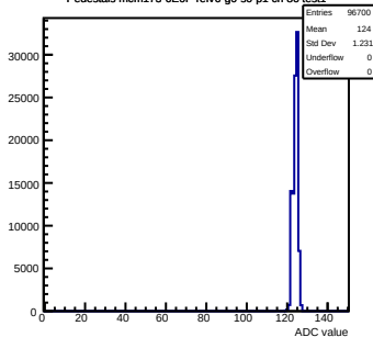
Pedestals mcm173-GEOf-refV6-g0-s0-p1 ch 86 test1
