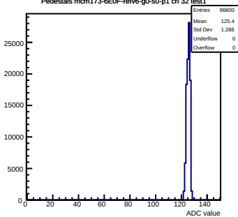
Pedestals mcm173-6E0F-refV6-g0-s0-p1 ch 32 test1
