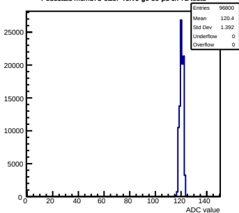
Pedestals mcm173-6E0F-refV6-g0-s0-p1 ch 72 test1
