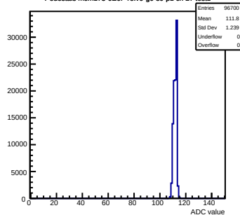
Pedestals mcm173-6E0F-refV6-g0-s0-p1 ch 27 test1
