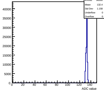
Pedestals mcm173-6E0F-rev6-g0-s0-p1 ch 119 test1
