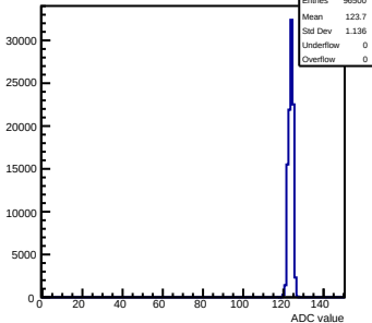
Pedestals mcm173-6E0F-rev6-g0-s0-p1 ch 118 test1
