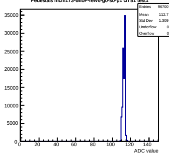
Pedestals mcm173-GEOf-refV6-g0-s0-p1 ch 81 test1
