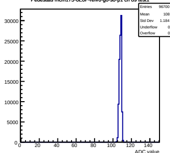
Pedestals mcm173-GEOf-refV6-g0-s0-p1 ch 89 test1
