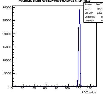
Pedestals mcm173-6E0F-refV6-g0-s0-p1 ch 34 test1
