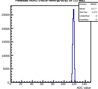
Pedestals mcm173-6E0F-rev6-g0-s0-p1 ch 112 test1
