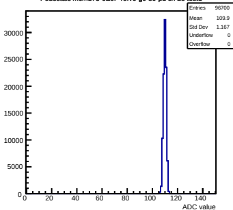
Pedestals mcm173-6E0F-refV6-g0-s0-p1 ch 28 test1
