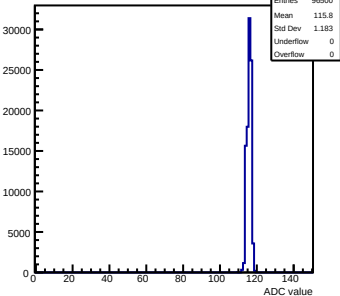
Pedestals mcm173-6E0F-rev6-g0-s0-p1 ch 117 test1
