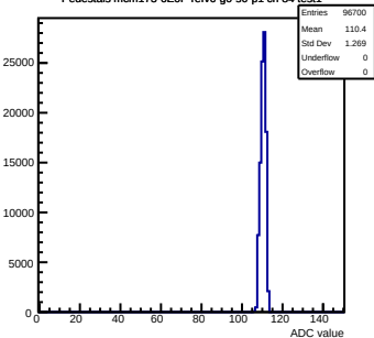
Pedestals mcm173-GEOf-refV6-g0-s0-p1 ch 84 test1
