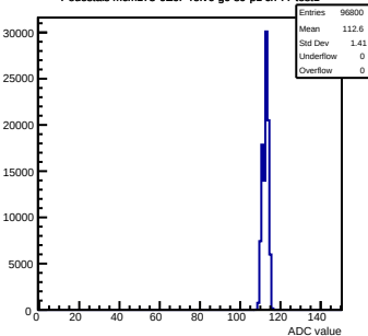
Pedestals mcm173-6E0F-refV6-g0-s0-p1 ch 77 test1
