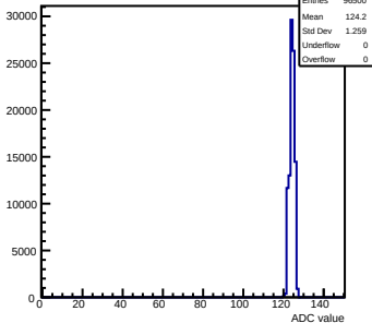
Pedestals mcm173-6E0F-rev6-g0-s0-p1 ch 116 test1
