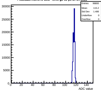
Pedestals mcm173-6E0F-refV6-g0-s0-p1 ch 64 test1
