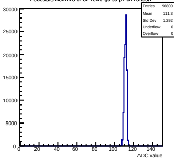
Pedestals mcm173-6E0F-refV6-g0-s0-p1 ch 70 test1
