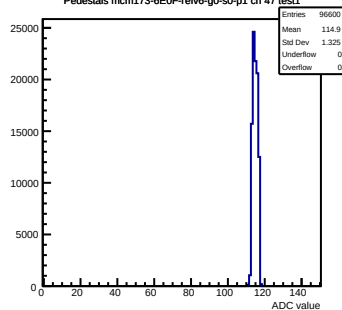
Pedestals mcm173-6E0F-refV6-g0-s0-p1 ch 47 test1
