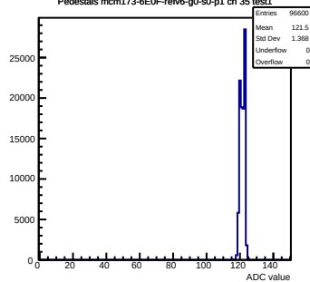
Pedestals mcm173-6E0F-refV6-g0-s0-p1 ch 35 test1
