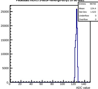
Pedestals mcm173-GEOf-refV6-g0-s0-p1 ch 80 test1
