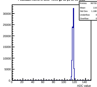
Pedestals mcm173-6E0F-refV6-g0-s0-p1 ch 19 test1
