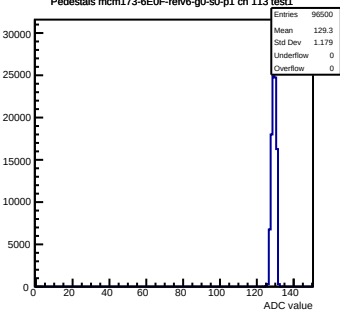
Pedestals mcm173-6E0F-rev6-g0-s0-p1 ch 113 test1
