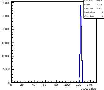
Pedestals mcm173-6E0F-rev6-g0-s0-p1 ch 124 test1
