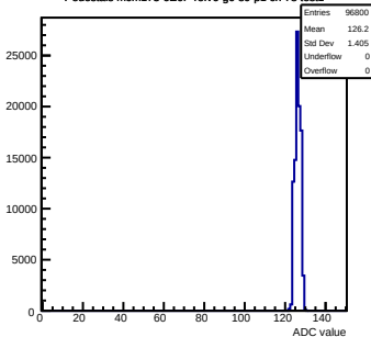
Pedestals mcm173-6E0F-refV6-g0-s0-p1 ch 78 test1
