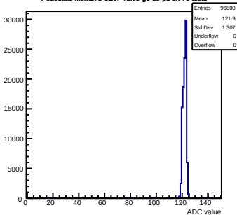
Pedestals mcm173-6E0F-refV6-g0-s0-p1 ch 79 test1
