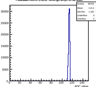
Pedestals mcm173-GEOf-refV6-g0-s0-p1 ch 88 test1
