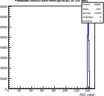
Pedestals mcm20-300F-refV0-g0-s0-p1 ch 101 test1
