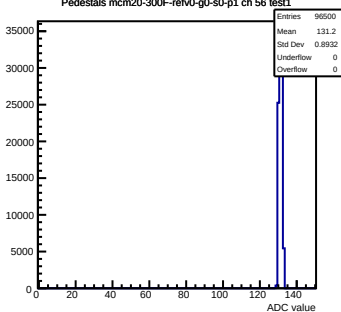
Pedestals mcm20-300F-refV0-g0-s0-p1 ch 56 test1
