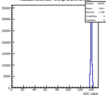
Pedestals mcm20-300F-refV0-g0-s0-p1 ch 80 test1
