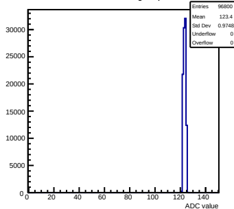
Pedestals mcm20-300F-refV0-g0-s0-p1 ch 78 test1
