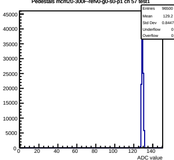
Pedestals mcm20-300F-refV0-g0-s0-p1 ch 57 test1
