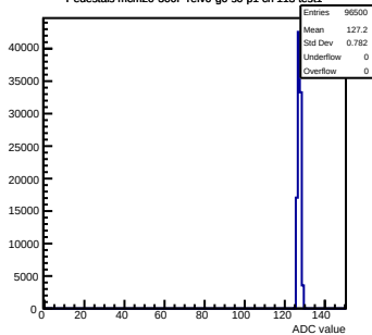
Pedestals mcm20-300F-refV0-g0-s0-p1 ch 113 test1
