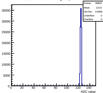
Pedestals mcm20-300F-refV0-g0-s0-p1 ch 41 test1
