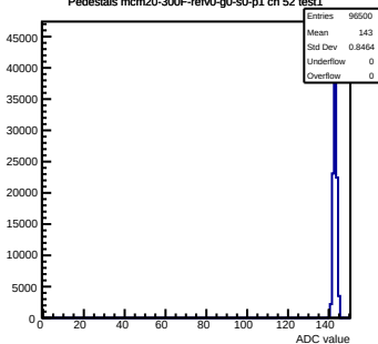
Pedestals mcm20-300F-refV0-g0-s0-p1 ch 52 test1
