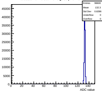
Pedestals mcm20-300F-refV0-g0-s0-p1 ch 45 test1
