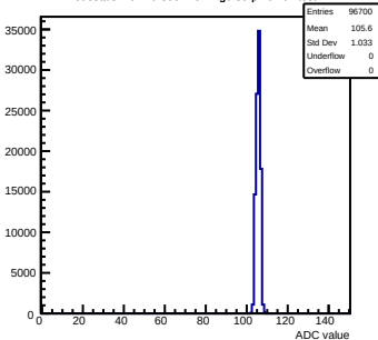
Pedestals mcm20-300F-refv1-g0-s0-p1 ch 94 test1
