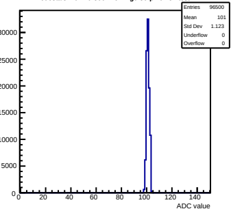
Pedestals mcm20-300F-refv1-g0-s0-p1 ch 57 test1
