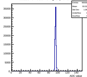
Pedestals mcm20-300F-refv1-g0-s0-p1 ch 59 test1
