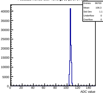
Pedestals mcm20-300F-refv1-g0-s0-p1 ch 84 test1
