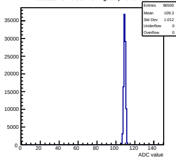
Pedestals mcm20-300F-refv1-g0-s0-p1 ch 62 test1
