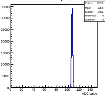
Pedestals mcm20-300F-refv1-g0-s0-p1 ch 92 test1
