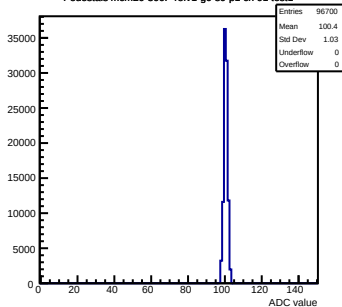
Pedestals mcm20-300F-refv1-g0-s0-p1 ch 91 test1
