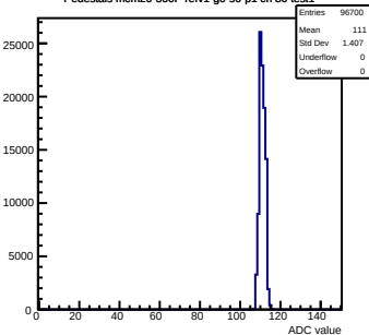
Pedestals mcm20-300F-refv1-g0-s0-p1 ch 80 test1
