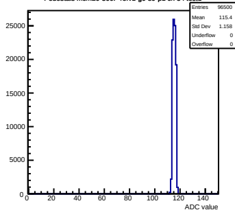
Pedestals mcm20-300F-refv1-g0-s0-p1 ch 54 test1
