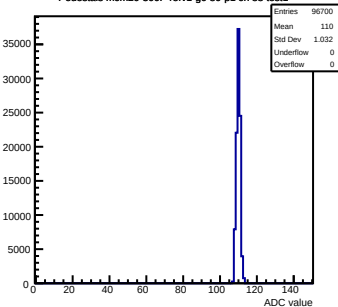
Pedestals mcm20-300F-refv1-g0-s0-p1 ch 88 test1
