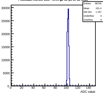
Pedestals mcm20-300F-refv1-g0-s0-p1 ch 82 test1
