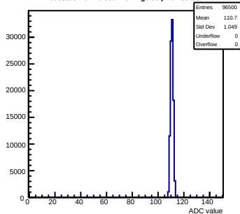
Pedestals mcm20-300F-refv1-g0-s0-p1 ch 58 test1
