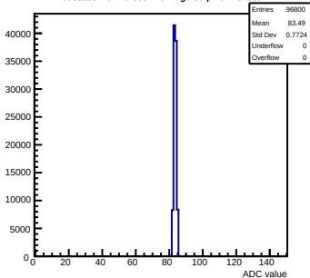
Pedestals mcm20-300F-refv2-g0-s0-p1 ch 76 test1
