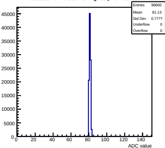
Pedestals mcm20-300F-refv2-g0-s0-p1 ch 104 test1
