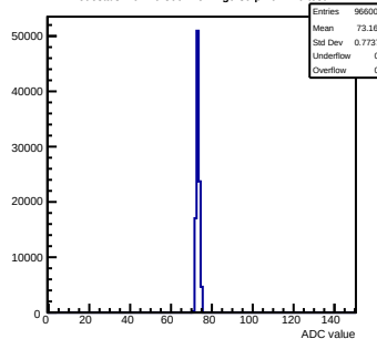
Pedestals mcm20-300F-refv2-g0-s0-p1 ch 106 test1
