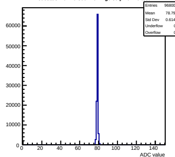
Pedestals mcm20-300F-refv2-g0-s0-p1 ch 79 test1
