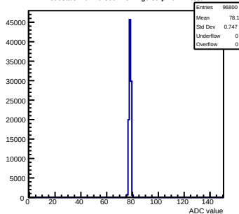
Pedestals mcm20-300F-refv2-g0-s0-p1 ch 74 test1
