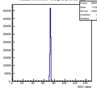
Pedestals mcm20-300F-refv2-g0-s0-p1 ch 98 test1
