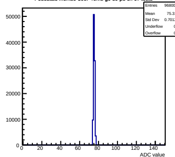
Pedestals mcm20-300F-refv2-g0-s0-p1 ch 67 test1
