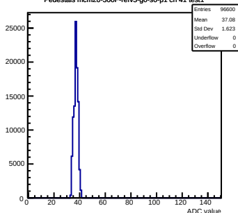
Pedestals mcm20-300F-refv3-g0-s0-p1 ch 41 test1
