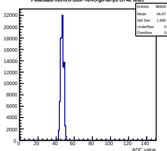
Pedestals mcm20-300F-refv3-g0-s0-p1 ch 42 test1
