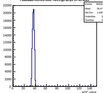
Pedestals mcm20-300F-refv3-g0-s0-p1 ch 43 test1
