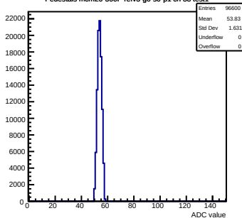
Pedestals mcm20-300F-refv3-g0-s0-p1 ch 38 test1
