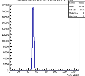
Pedestals mcm20-300F-refv3-g0-s0-p1 ch 37 test1
