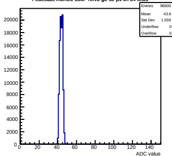
Pedestals mcm20-300F-refv3-g0-s0-p1 ch 34 test1
