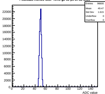
Pedestals mcm20-300F-refv3-g0-s0-p1 ch 33 test1
