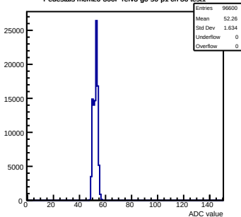
Pedestals mcm20-300F-refv3-g0-s0-p1 ch 36 test1
