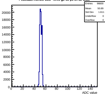
Pedestals mcm20-300F-refv3-g0-s0-p1 ch 32 test1
