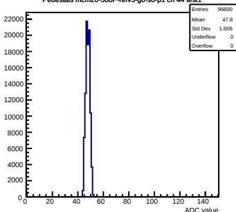
Pedestals mcm20-300F-refv3-g0-s0-p1 ch 44 test1
