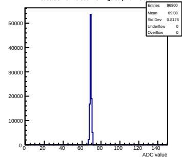
Pedestals mcm20-300F-refv4-g0-s0-p1 ch 75 test1
