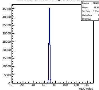
Pedestals mcm20-300F-refv4-g0-s0-p1 ch 103 test1
