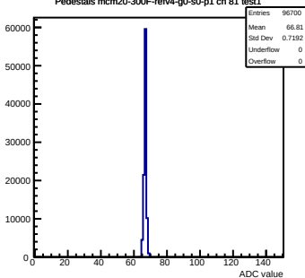
Pedestals mcm20-300F-refv4-g0-s0-p1 ch 81 test1
