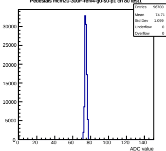
Pedestals mcm20-300F-refv4-g0-s0-p1 ch 80 test1
