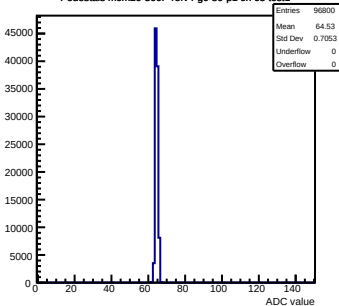
Pedestals mcm20-300F-refv4-g0-s0-p1 ch 65 test1
