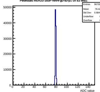
Pedestals mcm20-300F-refv4-g0-s0-p1 ch 83 test1
