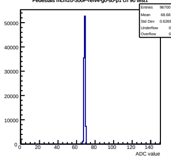
Pedestals mcm20-300F-refv4-g0-s0-p1 ch 90 test1
