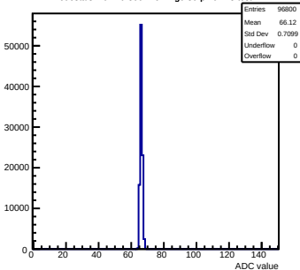
Pedestals mcm20-300F-refv4-g0-s0-p1 ch 73 test1
