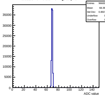
Pedestals mcm20-300F-refv4-g0-s0-p1 ch 111 test1
