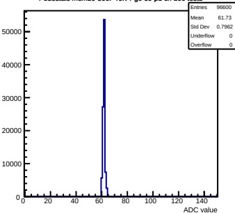
Pedestals mcm20-300F-refv4-g0-s0-p1 ch 100 test1
