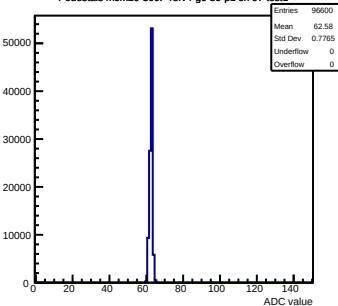
Pedestals mcm20-300F-refv4-g0-s0-p1 ch 97 test1
