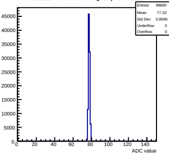
Pedestals mcm20-300F-refv4-g0-s0-p1 ch 105 test1
