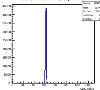
Pedestals mcm20-300F-refv4-g0-s0-p1 ch 99 test1
