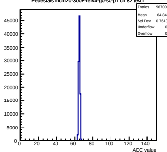
Pedestals mcm20-300F-refv4-g0-s0-p1 ch 82 test1
