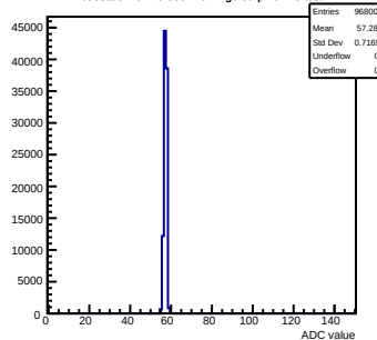
Pedestals mcm20-300F-refv4-g0-s0-p1 ch 78 test1
