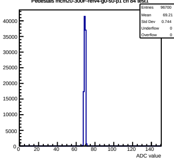
Pedestals mcm20-300F-refv4-g0-s0-p1 ch 84 test1
