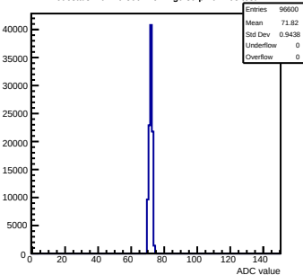
Pedestals mcm20-300F-refv4-g0-s0-p1 ch 108 test1
