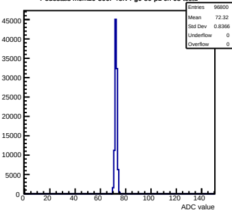
Pedestals mcm20-300F-refv4-g0-s0-p1 ch 68 test1
