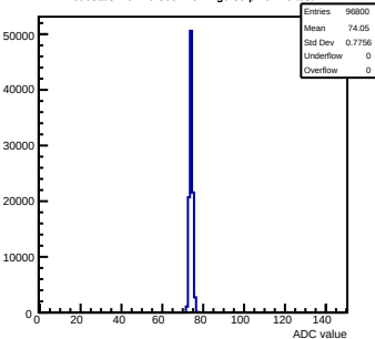
Pedestals mcm20-300F-refv4-g0-s0-p1 ch 76 test1
