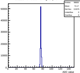
Pedestals mcm20-300F-refv4-g0-s0-p1 ch 104 test1
