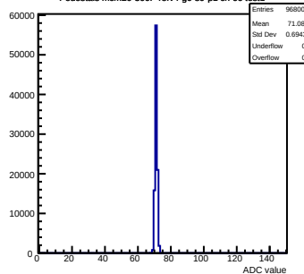
Pedestals mcm20-300F-refv4-g0-s0-p1 ch 66 test1
