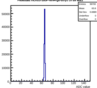
Pedestals mcm20-300F-refv4-g0-s0-p1 ch 89 test1
