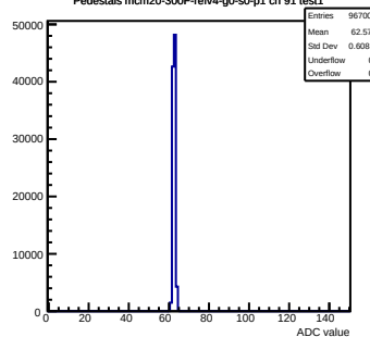
Pedestals mcm20-300F-refv4-g0-s0-p1 ch 91 test1
