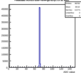
Pedestals mcm20-300F-refv4-g0-s0-p1 ch 92 test1
