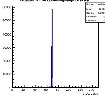
Pedestals mcm20-300F-refv4-g0-s0-p1 ch 94 test1
