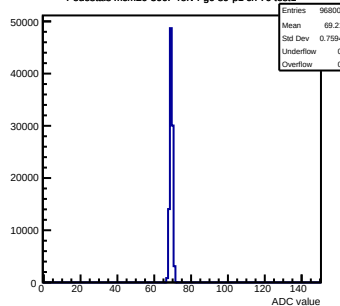
Pedestals mcm20-300F-refv4-g0-s0-p1 ch 70 test1
