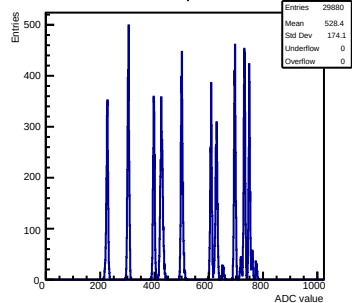
Pulse mcm 0 chip 3 chan 2 test1
