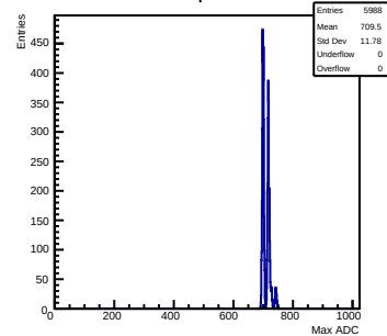
Max mcm 0 chip 3 chan 14 test1
