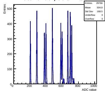
Pulse mcm 0 chip 3 chan 14 test1
