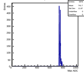
Max mcm 0 chip 3 chan 2 test1
