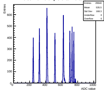
Pulse mcm 0 chip 3 chan 10 test1
