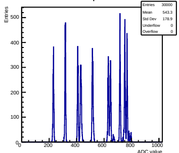
Pulse mcm 0 chip 0 chan 9 test1
