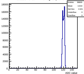
Pedestals mcm30-1A12-refV0-g0-s0-p1 ch 37 test1
