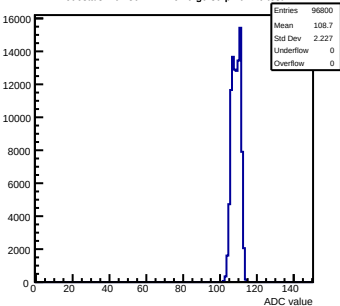
Pedestals mcm30-1A12-refV0-g0-s0-p1 ch 76 test1
