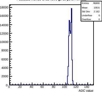
Pedestals mcm30-1A12-refV0-g0-s0-p1 ch 70 test1
