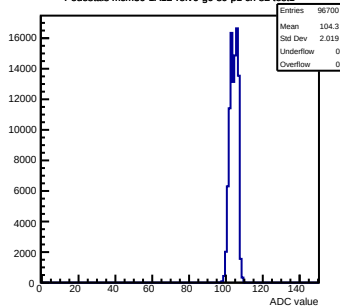
Pedestals mcm30-1A12-refV0-g0-s0-p1 ch 82 test1
