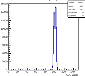
Pedestals mcm30-1A12-refV0-g0-s0-p1 ch 77 test1
