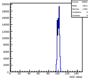
Pedestals mcm30-1A12-refV0-g0-s0-p1 ch 15 test1
