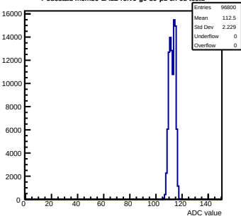
Pedestals mcm30-1A12-refV0-g0-s0-p1 ch 68 test1
