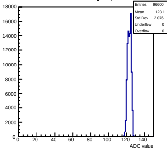
Pedestals mcm30-1A12-refV0-g0-s0-p1 ch 39 test1
