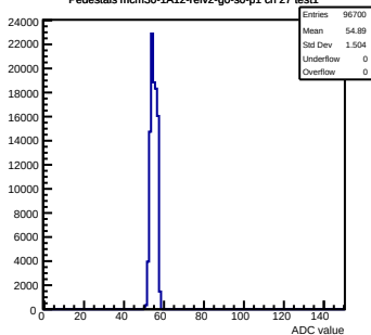
Pedestals mcm30-1A12-refv2-g0-s0-p1 ch 27 test1
