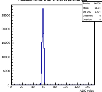
Pedestals mcm30-1A12-refv2-g0-s0-p1 ch 18 test1
