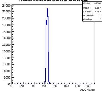
Pedestals mcm30-1A12-refv2-g0-s0-p1 ch 19 test1
