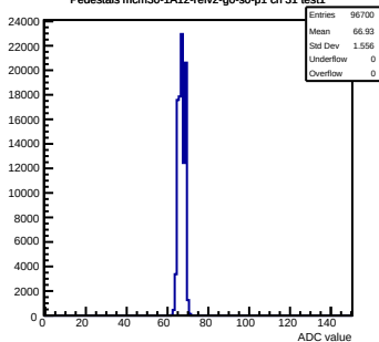
Pedestals mcm30-1A12-refv2-g0-s0-p1 ch 31 test1
