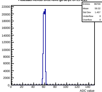
Pedestals mcm30-1A12-refv2-g0-s0-p1 ch 21 test1
