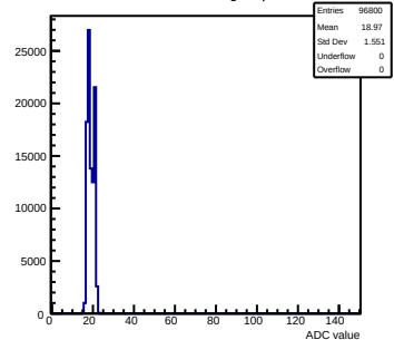
Pedestals mcm30-1A12-refv3-g0-s0-p1 ch 75 test1
