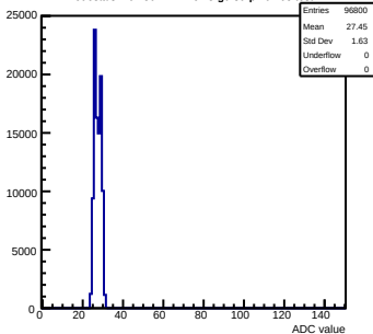
Pedestals mcm30-1A12-refv3-g0-s0-p1 ch 68 test1
