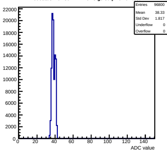
Pedestals mcm30-1A12-refv3-g0-s0-p1 ch 64 test1
