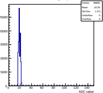
Pedestals mcm30-1A12-refv3-g0-s0-p1 ch 73 test1
