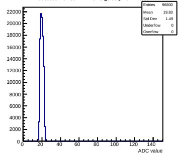
Pedestals mcm30-1A12-refv3-g0-s0-p1 ch 71 test1
