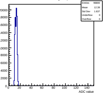
Pedestals mcm30-1A12-refv3-g0-s0-p1 ch 77 test1
