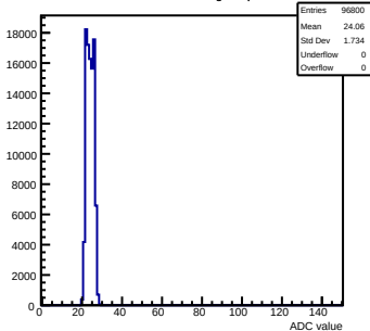
Pedestals mcm30-1A12-refv3-g0-s0-p1 ch 72 test1
