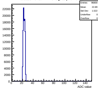
Pedestals mcm30-1A12-refv3-g0-s0-p1 ch 70 test1
