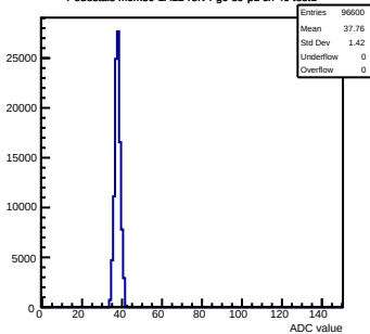
Pedestals mcm30-1A12-refv4-g0-s0-p1 ch 40 test1
