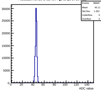
Pedestals mcm30-1A12-refv4-g0-s0-p1 ch 36 test1
