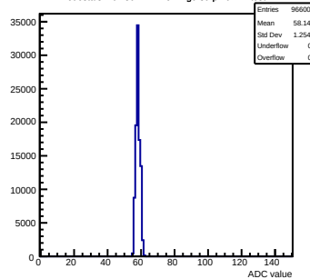
Pedestals mcm30-1A12-refv4-g0-s0-p1 ch 47 test1
