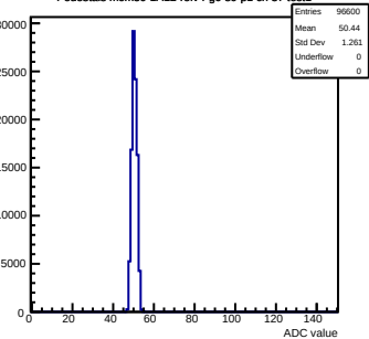
Pedestals mcm30-1A12-refv4-g0-s0-p1 ch 37 test1
