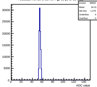
Pedestals mcm30-1A12-refv4-g0-s0-p1 ch 38 test1
