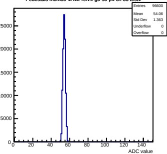
Pedestals mcm30-1A12-refv4-g0-s0-p1 ch 33 test1
