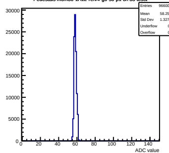
Pedestals mcm30-1A12-refv4-g0-s0-p1 ch 35 test1
