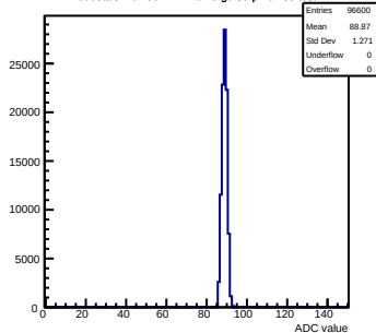
Pedestals mcm30-1A12-refv5-g0-s0-p1 ch 34 test1
