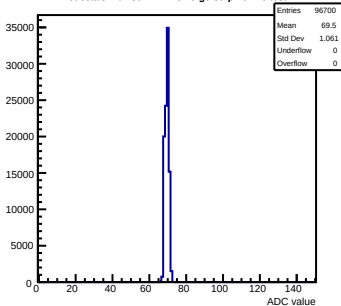
Pedestals mcm30-1A12-refv5-g0-s0-p1 ch 28 test1
