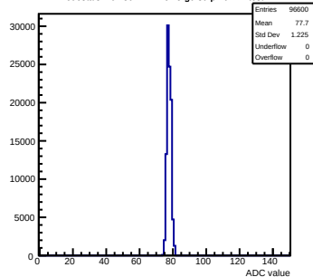
Pedestals mcm30-1A12-refv5-g0-s0-p1 ch 41 test1
