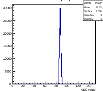
Pedestals mcm30-1A12-refv5-g0-s0-p1 ch 37 test1
