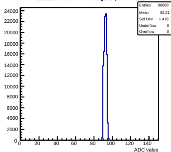
Pedestals mcm30-1A12-refv5-g0-s0-p1 ch 42 test1
