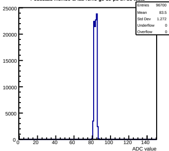
Pedestals mcm30-1A12-refv5-g0-s0-p1 ch 16 test1
