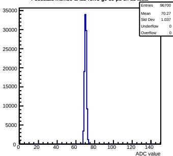
Pedestals mcm30-1A12-refv5-g0-s0-p1 ch 18 test1
