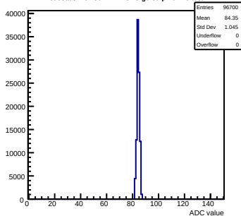
Pedestals mcm30-1A12-refv5-g0-s0-p1 ch 29 test1
