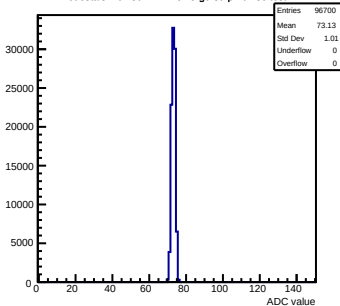
Pedestals mcm30-1A12-refv5-g0-s0-p1 ch 30 test1
