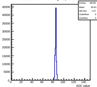
Pedestals mcm30-1A12-refv5-g0-s0-p1 ch 31 test1
