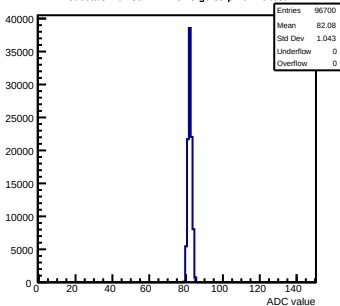
Pedestals mcm30-1A12-refv5-g0-s0-p1 ch 26 test1
