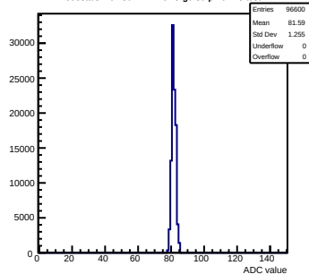
Pedestals mcm30-1A12-refv5-g0-s0-p1 ch 39 test1
