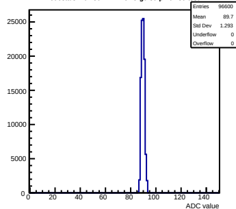
Pedestals mcm30-1A12-refv5-g0-s0-p1 ch 35 test1
