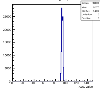
Pedestals mcm30-1A12-refv5-g0-s0-p1 ch 47 test1
