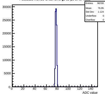
Pedestals mcm30-1A12-refv5-g0-s0-p1 ch 17 test1
