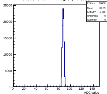
Pedestals mcm30-1A12-refv5-g0-s0-p1 ch 33 test1
