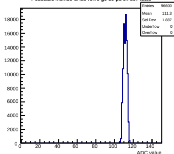
Pedestals mcm30-1A12-relv6-g0-s0-p1 ch 107 test1
