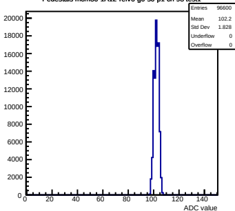
Pedestals mcm30-1A12-relv6-g0-s0-p1 ch 98 test1
