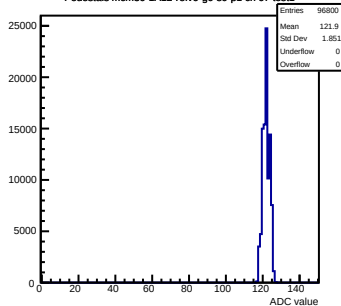
Pedestals mcm30-1A12-refv6-g0-s0-p1 ch 67 test1
