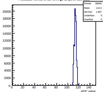
Pedestals mcm30-1A12-relv6-g0-s0-p1 ch 111 test1
