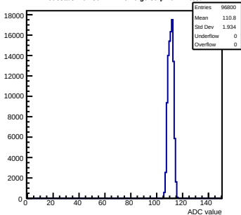
Pedestals mcm30-1A12-refv6-g0-s0-p1 ch 72 test1
