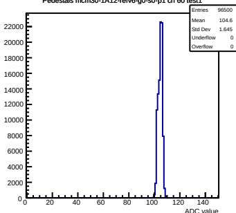
Pedestals mcm30-1A12-refv6-g0-s0-p1 ch 60 test1
