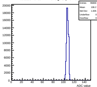
Pedestals mcm30-1A12-refv6-g0-s0-p1 ch 75 test1
