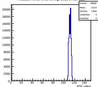
Pedestals mcm30-1A12-relv6-g0-s0-p1 ch 109 test1
