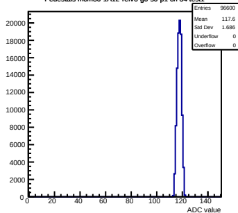
Pedestals mcm30-1A12-refv6-g0-s0-p1 ch 34 test1
