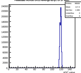
Pedestals mcm30-1A12-refv6-g0-s0-p1 ch 57 test1
