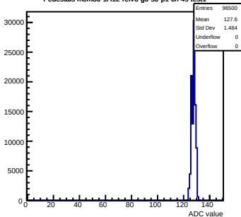
Pedestals mcm30-1A12-refv6-g0-s0-p1 ch 49 test1
