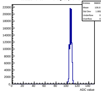
Pedestals mcm30-1A12-refv6-g0-s0-p1 ch 73 test1
