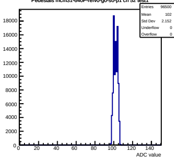
Pedestals mcm31-640F-refV0-g0-s0-p1 ch 52 test1
