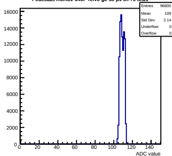
Pedestals mcm31-640F-refV0-g0-s0-p1 ch 70 test1
