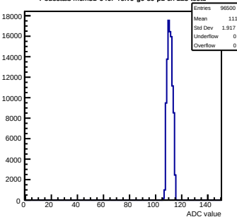
Pedestals mcm31-640F-refV0-g0-s0-p1 ch 125 test1
