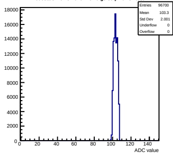
Pedestals mcm31-640F-refV0-g0-s0-p1 ch 31 test1
