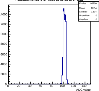
Pedestals mcm31-640F-refV0-g0-s0-p1 ch 17 test1
