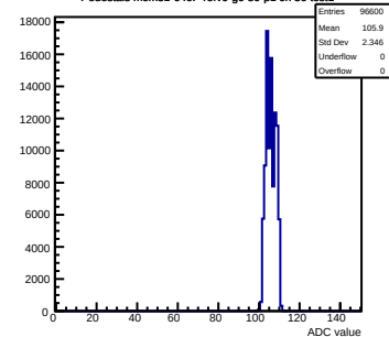
Pedestals mcm31-640F-refV0-g0-s0-p1 ch 36 test1
