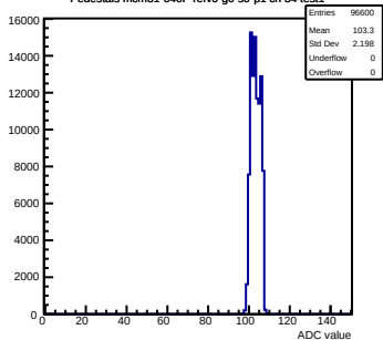
Pedestals mcm31-640F-refV0-g0-s0-p1 ch 34 test1
