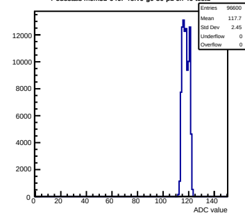
Pedestals mcm31-640F-refV0-g0-s0-p1 ch 40 test1
