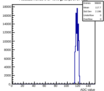
Pedestals mcm31-640F-refV0-g0-s0-p1 ch 37 test1
