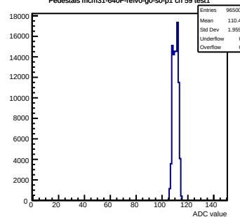
Pedestals mcm31-640F-refV0-g0-s0-p1 ch 59 test1
