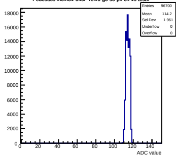
Pedestals mcm31-640F-refV0-g0-s0-p1 ch 19 test1
