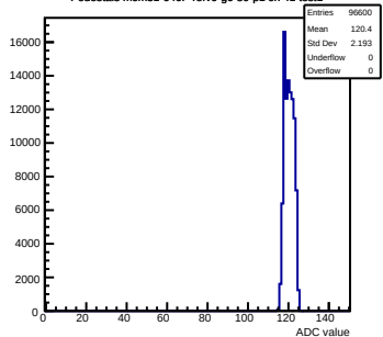
Pedestals mcm31-640F-refV0-g0-s0-p1 ch 41 test1
