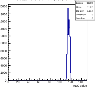
Pedestals mcm31-640F-refV0-g0-s0-p1 ch 21 test1
