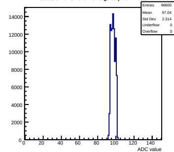
Pedestals mcm31-640F-refV0-g0-s0-p1 ch 44 test1
