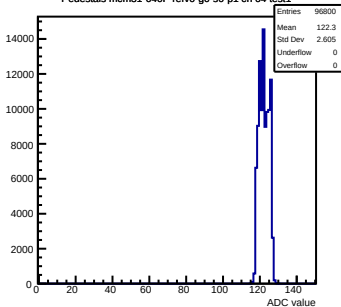
Pedestals mcm31-640F-refV0-g0-s0-p1 ch 64 test1
