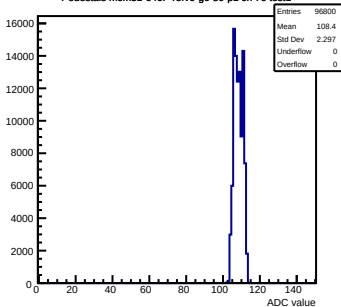
Pedestals mcm31-640F-refV0-g0-s0-p1 ch 76 test1
