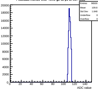
Pedestals mcm31-640F-refV0-g0-s0-p1 ch 117 test1
