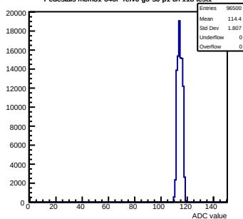
Pedestals mcm31-640F-refV0-g0-s0-p1 ch 118 test1
