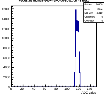
Pedestals mcm31-640F-refV0-g0-s0-p1 ch 48 test1
