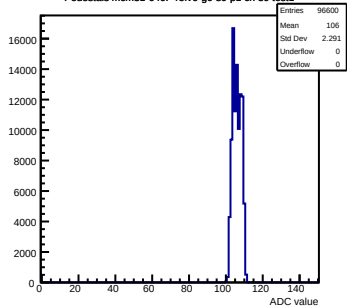
Pedestals mcm31-640F-refV0-g0-s0-p1 ch 39 test1
