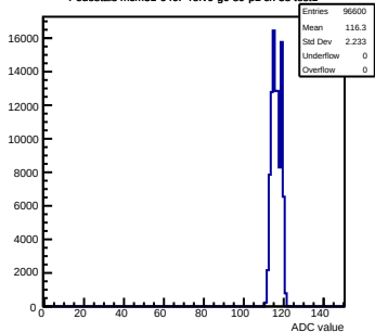
Pedestals mcm31-640F-refV0-g0-s0-p1 ch 38 test1
