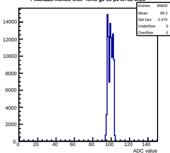
Pedestals mcm31-640F-refV0-g0-s0-p1 ch 68 test1
