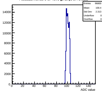
Pedestals mcm31-640F-refV0-g0-s0-p1 ch 75 test1
