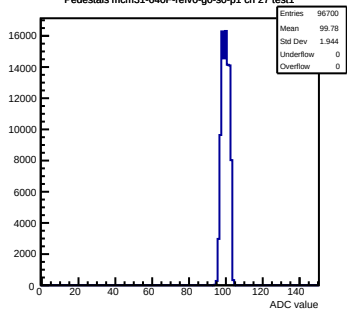
Pedestals mcm31-640F-refV0-g0-s0-p1 ch 27 test1
