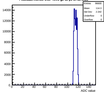
Pedestals mcm31-640F-refV0-g0-s0-p1 ch 35 test1
