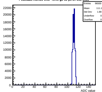
Pedestals mcm31-640F-refV0-g0-s0-p1 ch 115 test1
