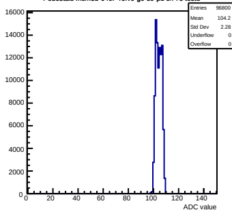
Pedestals mcm31-640F-refV0-g0-s0-p1 ch 78 test1
