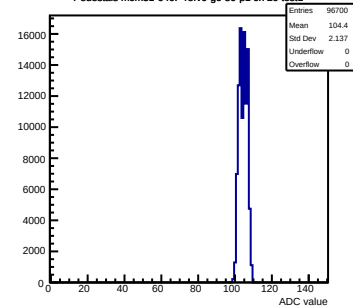
Pedestals mcm31-640F-refV0-g0-s0-p1 ch 20 test1
