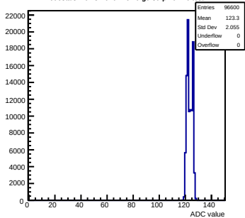
Pedestals mcm31-640F-refV0-g0-s0-p1 ch 46 test1
