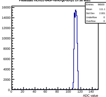
Pedestals mcm31-640F-refV0-g0-s0-p1 ch 56 test1
