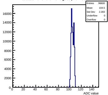
Pedestals mcm31-640F-refV0-g0-s0-p1 ch 45 test1
