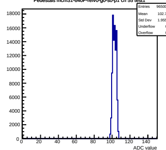
Pedestals mcm31-640F-refV0-g0-s0-p1 ch 51 test1
