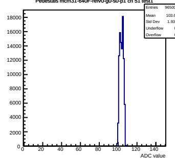
Pedestals mcm31-640F-refV0-g0-s0-p1 ch 51 test1
