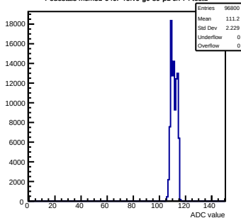
Pedestals mcm31-640F-refV0-g0-s0-p1 ch 74 test1
