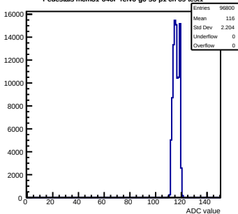
Pedestals mcm31-640F-refV0-g0-s0-p1 ch 69 test1
