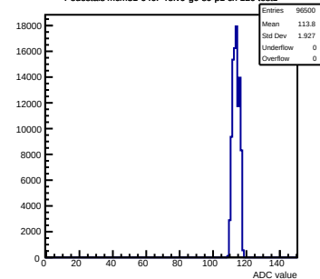
Pedestals mcm31-640F-refV0-g0-s0-p1 ch 120 test1
