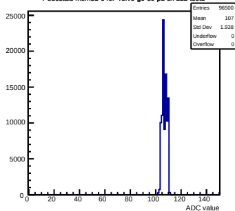
Pedestals mcm31-640F-refV0-g0-s0-p1 ch 122 test1
