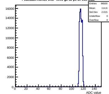
Pedestals mcm31-640F-refV0-g0-s0-p1 ch 116 test1
