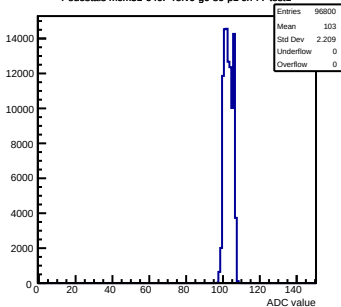
Pedestals mcm31-640F-refV0-g0-s0-p1 ch 77 test1
