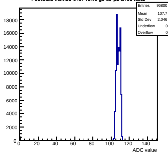
Pedestals mcm31-640F-refV0-g0-s0-p1 ch 66 test1
