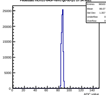
Pedestals mcm31-640F-refv1-g0-s0-p1 ch 54 test1
