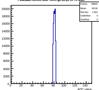
Pedestals mcm31-640F-refv1-g0-s0-p1 ch 76 test1
