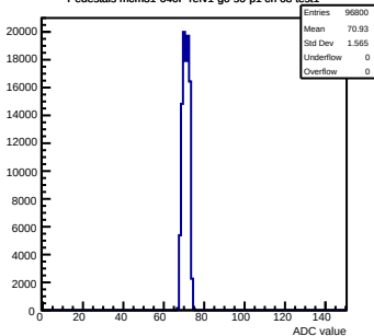
Pedestals mcm31-640F-refv1-g0-s0-p1 ch 68 test1
