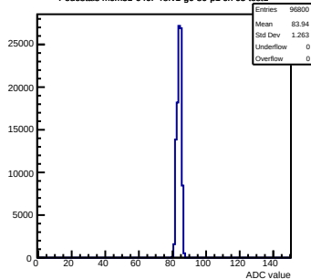
Pedestals mcm31-640F-refv1-g0-s0-p1 ch 65 test1
