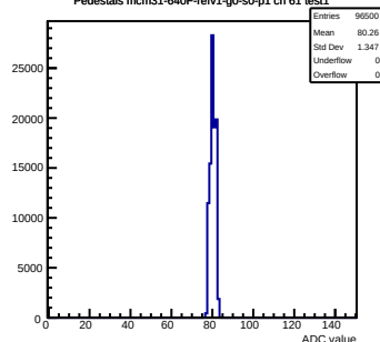
Pedestals mcm31-640F-refv1-g0-s0-p1 ch 61 test1
