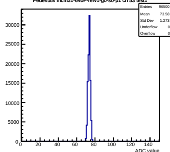
Pedestals mcm31-640F-refv1-g0-s0-p1 ch 53 test1
