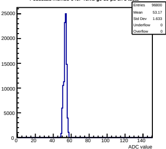
Pedestals mcm31-640F-refv2-g0-s0-p1 ch 5 test1
