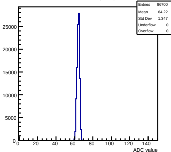
Pedestals mcm31-640F-refv2-g0-s0-p1 ch 88 test1
