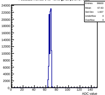
Pedestals mcm31-640F-refv2-g0-s0-p1 ch 37 test1
