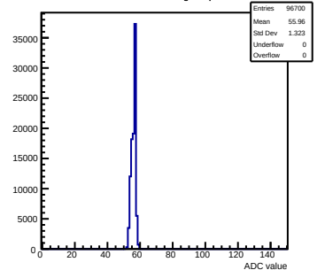
Pedestals mcm31-640F-refv2-g0-s0-p1 ch 91 test1
