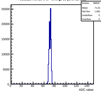
Pedestals mcm31-640F-refv2-g0-s0-p1 ch 33 test1
