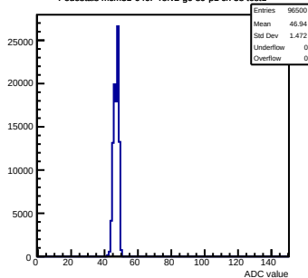
Pedestals mcm31-640F-refv2-g0-s0-p1 ch 58 test1
