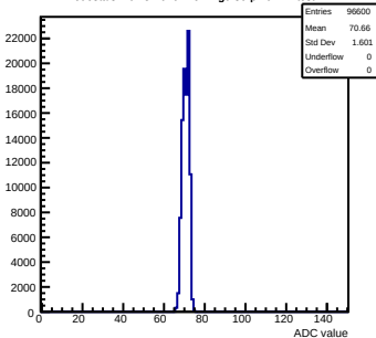
Pedestals mcm31-640F-refv2-g0-s0-p1 ch 41 test1
