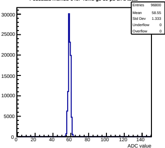
Pedestals mcm31-640F-refv2-g0-s0-p1 ch 1 test1
