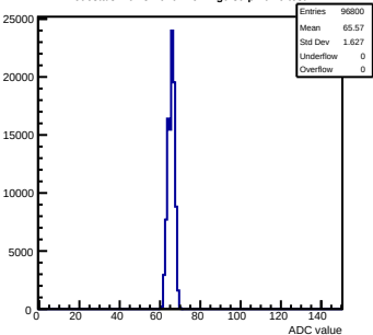
Pedestals mcm31-640F-refv2-g0-s0-p1 ch 9 test1
