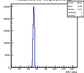
Pedestals mcm31-640F-refv2-g0-s0-p1 ch 55 test1
