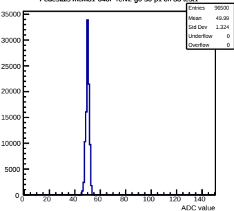
Pedestals mcm31-640F-refv2-g0-s0-p1 ch 53 test1
