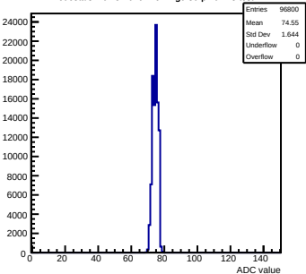
Pedestals mcm31-640F-refv2-g0-s0-p1 ch 13 test1
