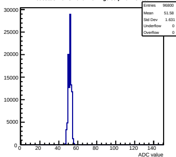
Pedestals mcm31-640F-refv2-g0-s0-p1 ch 15 test1
