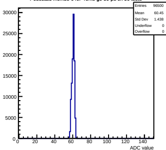
Pedestals mcm31-640F-refv2-g0-s0-p1 ch 56 test1
