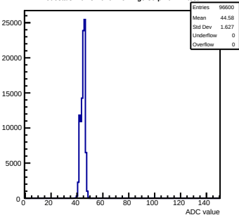
Pedestals mcm31-640F-refv2-g0-s0-p1 ch 44 test1
