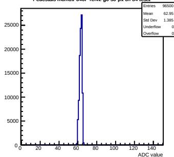
Pedestals mcm31-640F-refv2-g0-s0-p1 ch 54 test1
