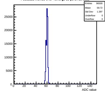
Pedestals mcm31-640F-refv2-g0-s0-p1 ch 59 test1
