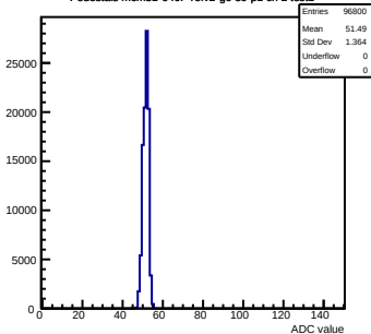
Pedestals mcm31-640F-refv2-g0-s0-p1 ch 2 test1
