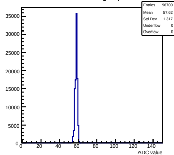
Pedestals mcm31-640F-refv2-g0-s0-p1 ch 90 test1
