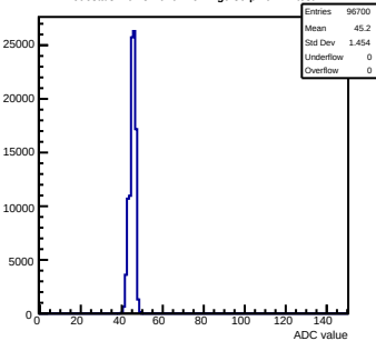
Pedestals mcm31-640F-refv2-g0-s0-p1 ch 24 test1
