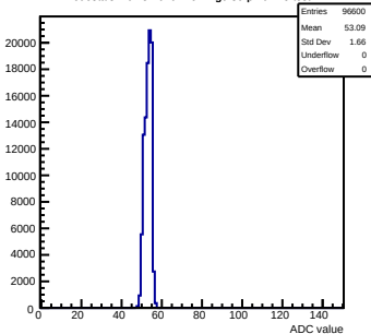
Pedestals mcm31-640F-refv2-g0-s0-p1 ch 45 test1
