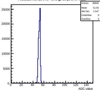
Pedestals mcm31-640F-refv2-g0-s0-p1 ch 34 test1
