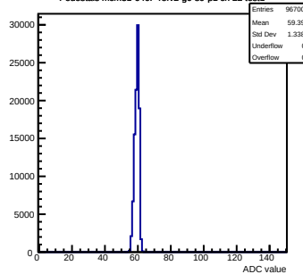
Pedestals mcm31-640F-refv2-g0-s0-p1 ch 18 test1
