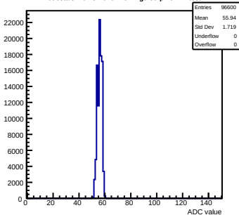
Pedestals mcm31-640F-refv2-g0-s0-p1 ch 42 test1
