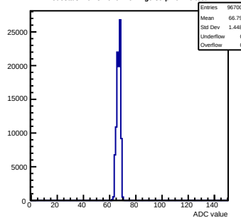
Pedestals mcm31-640F-refv2-g0-s0-p1 ch 22 test1
