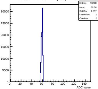
Pedestals mcm31-640F-refv2-g0-s0-p1 ch 28 test1
