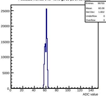
Pedestals mcm31-640F-refv2-g0-s0-p1 ch 16 test1
