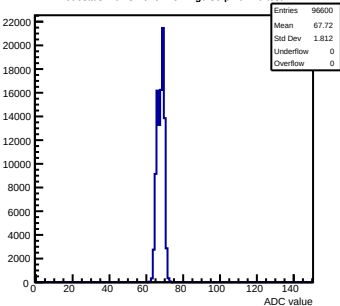
Pedestals mcm31-640F-refv2-g0-s0-p1 ch 40 test1
