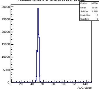
Pedestals mcm31-640F-refv2-g0-s0-p1 ch 52 test1
