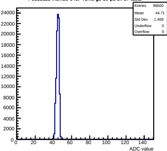
Pedestals mcm31-640F-refv2-g0-s0-p1 ch 57 test1
