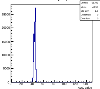
Pedestals mcm31-640F-refv2-g0-s0-p1 ch 84 test1
