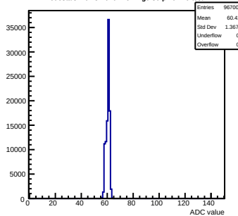
Pedestals mcm31-640F-refv2-g0-s0-p1 ch 29 test1
