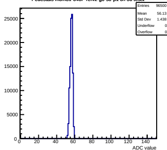
Pedestals mcm31-640F-refv2-g0-s0-p1 ch 50 test1
