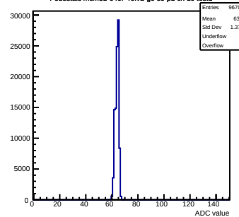
Pedestals mcm31-640F-refv2-g0-s0-p1 ch 19 test1
