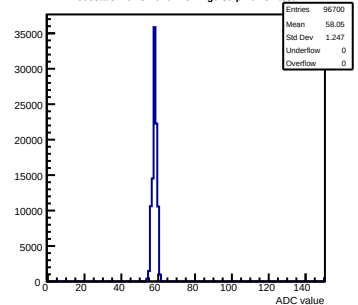
Pedestals mcm31-640F-refv2-g0-s0-p1 ch 87 test1
