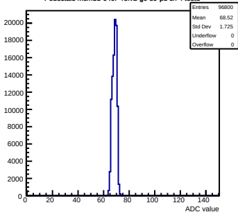
Pedestals mcm31-640F-refv2-g0-s0-p1 ch 4 test1
