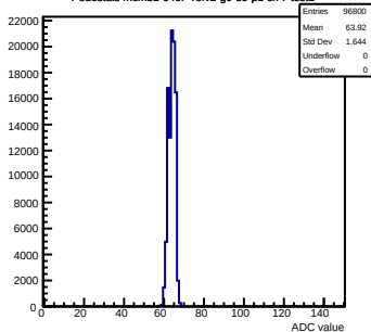
Pedestals mcm31-640F-refv2-g0-s0-p1 ch 7 test1
