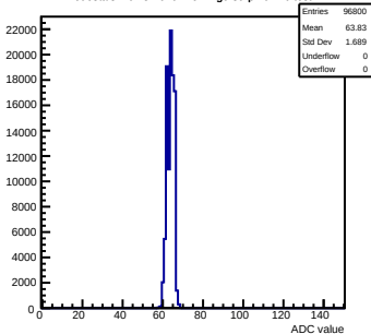
Pedestals mcm31-640F-refv2-g0-s0-p1 ch 10 test1
