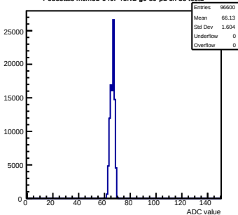
Pedestals mcm31-640F-refv2-g0-s0-p1 ch 38 test1
