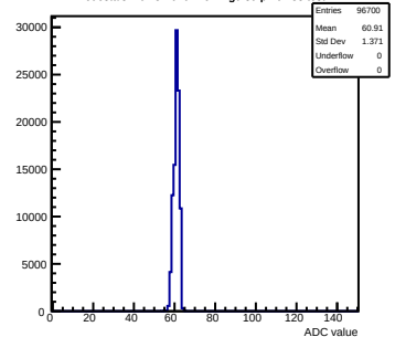
Pedestals mcm31-640F-refv2-g0-s0-p1 ch 83 test1
