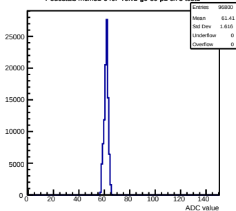
Pedestals mcm31-640F-refv2-g0-s0-p1 ch 3 test1
