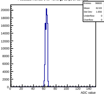
Pedestals mcm31-640F-refv2-g0-s0-p1 ch 32 test1
