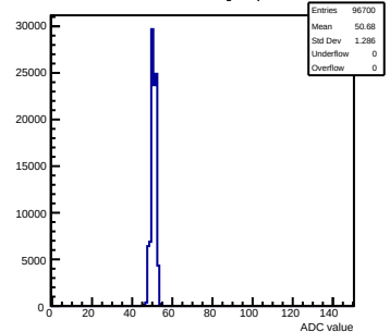
Pedestals mcm31-640F-refv2-g0-s0-p1 ch 95 test1
