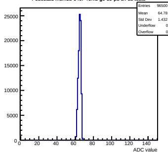
Pedestals mcm31-640F-refv2-g0-s0-p1 ch 62 test1
