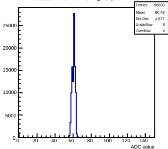
Pedestals mcm31-640F-refv2-g0-s0-p1 ch 12 test1
