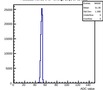
Pedestals mcm31-640F-refv2-g0-s0-p1 ch 63 test1
