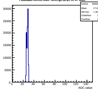
Pedestals mcm31-640F-refv3-g0-s0-p1 ch 43 test1
