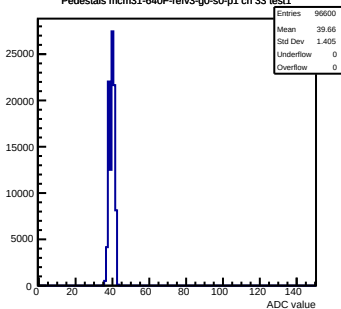
Pedestals mcm31-640F-refv3-g0-s0-p1 ch 33 test1
