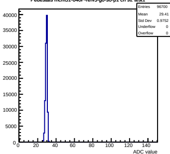
Pedestals mcm31-640F-refv3-g0-s0-p1 ch 92 test1
