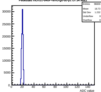
Pedestals mcm31-640F-refv3-g0-s0-p1 ch 34 test1
