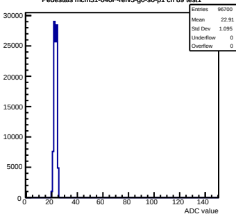
Pedestals mcm31-640F-refv3-g0-s0-p1 ch 89 test1
