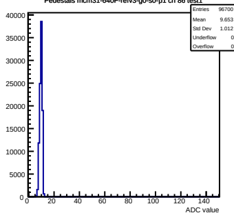
Pedestals mcm31-640F-refv3-g0-s0-p1 ch 86 test1
