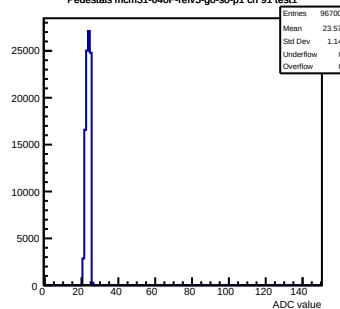
Pedestals mcm31-640F-refv3-g0-s0-p1 ch 91 test1
