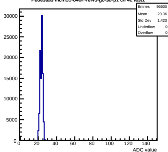
Pedestals mcm31-640F-refv3-g0-s0-p1 ch 42 test1
