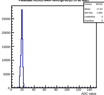
Pedestals mcm31-640F-refv3-g0-s0-p1 ch 80 test1
