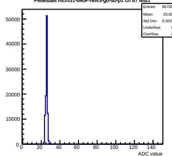
Pedestals mcm31-640F-refv3-g0-s0-p1 ch 87 test1
