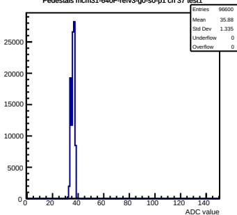
Pedestals mcm31-640F-refv3-g0-s0-p1 ch 37 test1
