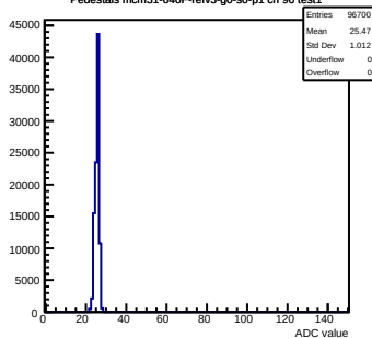
Pedestals mcm31-640F-refv3-g0-s0-p1 ch 90 test1
