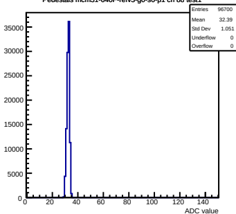
Pedestals mcm31-640F-refv3-g0-s0-p1 ch 88 test1
