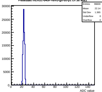
Pedestals mcm31-640F-refv3-g0-s0-p1 ch 36 test1
