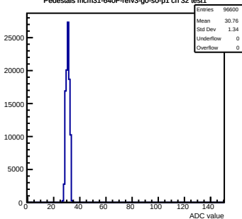
Pedestals mcm31-640F-refv3-g0-s0-p1 ch 32 test1
