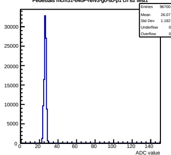
Pedestals mcm31-640F-refv3-g0-s0-p1 ch 82 test1
