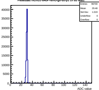
Pedestals mcm31-640F-refv3-g0-s0-p1 ch 85 test1
