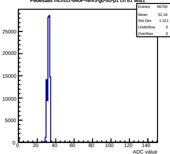
Pedestals mcm31-640F-refv3-g0-s0-p1 ch 81 test1
