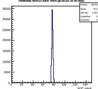
Pedestals mcm31-640F-refv5-g0-s0-p1 ch 90 test1
