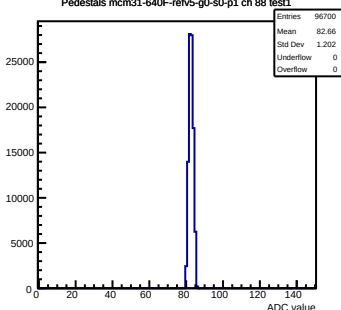
Pedestals mcm31-640F-refv5-g0-s0-p1 ch 88 test1
