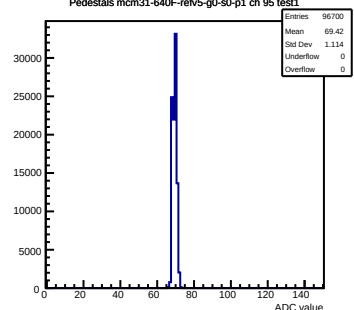
Pedestals mcm31-640F-refv5-g0-s0-p1 ch 95 test1
