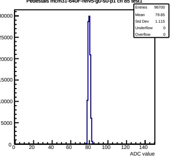
Pedestals mcm31-640F-refv5-g0-s0-p1 ch 85 test1
