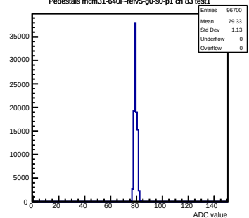
Pedestals mcm31-640F-refv5-g0-s0-p1 ch 83 test1
