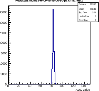
Pedestals mcm31-640F-refv5-g0-s0-p1 ch 81 test1
