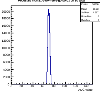
Pedestals mcm31-640F-refv5-g0-s0-p1 ch 80 test1
