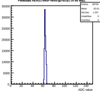
Pedestals mcm31-640F-refv5-g0-s0-p1 ch 84 test1
