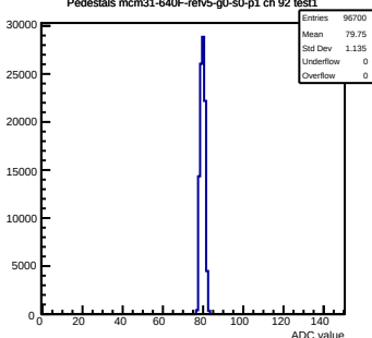
Pedestals mcm31-640F-refv5-g0-s0-p1 ch 92 test1
