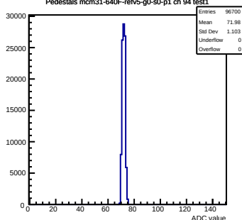
Pedestals mcm31-640F-refv5-g0-s0-p1 ch 94 test1
