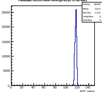
Pedestals mcm31-640F-refv6-g0-s0-p1 ch 88 test1
