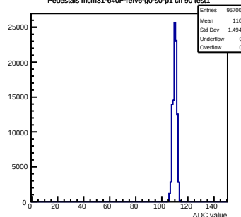
Pedestals mcm31-640F-refv6-g0-s0-p1 ch 90 test1
