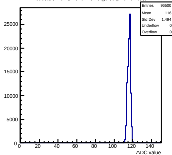
Pedestals mcm31-640F-refv6-g0-s0-p1 ch 62 test1
