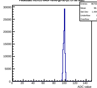
Pedestals mcm31-640F-refv6-g0-s0-p1 ch 86 test1
