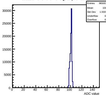
Pedestals mcm31-640F-refv6-g0-s0-p1 ch 58 test1
