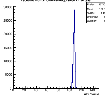
Pedestals mcm31-640F-refv6-g0-s0-p1 ch 94 test1
