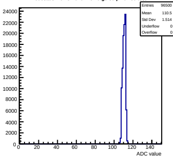
Pedestals mcm31-640F-refv6-g0-s0-p1 ch 55 test1
