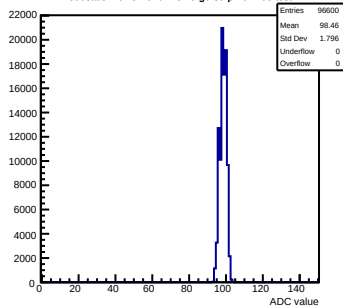
Pedestals mcm31-640F-refv6-g0-s0-p1 ch 101 test1
