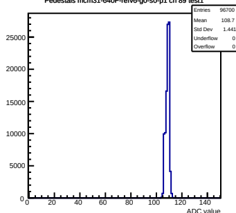
Pedestals mcm31-640F-refv6-g0-s0-p1 ch 89 test1
