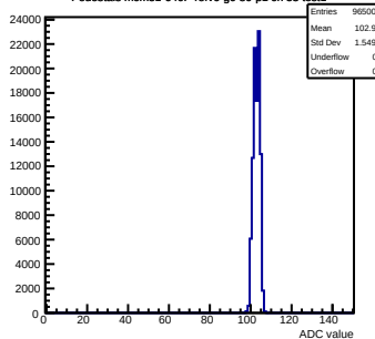
Pedestals mcm31-640F-refv6-g0-s0-p1 ch 49 test1
