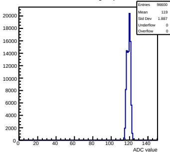
Pedestals mcm31-640F-refv6-g0-s0-p1 ch 40 test1
