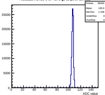
Pedestals mcm31-640F-refv6-g0-s0-p1 ch 51 test1
