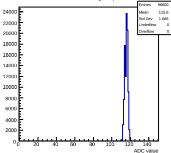
Pedestals mcm31-640F-refv6-g0-s0-p1 ch 104 test1
