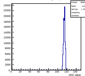
Pedestals mcm31-640F-refv6-g0-s0-p1 ch 43 test1
