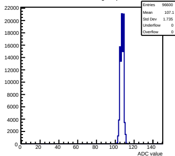
Pedestals mcm31-640F-refv6-g0-s0-p1 ch 109 test1
