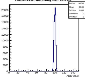
Pedestals mcm31-640F-refv6-g0-s0-p1 ch 84 test1
