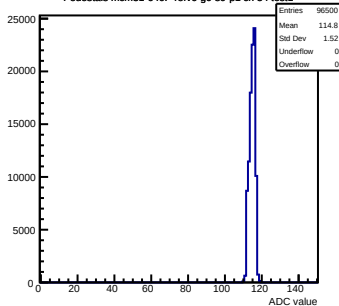
Pedestals mcm31-640F-refv6-g0-s0-p1 ch 50 test1
