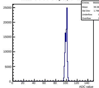
Pedestals mcm31-640F-refv6-g0-s0-p1 ch 99 test1
