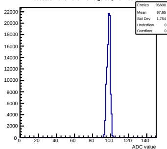
Pedestals mcm31-640F-refv6-g0-s0-p1 ch 102 test1
