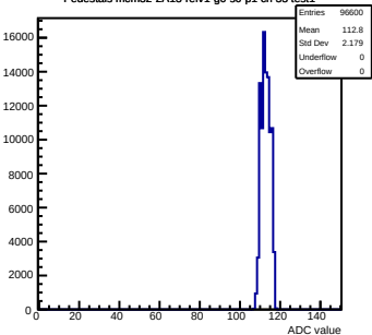
Pedestals mcm32-2A13-refv1-g0-s0-p1 ch 33 test1
