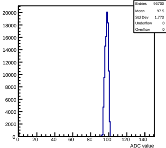
Pedestals mcm32-2A13-refv1-q0-s0-p1 ch 31 test1
