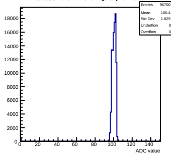
Pedestals mcm32-2A13-refv1-q0-s0-p1 ch 18 test1
