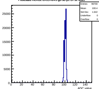
Pedestals mcm32-2A13-refv1-q0-s0-p1 ch 92 test1
