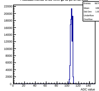
Pedestals mcm32-2A13-refv1-q0-s0-p1 ch 83 test1
