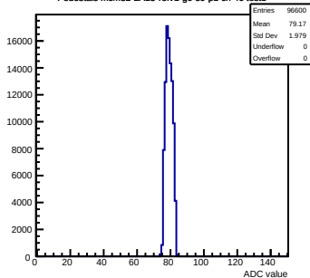
Pedestals mcm32-2A13-refv1-g0-s0-p1 ch 46 test1
