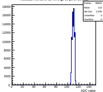
Pedestals mcm32-2A13-refv1-g0-s0-p1 ch 38 test1
