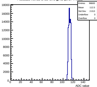
Pedestals mcm32-2A13-refv1-g0-s0-p1 ch 44 test1
