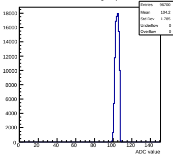
Pedestals mcm32-2A13-refv1-q0-s0-p1 ch 24 test1
