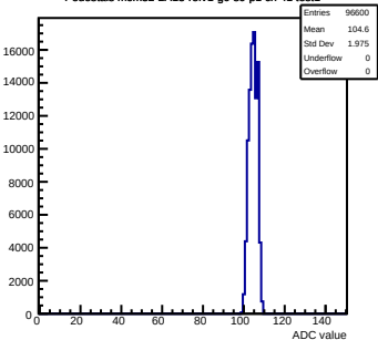
Pedestals mcm32-2A13-refv1-g0-s0-p1 ch 41 test1
