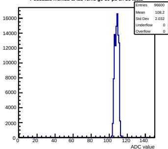
Pedestals mcm32-2A13-refv1-g0-s0-p1 ch 36 test1
