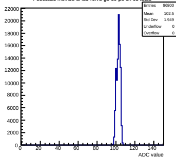
Pedestals mcm32-2A13-refv1-q0-s0-p1 ch 65 test1
