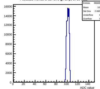
Pedestals mcm32-2A13-refv1-g0-s0-p1 ch 39 test1
