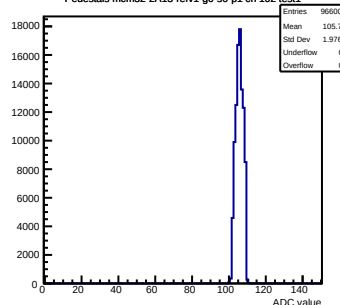
Pedestals mcm32-2A13-refv1-g0-s0-p1 ch 102 test1
