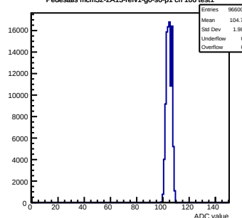
Pedestals mcm32-2A13-refv1-g0-s0-p1 ch 106 test1
