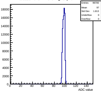
Pedestals mcm32-2A13-refv1-q0-s0-p1 ch 17 test1
