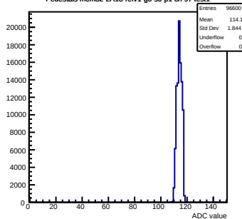
Pedestals mcm32-2A13-refv1-g0-s0-p1 ch 97 test1
