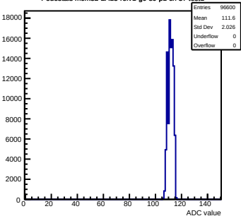
Pedestals mcm32-2A13-refv1-g0-s0-p1 ch 37 test1
