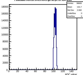
Pedestals mcm32-2A13-refv1-g0-s0-p1 ch 104 test1
