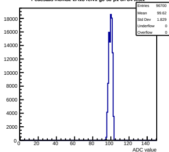
Pedestals mcm32-2A13-refv1-q0-s0-p1 ch 80 test1
