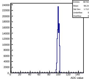
Pedestals mcm32-2A13-refv1-q0-s0-p1 ch 22 test1
