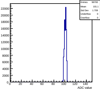
Pedestals mcm32-2A13-refv1-q0-s0-p1 ch 29 test1
