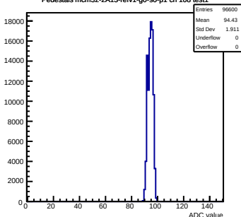
Pedestals mcm32-2A13-refv1-g0-s0-p1 ch 108 test1
