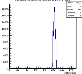
Pedestals mcm32-2A13-refv1-g0-s0-p1 ch 34 test1
