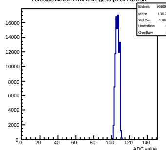
Pedestals mcm32-2A13-refv1-g0-s0-p1 ch 110 test1
