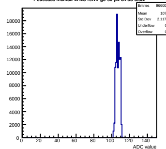
Pedestals mcm32-2A13-refv1-g0-s0-p1 ch 35 test1
