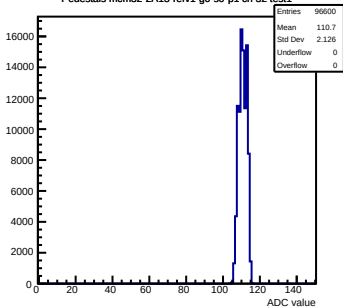
Pedestals mcm32-2A13-refv1-g0-s0-p1 ch 32 test1
