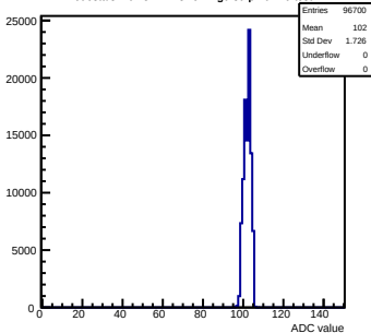
Pedestals mcm32-2A13-refv1-q0-s0-p1 ch 19 test1
