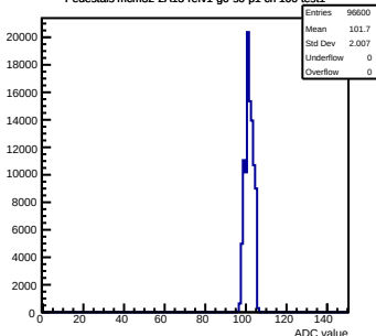
Pedestals mcm32-2A13-refv1-g0-s0-p1 ch 100 test1
