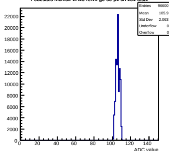
Pedestals mcm32-2A13-refv1-g0-s0-p1 ch 101 test1
