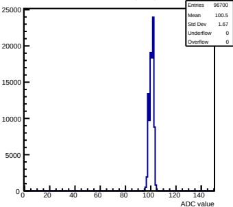
Pedestals mcm32-2A13-refv1-q0-s0-p1 ch 21 test1
