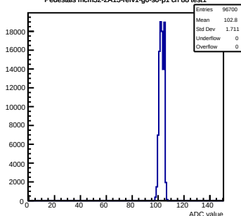
Pedestals mcm32-2A13-refv1-q0-s0-p1 ch 84 test1
