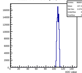
Pedestals mcm32-2A13-refv1-q0-s0-p1 ch 78 test1
