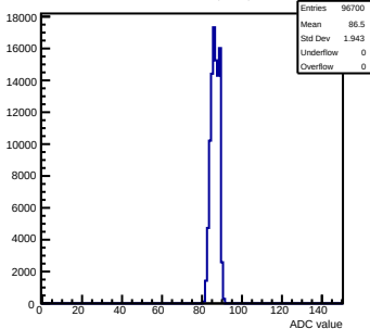
Pedestals mcm32-2A13-refv1-q0-s0-p1 ch 20 test1
