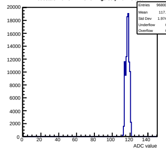
Pedestals mcm32-2A13-refv1-q0-s0-p1 ch 75 test1
