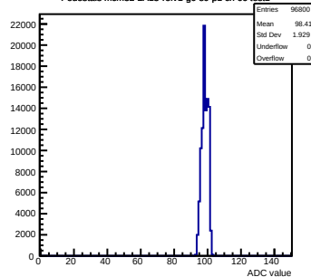
Pedestals mcm32-2A13-refv1-q0-s0-p1 ch 66 test1
