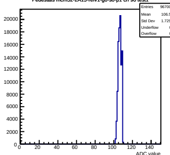
Pedestals mcm32-2A13-refv1-q0-s0-p1 ch 86 test1
