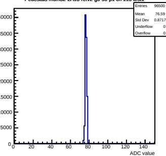
Pedestals mcm32-2A13-refv2-g0-s0-p1 ch 113 test1
