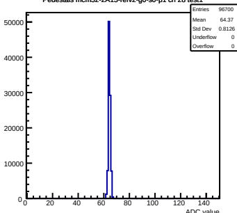
Pedestals mcm32-2A13-refv2-g0-s0-p1 ch 28 test1
