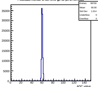
Pedestals mcm32-2A13-refv2-g0-s0-p1 ch 16 test1
