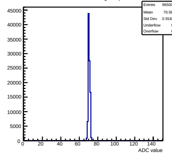
Pedestals mcm32-2A13-refv4-g0-s0-p1 ch 59 test1
