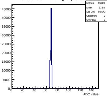
Pedestals mcm32-2A13-refv4-g0-s0-p1 ch 52 test1
