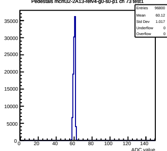
Pedestals mcm32-2A13-refv4-g0-s0-p1 ch 73 test1
