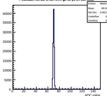
Pedestals mcm32-2A13-refv4-g0-s0-p1 ch 102 test1
