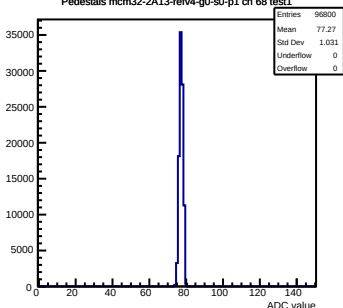
Pedestals mcm32-2A13-refv4-g0-s0-p1 ch 68 test1
