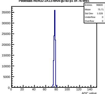
Pedestals mcm32-2A13-refv4-g0-s0-p1 ch 76 test1
