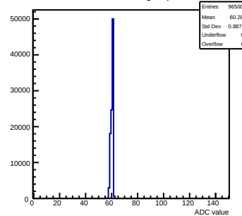
Pedestals mcm32-2A13-refv4-g0-s0-p1 ch 63 test1
