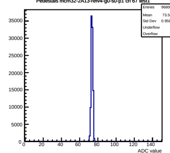
Pedestals mcm32-2A13-refv4-g0-s0-p1 ch 67 test1
