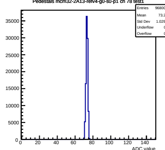
Pedestals mcm32-2A13-refv4-g0-s0-p1 ch 78 test1
