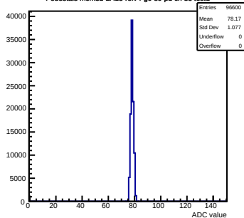
Pedestals mcm32-2A13-refv4-g0-s0-p1 ch 33 test1
