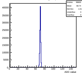
Pedestals mcm32-2A13-refv4-g0-s0-p1 ch 41 test1
