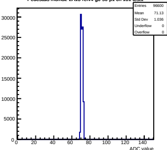
Pedestals mcm32-2A13-refv4-g0-s0-p1 ch 101 test1
