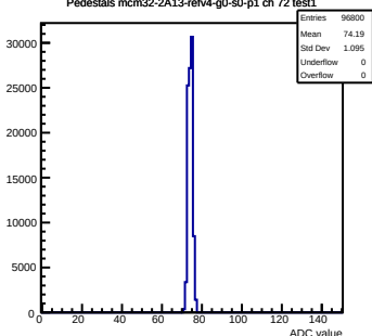
Pedestals mcm32-2A13-refv4-g0-s0-p1 ch 72 test1
