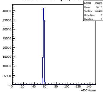
Pedestals mcm32-2A13-refv4-g0-s0-p1 ch 53 test1
