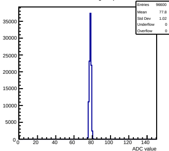
Pedestals mcm32-2A13-refv4-g0-s0-p1 ch 44 test1
