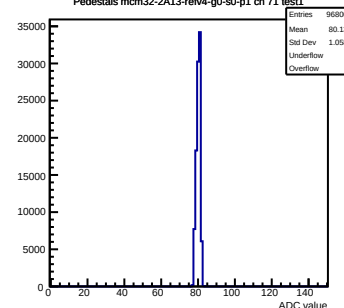
Pedestals mcm32-2A13-refv4-g0-s0-p1 ch 71 test1
