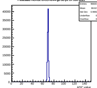
Pedestals mcm32-2A13-refv4-g0-s0-p1 ch 106 test1
