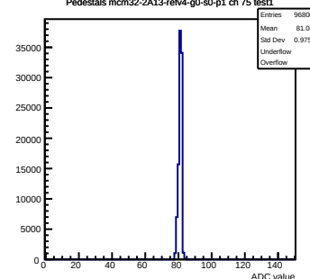
Pedestals mcm32-2A13-refv4-g0-s0-p1 ch 75 test1
