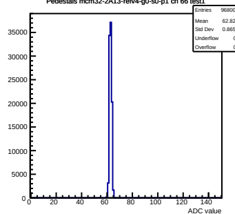
Pedestals mcm32-2A13-refv4-g0-s0-p1 ch 66 test1
