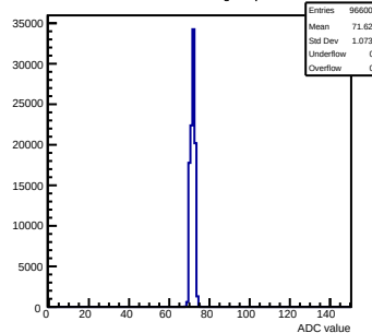
Pedestals mcm32-2A13-refv4-g0-s0-p1 ch 47 test1
