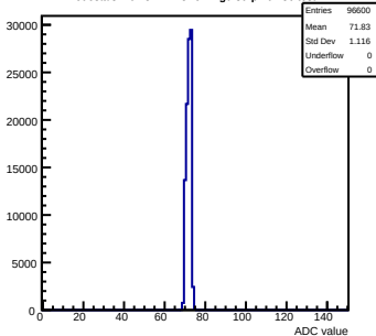
Pedestals mcm32-2A13-refv4-g0-s0-p1 ch 36 test1
