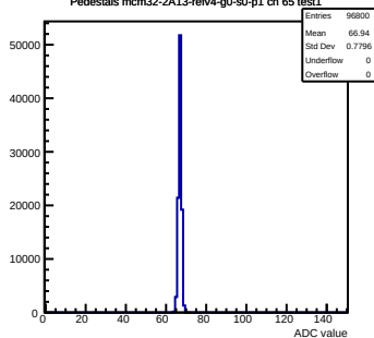
Pedestals mcm32-2A13-refv4-g0-s0-p1 ch 65 test1
