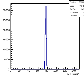
Pedestals mcm32-2A13-refv4-g0-s0-p1 ch 43 test1
