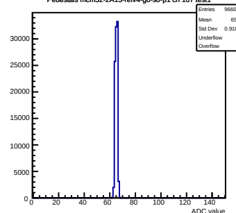
Pedestals mcm32-2A13-refv4-g0-s0-p1 ch 107 test1
