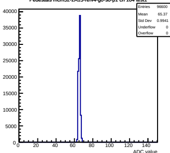
Pedestals mcm32-2A13-refv4-g0-s0-p1 ch 104 test1
