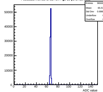
Pedestals mcm32-2A13-refv4-g0-s0-p1 ch 51 test1
