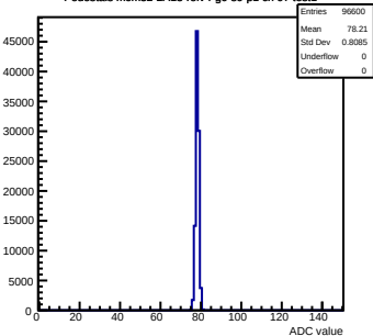
Pedestals mcm32-2A13-refv4-g0-s0-p1 ch 97 test1
