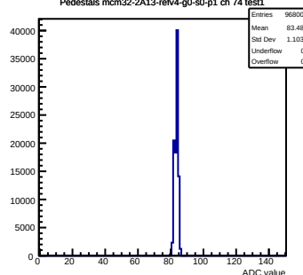
Pedestals mcm32-2A13-refv4-g0-s0-p1 ch 74 test1
