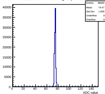
Pedestals mcm32-2A13-refv4-g0-s0-p1 ch 38 test1
