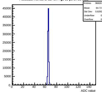
Pedestals mcm32-2A13-refv4-g0-s0-p1 ch 98 test1
