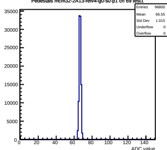
Pedestals mcm32-2A13-refv4-g0-s0-p1 ch 69 test1
