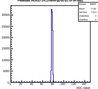
Pedestals mcm32-2A13-refv4-g0-s0-p1 ch 64 test1
