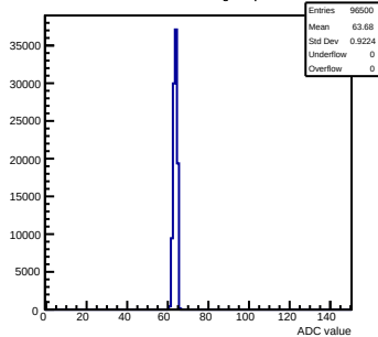
Pedestals mcm32-2A13-refv4-g0-s0-p1 ch 61 test1
