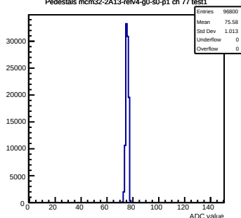
Pedestals mcm32-2A13-refv4-g0-s0-p1 ch 77 test1
