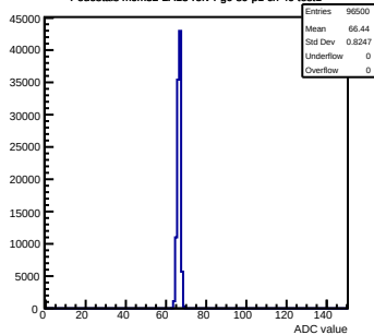
Pedestals mcm32-2A13-refv4-g0-s0-p1 ch 49 test1
