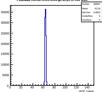
Pedestals mcm32-2A13-refv4-g0-s0-p1 ch 109 test1
