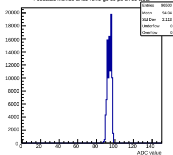
Pedestals mcm32-2A13-refv5-g0-s0-p1 ch 55 test1
