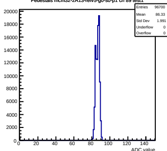
Pedestals mcm32-2A13-refV5-g0-s0-p1 ch 89 test1
