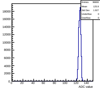
Pedestals mcm40-7411- \text{rev0-g0-s0-p1} ch 6 test1
