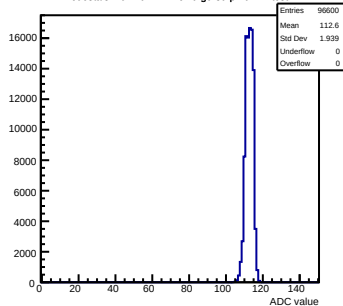
Pedestals mcm40-7411-refV0-g0-s0-p1 ch 41 test1
