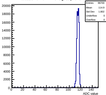
Pedestals mcm40-7411-refV0-g0-s0-p1 ch 84 test1
