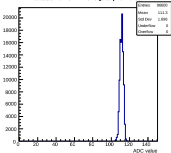
Pedestals mcm40-7411-refV0-g0-s0-p1 ch 40 test1
