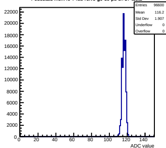
Pedestals mcm40-7411-refV0-g0-s0-p1 ch 37 test1
