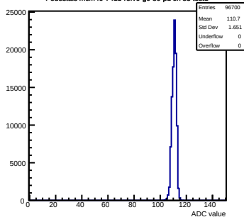
Pedestals mcm40-7411-refV0-g0-s0-p1 ch 83 test1
