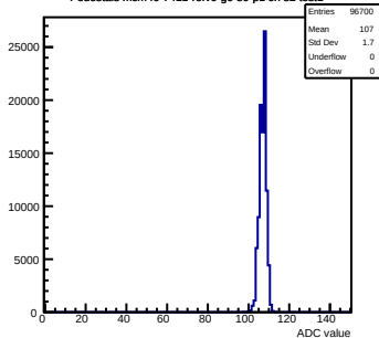
Pedestals mcm40-7411-refV0-g0-s0-p1 ch 82 test1
