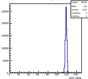
Pedestals mcm40-7411-refV0-g0-s0-p1 ch 88 test1
