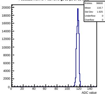
Pedestals mcm40-7411-refV0-g0-s0-p1 ch 36 test1
