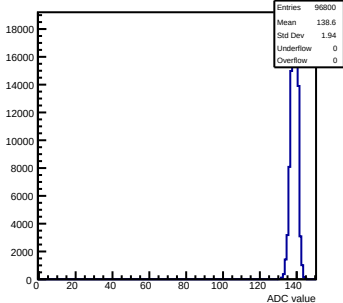
Pedestals mcm40-7411- \text{rev0-g0-s0-p1} ch 8 test1
