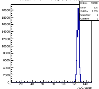
Pedestals mcm40-7411-refV0-g0-s0-p1 ch 80 test1
