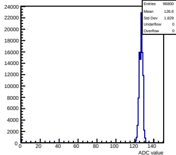
Pedestals mcm40-7411- \text{rev0-g0-s0-p1} ch 15 test1
