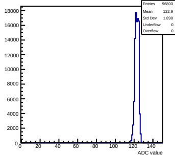
Pedestals mcm40-7411- \text{rev0-g0-s0-p1} ch 9 test1
