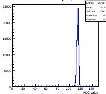
Pedestals mcm40-7411-refV0-g0-s0-p1 ch 85 test1
