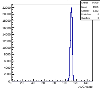
Pedestals mcm40-7411-refV0-g0-s0-p1 ch 95 test1
