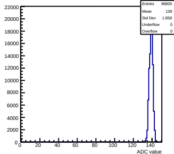
Pedestals mcm40-7411- \text{rev0-g0-s0-p1} ch 5 test1
