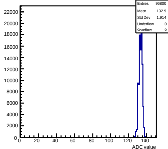
Pedestals mcm40-7411- \text{rev0-g0-s0-p1} ch 10 test1
