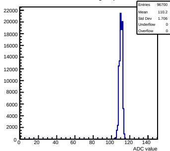
Pedestals mcm40-7411-refV0-g0-s0-p1 ch 94 test1
