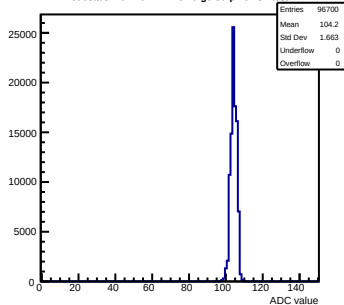
Pedestals mcm40-7411-refV0-g0-s0-p1 ch 87 test1
