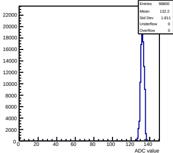
Pedestals mcm40-7411- \text{rev0-g0-s0-p1} ch 12 test1
