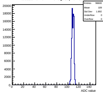
Pedestals mcm40-7411-refV0-g0-s0-p1 ch 45 test1
