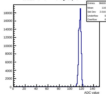
Pedestals mcm40-7411-refV0-g0-s0-p1 ch 42 test1
