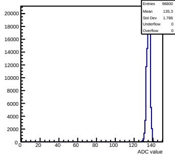
Pedestals mcm40-7411- \text{rev0-g0-s0-p1} ch 13 test1
