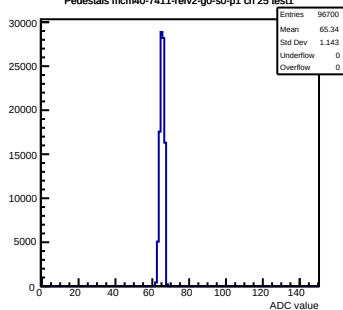
Pedestals mcm40-7411-refv2-g0-s0-p1 ch 25 test1
