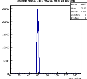
Pedestals mcm40-7411-refv2-g0-s0-p1 ch 105 test1
