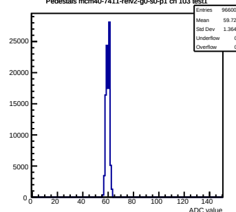
Pedestals mcm40-7411-refv2-g0-s0-p1 ch 103 test1
