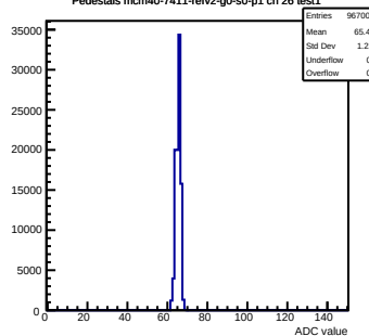
Pedestals mcm40-7411-refv2-g0-s0-p1 ch 26 test1
