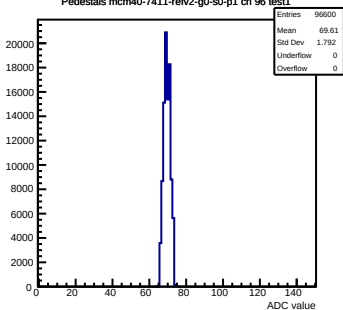
Pedestals mcm40-7411-refv2-g0-s0-p1 ch 96 test1
