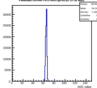
Pedestals mcm40-7411-refv2-g0-s0-p1 ch 30 test1
