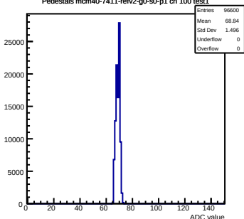
Pedestals mcm40-7411-refv2-g0-s0-p1 ch 100 test1
