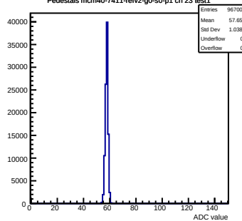
Pedestals mcm40-7411-refv2-g0-s0-p1 ch 23 test1
