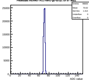
Pedestals mcm40-7411-refv2-g0-s0-p1 ch 97 test1
