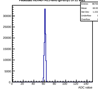
Pedestals mcm40-7411-refv2-g0-s0-p1 ch 22 test1
