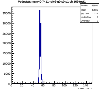
Pedestals mcm40-7411-refv2-g0-s0-p1 ch 109 test1
