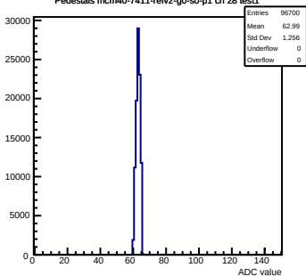
Pedestals mcm40-7411-refv2-g0-s0-p1 ch 28 test1
