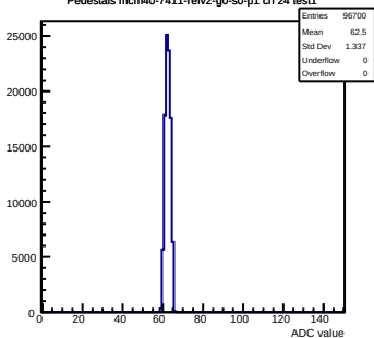
Pedestals mcm40-7411-refv2-g0-s0-p1 ch 24 test1
