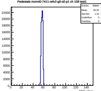
Pedestals mcm40-7411-refv2-g0-s0-p1 ch 108 test1
