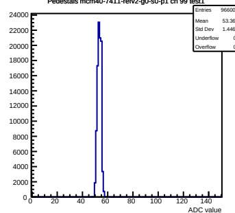
Pedestals mcm40-7411-refv2-g0-s0-p1 ch 99 test1
