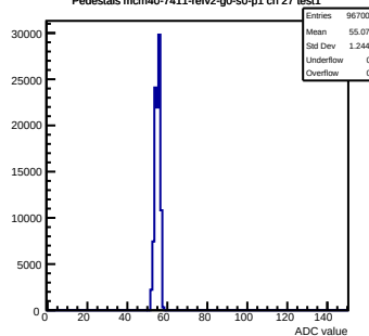
Pedestals mcm40-7411-refv2-g0-s0-p1 ch 27 test1
