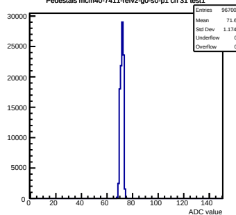
Pedestals mcm40-7411-refv2-g0-s0-p1 ch 31 test1
