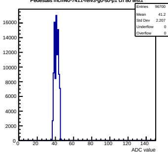
Pedestals mcm40-7411-refv3-g0-s0-p1 ch 80 test1
