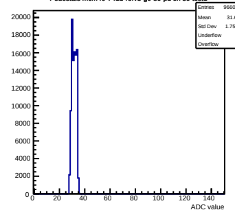
Pedestals mcm40-7411-refv3-g0-s0-p1 ch 39 test1
