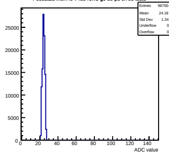
Pedestals mcm40-7411-refv3-g0-s0-p1 ch 91 test1
