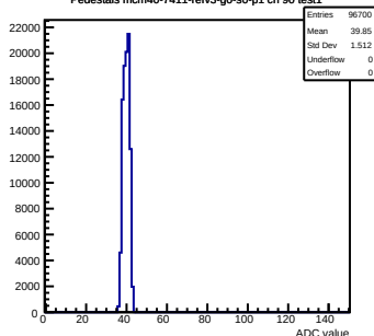
Pedestals mcm40-7411-refv3-g0-s0-p1 ch 90 test1
