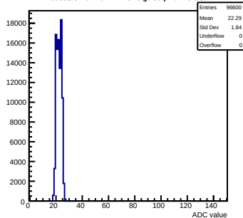
Pedestals mcm40-7411-refv3-g0-s0-p1 ch 45 test1
