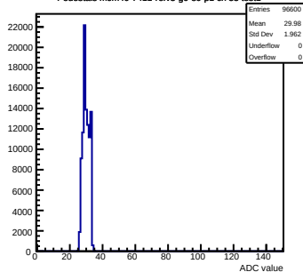
Pedestals mcm40-7411-refv3-g0-s0-p1 ch 33 test1
