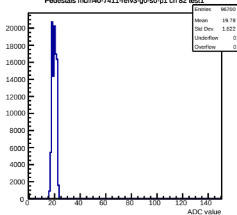
Pedestals mcm40-7411-refv3-g0-s0-p1 ch 82 test1
