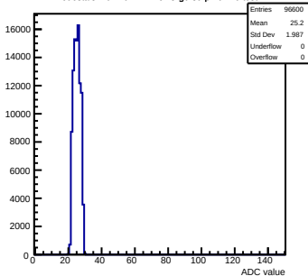
Pedestals mcm40-7411-refv3-g0-s0-p1 ch 40 test1
