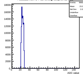
Pedestals mcm40-7411-refv3-g0-s0-p1 ch 35 test1
