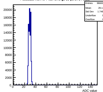
Pedestals mcm40-7411-refv3-g0-s0-p1 ch 34 test1
