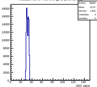
Pedestals mcm40-7411-refv3-g0-s0-p1 ch 36 test1
