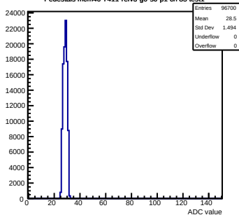
Pedestals mcm40-7411-refv3-g0-s0-p1 ch 85 test1
