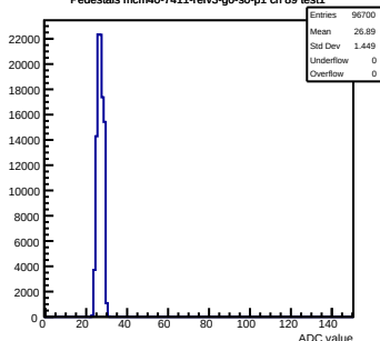
Pedestals mcm40-7411-refv3-g0-s0-p1 ch 89 test1
