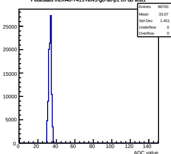
Pedestals mcm40-7411-refv3-g0-s0-p1 ch 88 test1
