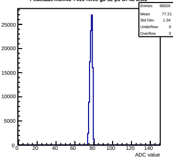
Pedestals mcm40-7411-refV5-g0-s0-p1 ch 48 test1
