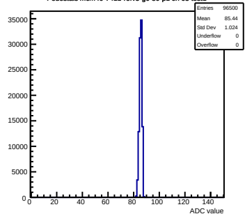
Pedestals mcm40-7411-refV5-g0-s0-p1 ch 63 test1
