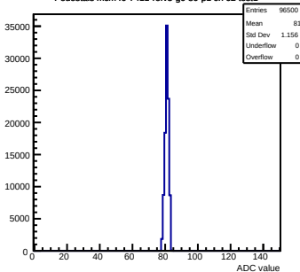
Pedestals mcm40-7411-refV5-g0-s0-p1 ch 62 test1
