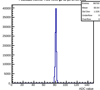
Pedestals mcm40-7411-refV5-g0-s0-p1 ch 22 test1
