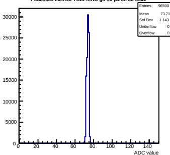
Pedestals mcm40-7411-refV5-g0-s0-p1 ch 50 test1
