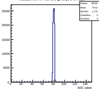
Pedestals mcm40-7411-refV5-g0-s0-p1 ch 24 test1
