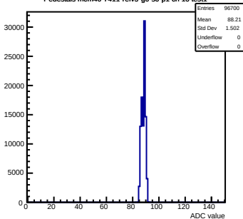
Pedestals mcm40-7411-refV5-g0-s0-p1 ch 16 test1
