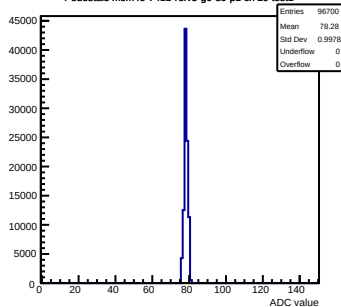
Pedestals mcm40-7411-refV5-g0-s0-p1 ch 29 test1
