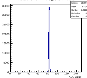
Pedestals mcm40-7411-refV5-g0-s0-p1 ch 25 test1
