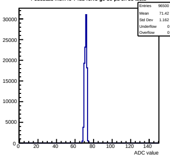
Pedestals mcm40-7411-refV5-g0-s0-p1 ch 58 test1
