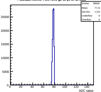
Pedestals mcm40-7411-refV5-g0-s0-p1 ch 52 test1
