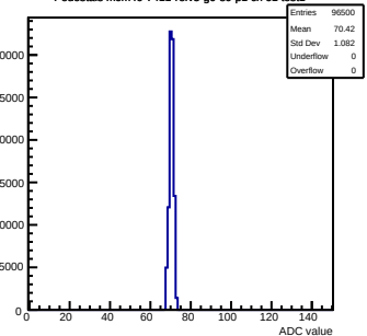
Pedestals mcm40-7411-refV5-g0-s0-p1 ch 61 test1
