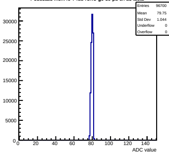
Pedestals mcm40-7411-refV5-g0-s0-p1 ch 28 test1
