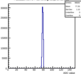
Pedestals mcm40-7411-refV5-g0-s0-p1 ch 60 test1
