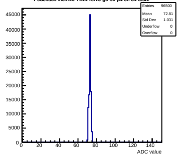
Pedestals mcm40-7411-refV5-g0-s0-p1 ch 51 test1
