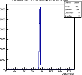
Pedestals mcm40-7411-refV5-g0-s0-p1 ch 49 test1
