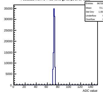
Pedestals mcm40-7411-refV5-g0-s0-p1 ch 27 test1
