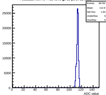
Pedestals mcm40-7411- rfv6-g0-s0-p1 ch 23 test1
