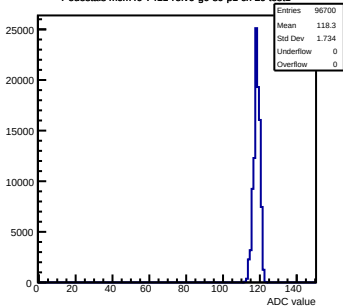
Pedestals mcm40-7411- rfv6-g0-s0-p1 ch 20 test1
