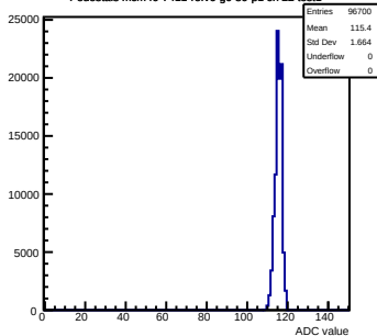
Pedestals mcm40-7411- rfv6-g0-s0-p1 ch 22 test1
