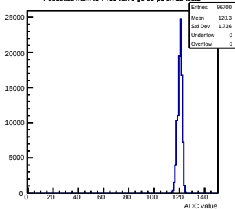
Pedestals mcm40-7411- rfv6-g0-s0-p1 ch 18 test1
