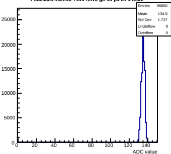
Pedestals mcm40-7411-rlv6-g0-s0-p1 ch 1 test1
