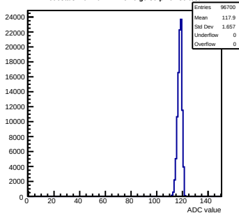
Pedestals mcm40-7411- rfv6-g0-s0-p1 ch 30 test1
