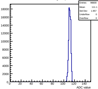
Pedestals mcm40-7411- rev6-g0-s0-p1 ch 44 test1
