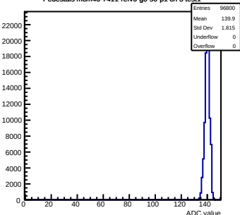
Pedestals mcm40-7411-rlv6-g0-s0-p1 ch 5 test1
