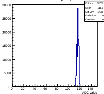
Pedestals mcm40-7411- rfv6-g0-s0-p1 ch 29 test1
