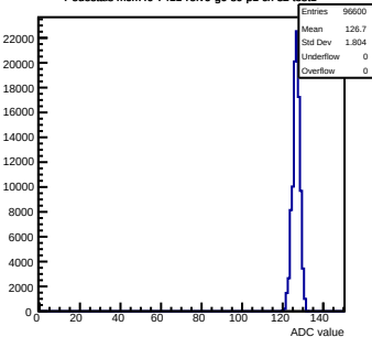
Pedestals mcm40-7411- rev6-g0-s0-p1 ch 33 test1
