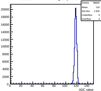
Pedestals mcm40-7411- rev6-g0-s0-p1 ch 36 test1
