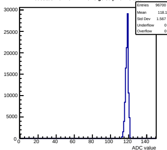
Pedestals mcm40-7411- rfv6-g0-s0-p1 ch 25 test1
