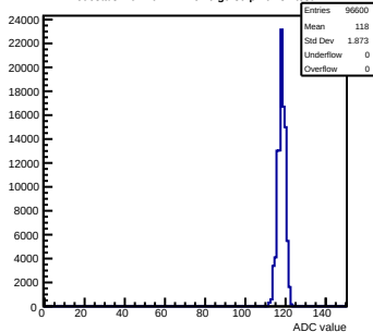
Pedestals mcm40-7411- rev6-g0-s0-p1 ch 37 test1
