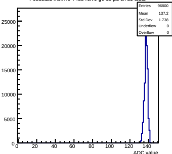
Pedestals mcm40-7411-rlv6-g0-s0-p1 ch 13 test1
