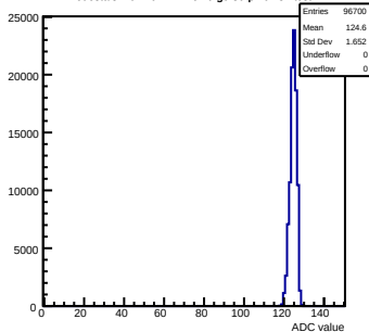
Pedestals mcm40-7411- rfv6-g0-s0-p1 ch 31 test1
