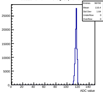
Pedestals mcm40-7411- rfv6-g0-s0-p1 ch 28 test1
