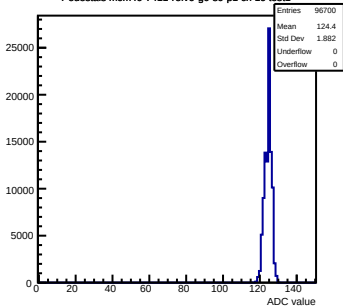
Pedestals mcm40-7411- rfv6-g0-s0-p1 ch 16 test1
