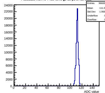
Pedestals mcm40-7411- rev6-g0-s0-p1 ch 35 test1
