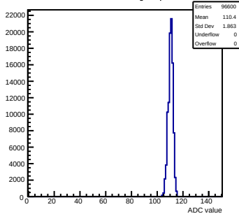
Pedestals mcm40-7411- rev6-g0-s0-p1 ch 45 test1
