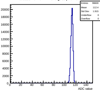
Pedestals mcm40-7411- rev6-g0-s0-p1 ch 40 test1
