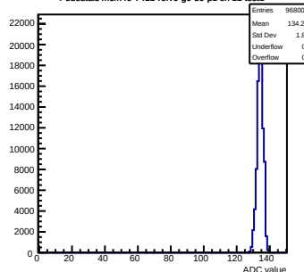
Pedestals mcm40-7411-rlv6-g0-s0-p1 ch 11 test1
