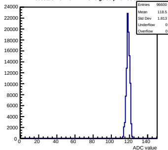
Pedestals mcm40-7411- rev6-g0-s0-p1 ch 38 test1
