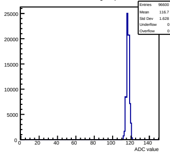
Pedestals mcm40-7411- rev6-g0-s0-p1 ch 46 test1
