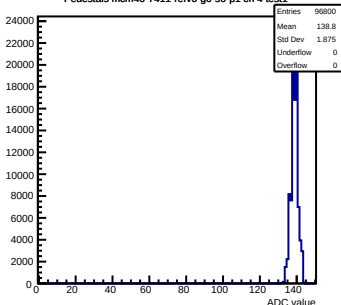
Pedestals mcm40-7411-rlv6-g0-s0-p1 ch 4 test1
