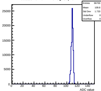
Pedestals mcm40-7411- rfv6-g0-s0-p1 ch 27 test1
