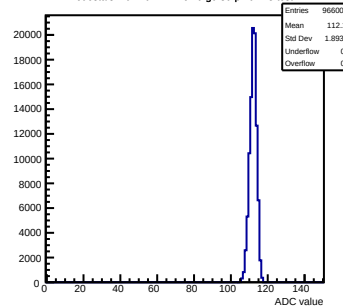
Pedestals mcm40-7411- rev6-g0-s0-p1 ch 43 test1
