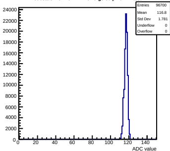
Pedestals mcm40-7411- rfv6-g0-s0-p1 ch 24 test1
