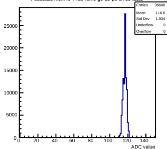
Pedestals mcm40-7411- rev6-g0-s0-p1 ch 33 test1
