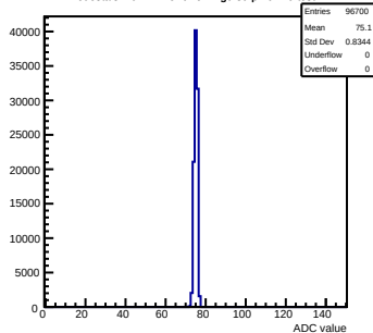
Pedestals mcm41-2C10-refv2-g0-s0-p1 ch 29 test1
