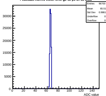
Pedestals mcm41-2C10-refv2-g0-s0-p1 ch 18 test1
