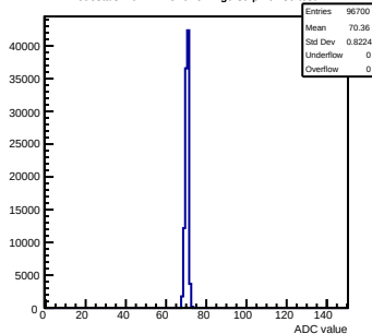
Pedestals mcm41-2C10-refv2-g0-s0-p1 ch 30 test1
