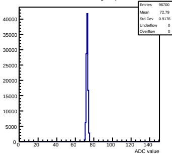
Pedestals mcm41-2C10-refv2-g0-s0-p1 ch 84 test1
