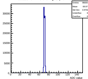
Pedestals mcm41-2C10-refV2-g0-s0-p1 ch 110 test1
