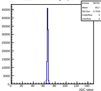
Pedestals mcm41-2C10-refv2-g0-s0-p1 ch 28 test1
