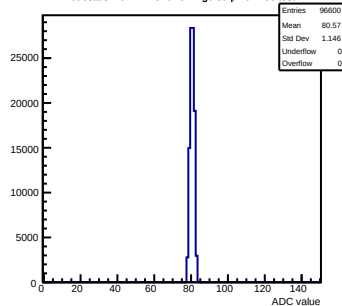
Pedestals mcm41-2C10-refV2-g0-s0-p1 ch 106 test1
