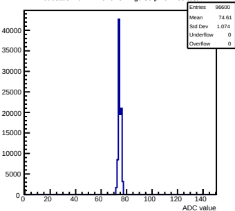
Pedestals mcm41-2C10-refV2-g0-s0-p1 ch 108 test1
