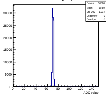
Pedestals mcm41-2C10-refV2-g0-s0-p1 ch 105 test1
