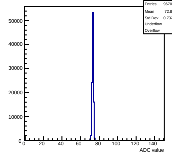
Pedestals mcm41-2C10-refv2-g0-s0-p1 ch 95 test1
