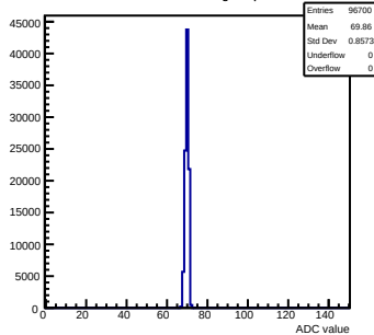
Pedestals mcm41-2C10-refv2-g0-s0-p1 ch 85 test1
