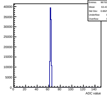
Pedestals mcm41-2C10-refv2-g0-s0-p1 ch 90 test1
