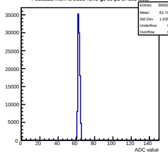
Pedestals mcm41-2C10-refV2-g0-s0-p1 ch 103 test1
