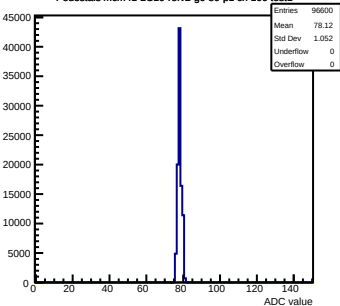
Pedestals mcm41-2C10-refV2-g0-s0-p1 ch 100 test1
