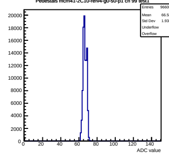
Pedestals mcm41-2C10-refV4-g0-s0-p1 ch 99 test1
