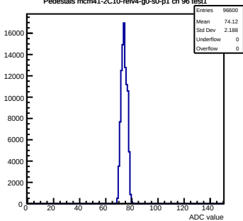
Pedestals mcm41-2C10-refV4-g0-s0-p1 ch 96 test1
