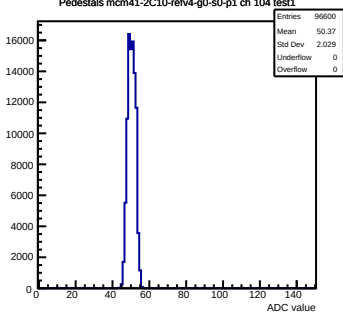
Pedestals mcm41-2C10-refV4-g0-s0-p1 ch 104 test1
