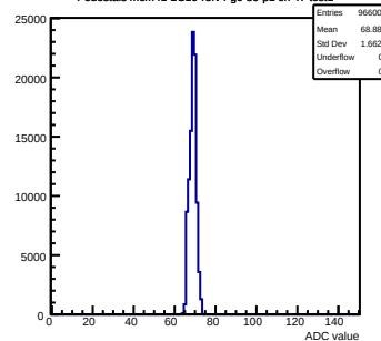
Pedestals mcm41-2C10-refv4-g0-s0-p1 ch 47 test1
