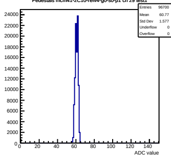
Pedestals mcm41-2C10-refV4-g0-s0-p1 ch 29 test1
