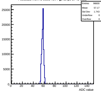
Pedestals mcm41-2C10-refv4-g0-s0-p1 ch 45 test1
