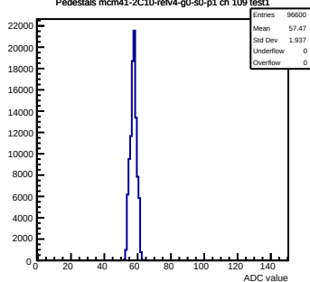
Pedestals mcm41-2C10-refV4-g0-s0-p1 ch 109 test1
