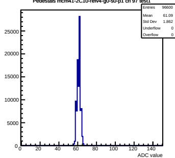
Pedestals mcm41-2C10-refV4-g0-s0-p1 ch 97 test1
