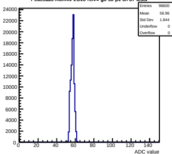
Pedestals mcm41-2C10-refv4-g0-s0-p1 ch 37 test1
