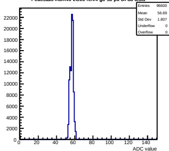
Pedestals mcm41-2C10-refv4-g0-s0-p1 ch 38 test1
