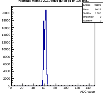
Pedestals mcm41-2C10-refV4-g0-s0-p1 ch 108 test1
