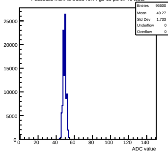
Pedestals mcm41-2C10-refv4-g0-s0-p1 ch 46 test1
