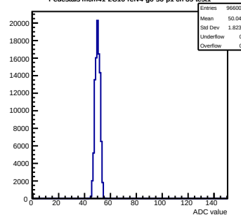
Pedestals mcm41-2C10-refv4-g0-s0-p1 ch 39 test1
