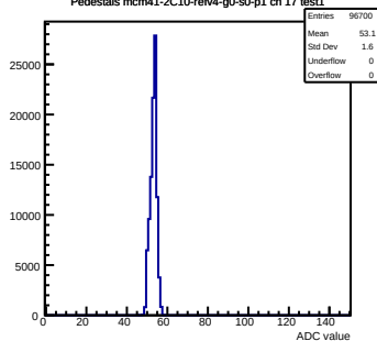
Pedestals mcm41-2C10-refV4-g0-s0-p1 ch 17 test1
