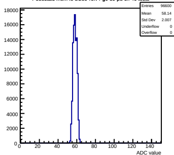
Pedestals mcm41-2C10-refv4-g0-s0-p1 ch 40 test1
