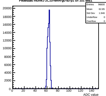
Pedestals mcm41-2C10-refV4-g0-s0-p1 ch 101 test1
