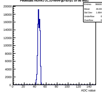
Pedestals mcm41-2C10-refV4-g0-s0-p1 ch 98 test1
