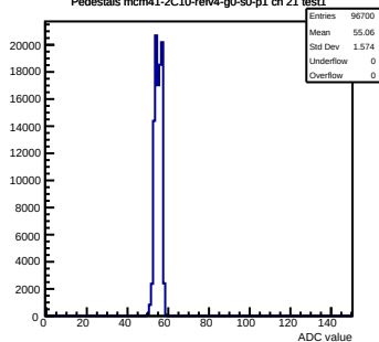
Pedestals mcm41-2C10-refV4-g0-s0-p1 ch 21 test1
