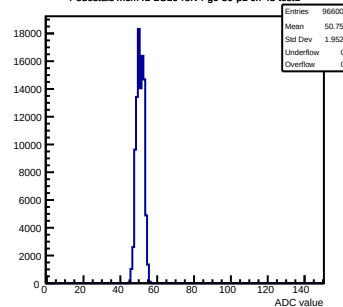
Pedestals mcm41-2C10-refv4-g0-s0-p1 ch 43 test1
