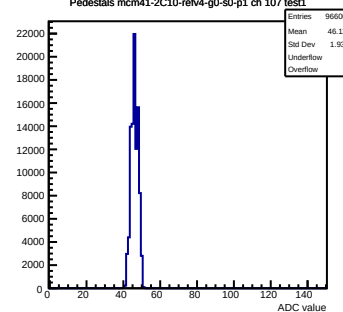
Pedestals mcm41-2C10-refV4-g0-s0-p1 ch 107 test1
