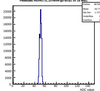
Pedestals mcm41-2C10-refV4-g0-s0-p1 ch 18 test1
