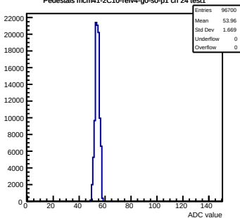
Pedestals mcm41-2C10-refV4-g0-s0-p1 ch 24 test1
