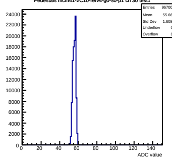
Pedestals mcm41-2C10-refV4-g0-s0-p1 ch 30 test1
