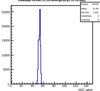
Pedestals mcm41-2C10-refV4-g0-s0-p1 ch 28 test1
