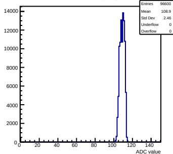
Pedestals mcm42-1412-refV0-g0-s0-p1 ch 37 test1
