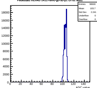
Pedestals mcm42-1412- \text{refV0} -g0-s0-p1 ch 61 test1
