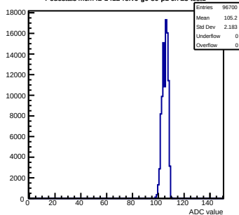
Pedestals mcm42-1412-refV0-g0-s0-p1 ch 23 test1
