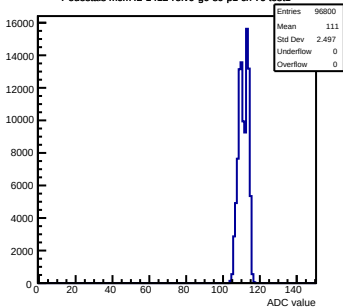
Pedestals mcm42-1412- \text{refV0-g0-s0-p1} ch 76 test1
