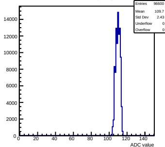
Pedestals mcm42-1412-refV0-g0-s0-p1 ch 34 test1
