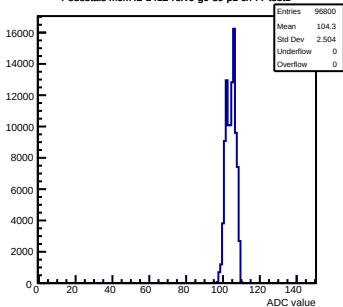
Pedestals mcm42-1412- \text{refV0-g0-s0-p1} ch 77 test1
