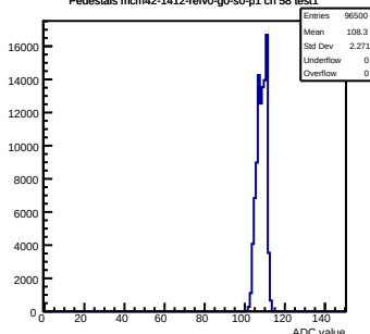
Pedestals mcm42-1412- \text{refV0} -g0-s0-p1 ch 54 test1
