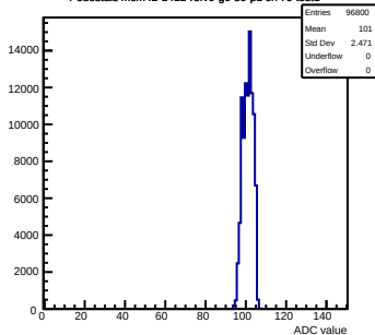
Pedestals mcm42-1412- \text{refV0-g0-s0-p1} ch 79 test1
