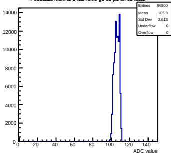
Pedestals mcm42-1412- \text{refV0-g0-s0-p1} ch 68 test1
