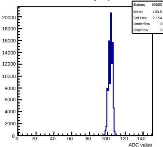
Pedestals mcm42-1412-refv0-g0-s0-p1 ch 126 test1
