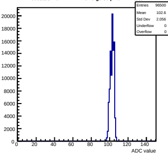
Pedestals mcm42-1412-refv0-g0-s0-p1 ch 121 test1
