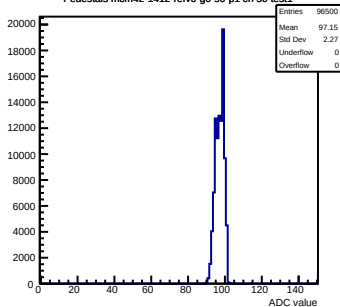
Pedestals mcm42-1412- \text{refV0} -g0-s0-p1 ch 50 test1
