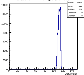
Pedestals mcm42-1412- \text{refV0-g0-s0-p1} ch 65 test1
