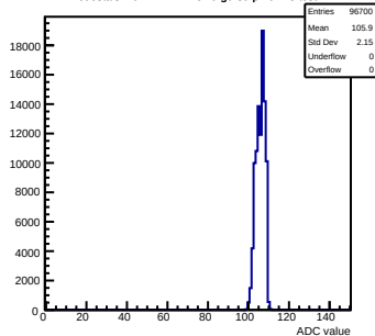
Pedestals mcm42-1412-refV0-g0-s0-p1 ch 25 test1
