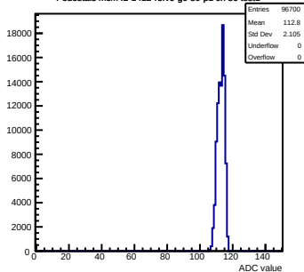
Pedestals mcm42-1412-refV0-g0-s0-p1 ch 86 test1
