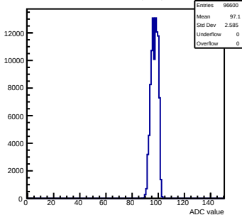
Pedestals mcm42-1412-refV0-g0-s0-p1 ch 32 test1
