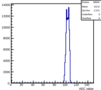
Pedestals mcm42-1412-refV0-g0-s0-p1 ch 36 test1
