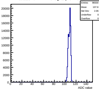
Pedestals mcm42-1412-refv0-g0-s0-p1 ch 118 test1
