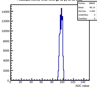
Pedestals mcm42-1412- \text{refV0-g0-s0-p1} ch 69 test1
