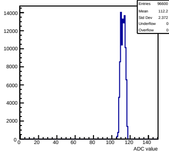
Pedestals mcm42-1412-refV0-g0-s0-p1 ch 46 test1
