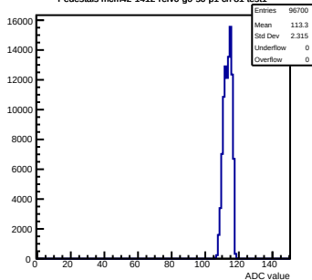
Pedestals mcm42-1412-refV0-g0-s0-p1 ch 81 test1
