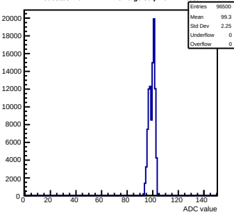
Pedestals mcm42-1412-refv0-g0-s0-p1 ch 117 test1
