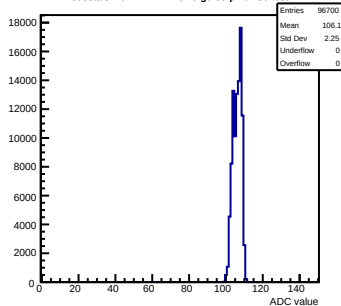
Pedestals mcm42-1412-refV0-g0-s0-p1 ch 30 test1
