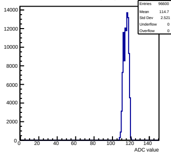
Pedestals mcm42-1412-refV0-g0-s0-p1 ch 33 test1
