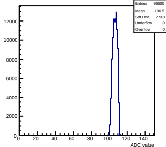
Pedestals mcm42-1412-refV0-g0-s0-p1 ch 45 test1
