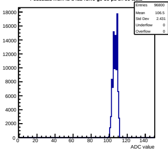
Pedestals mcm42-1412- \text{refV0-g0-s0-p1} ch 66 test1
