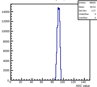
Pedestals mcm42-1412-refv0-g0-s0-p1 ch 124 test1
