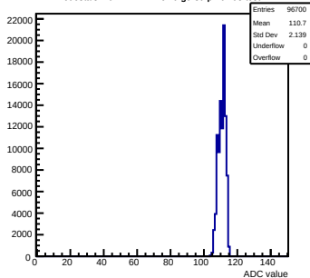
Pedestals mcm42-1412-refV0-g0-s0-p1 ch 93 test1
