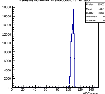
Pedestals mcm42-1412- \text{refV0} -g0-s0-p1 ch 62 test1
