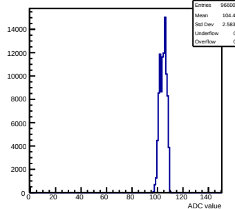
Pedestals mcm42-1412-refV0-g0-s0-p1 ch 43 test1
