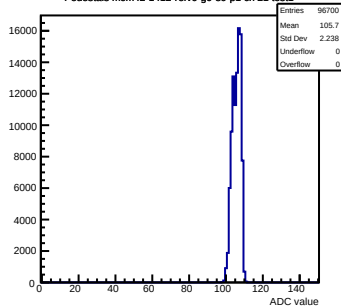
Pedestals mcm42-1412-refV0-g0-s0-p1 ch 21 test1
