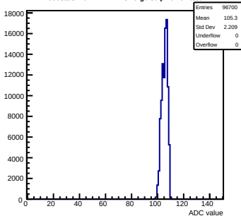
Pedestals mcm42-1412-refV0-g0-s0-p1 ch 92 test1
