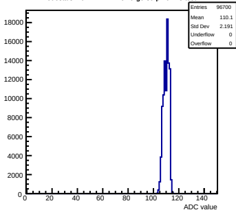
Pedestals mcm42-1412-refV0-g0-s0-p1 ch 28 test1
