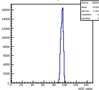
Pedestals mcm42-1412-refv0-g0-s0-p1 ch 127 test1
