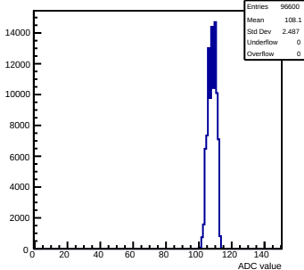
Pedestals mcm42-1412-refV0-g0-s0-p1 ch 44 test1
