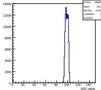
Pedestals mcm42-1412-refV0-g0-s0-p1 ch 47 test1
