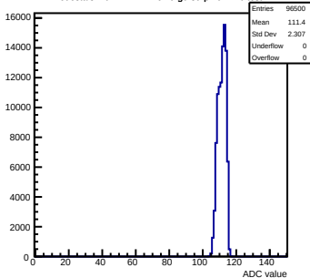
Pedestals mcm42-1412-refv0-g0-s0-p1 ch 116 test1
