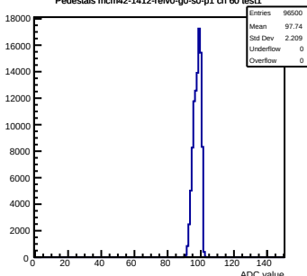
Pedestals mcm42-1412- \text{refV0} -g0-s0-p1 ch 60 test1
