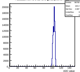
Pedestals mcm42-1412-refV0-g0-s0-p1 ch 87 test1
