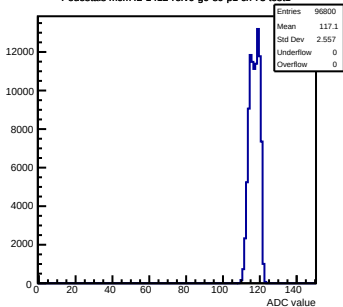
Pedestals mcm42-1412- \text{refV0-g0-s0-p1} ch 73 test1
