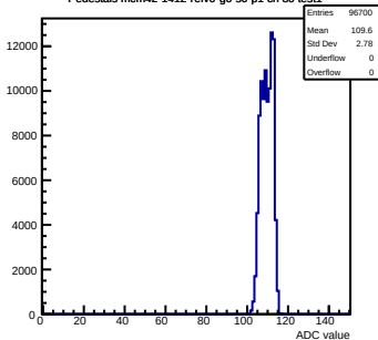
Pedestals mcm42-1412-refV0-g0-s0-p1 ch 80 test1
