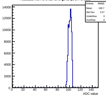
Pedestals mcm42-1412- \text{refV0-g0-s0-p1} ch 75 test1
