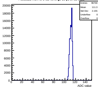
Pedestals mcm42-1412-refV0-g0-s0-p1 ch 22 test1
