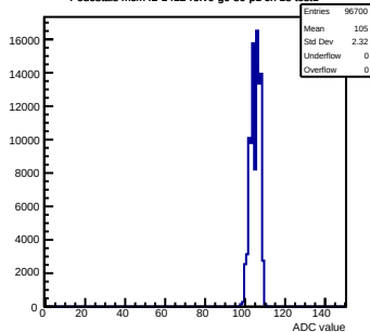
Pedestals mcm42-1412-refV0-g0-s0-p1 ch 18 test1
