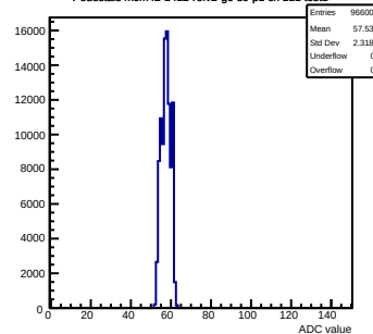
Pedestals mcm42-1412-refv2-g0-s0-p1 ch 111 test1
