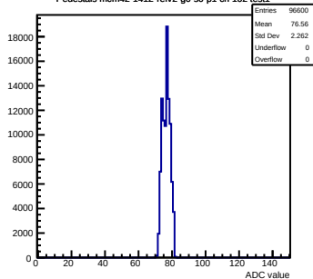
Pedestals mcm42-1412-refv2-g0-s0-p1 ch 102 test1
