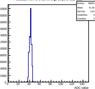
Pedestals mcm42-1412-ref2-g0-s0-p1 ch 125 test1
