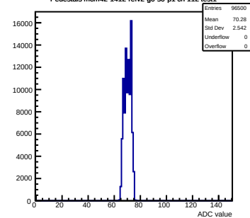
Pedestals mcm42-1412-ref2-g0-s0-p1 ch 112 test1
