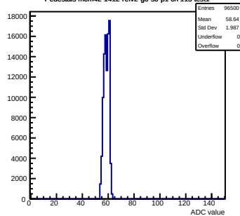
Pedestals mcm42-1412-ref2-g0-s0-p1 ch 115 test1
