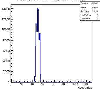
Pedestals mcm42-1412-refv2-g0-s0-p1 ch 104 test1
