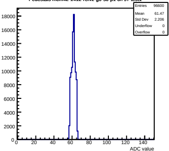
Pedestals mcm42-1412-refv2-g0-s0-p1 ch 97 test1
