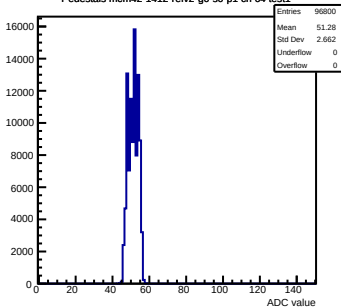
Pedestals mcm42-1412-refv2-g0-s0-p1 ch 64 test1
