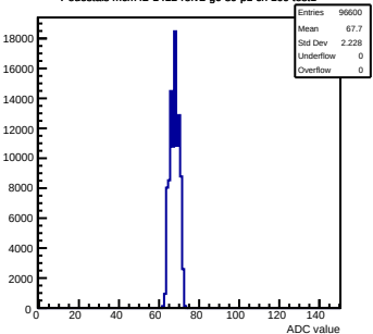
Pedestals mcm42-1412-refv2-g0-s0-p1 ch 109 test1
