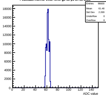
Pedestals mcm42-1412-refv2-g0-s0-p1 ch 98 test1
