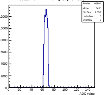
Pedestals mcm42-1412-refv2-g0-s0-p1 ch 73 test1
