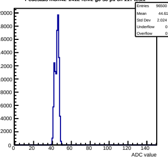
Pedestals mcm42-1412-ref2-g0-s0-p1 ch 117 test1
