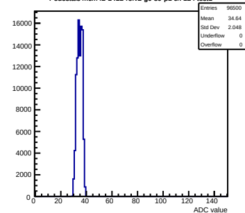
Pedestals mcm42-1412-ref2-g0-s0-p1 ch 124 test1
