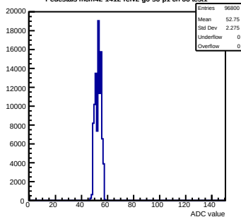
Pedestals mcm42-1412-refv2-g0-s0-p1 ch 66 test1
