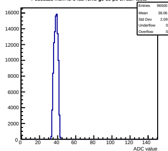
Pedestals mcm42-1412-ref2-g0-s0-p1 ch 127 test1
