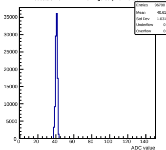
Pedestals mcm2-1412-refv4-g0-s0-p1 ch 29 test1
