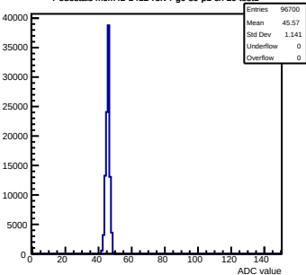
Pedestals mcm2-1412-refv4-g0-s0-p1 ch 20 test1
