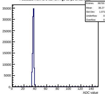
Pedestals mcm2-1412-refv4-g0-s0-p1 ch 21 test1
