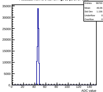
Pedestals mcm2-1412-refv4-g0-s0-p1 ch 17 test1
