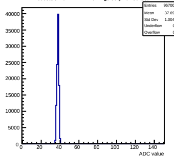
Pedestals mcm2-1412-refv4-g0-s0-p1 ch 30 test1
