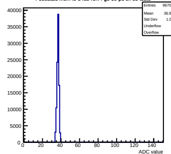
Pedestals mcm2-1412-refv4-g0-s0-p1 ch 19 test1
