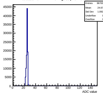
Pedestals mcm2-1412-refv4-g0-s0-p1 ch 26 test1
