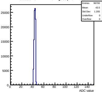
Pedestals mcm2-1412-refv4-g0-s0-p1 ch 24 test1
