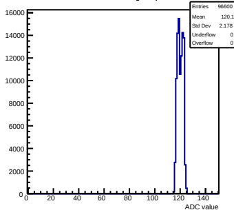
Pedestals mcm42-1412-refv6-g0-s0-p1 ch 106 test1
