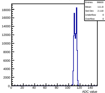
Pedestals mcm42-1412-refv6-g0-s0-p1 ch 96 test1
