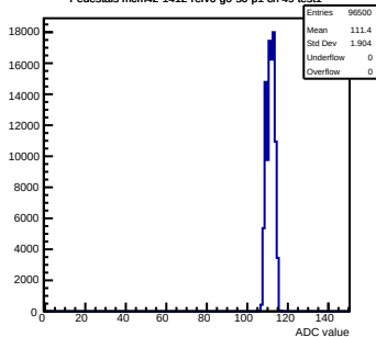
Pedestals mcm42-1412- refv6-g0-s0-p1 ch 49 test1
