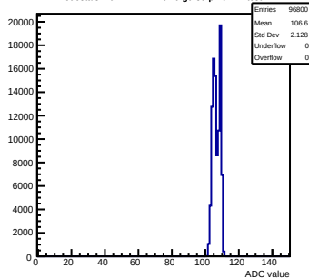
Pedestals mcm42-1412-rlv6-g0-s0-p1 ch 77 test1
