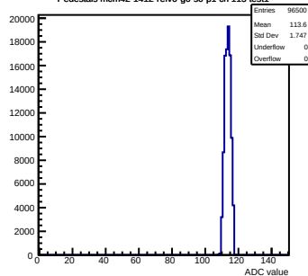
Pedestals mcm42-1412-refv6-g0-s0-p1 ch 115 test1
