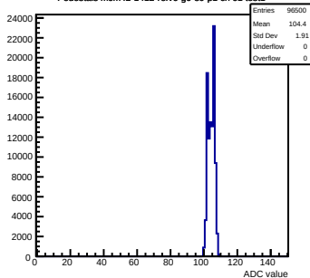
Pedestals mcm42-1412- refv6-g0-s0-p1 ch 61 test1
