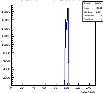
Pedestals mcm42-1412- refv6-g0-s0-p1 ch 60 test1
