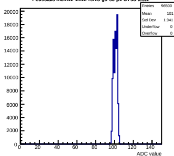
Pedestals mcm42-1412- refv6-g0-s0-p1 ch 53 test1
