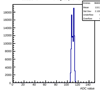
Pedestals mcm42-1412-rlv6-g0-s0-p1 ch 78 test1
