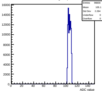
Pedestals mcm42-1412-refv6-g0-s0-p1 ch 100 test1
