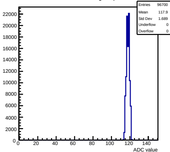
Pedestals mcm42-1412-rlv6-g0-s0-p1 ch 95 test1
