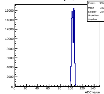
Pedestals mcm42-1412-rlv6-g0-s0-p1 ch 79 test1
