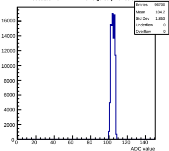
Pedestals mcm42-1412-rlv6-g0-s0-p1 ch 85 test1
