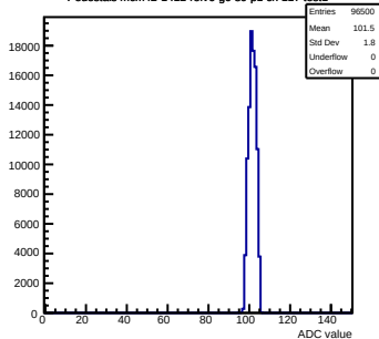
Pedestals mcm42-1412-refv6-g0-s0-p1 ch 117 test1
