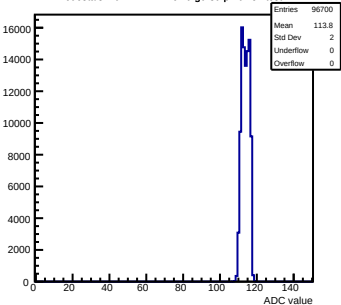
Pedestals mcm42-1412-rlv6-g0-s0-p1 ch 81 test1
