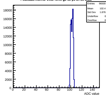
Pedestals mcm42-1412- refv6-g0-s0-p1 ch 51 test1
