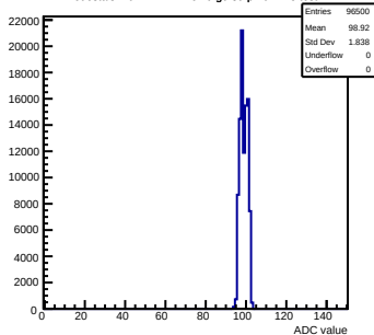
Pedestals mcm42-1412-refv6-g0-s0-p1 ch 125 test1
