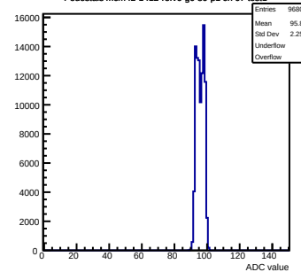
Pedestals mcm42-1412-rlv6-g0-s0-p1 ch 67 test1
