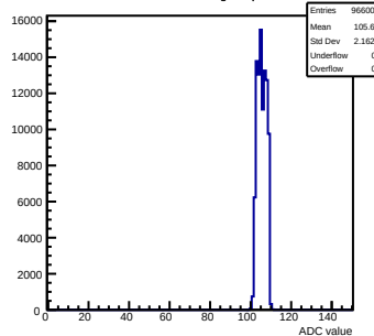
Pedestals mcm42-1412-refv6-g0-s0-p1 ch 107 test1
