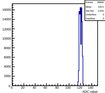
Pedestals mcm42-1412-refv6-g0-s0-p1 ch 109 test1
