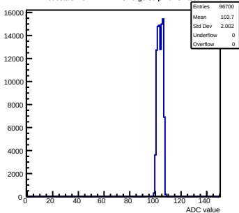
Pedestals mcm42-1412-rlv6-g0-s0-p1 ch 84 test1
