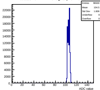
Pedestals mcm42-1412-refv6-g0-s0-p1 ch 126 test1
