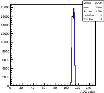
Pedestals mcm42-1412-rlv6-g0-s0-p1 ch 89 test1
