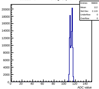
Pedestals mcm42-1412-rlv6-g0-s0-p1 ch 76 test1
