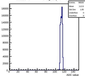
Pedestals mcm42-1412-refv6-g0-s0-p1 ch 120 test1
