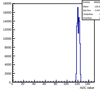
Pedestals mcm42-1412-refv6-g0-s0-p1 ch 103 test1
