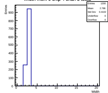
Width mcm 0 chip 4 chan 3 test1
