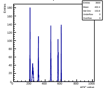
Pulse mcm 0 chip 3 chan 15 test1
