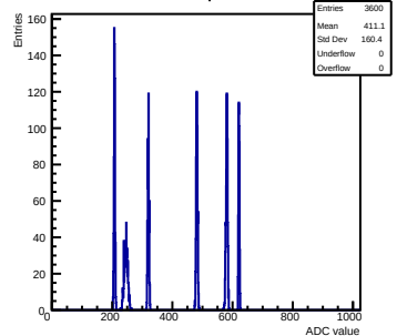
Pulse mcm 0 chip 3 chan 3 test1
