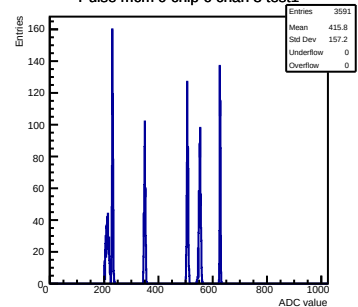
Pulse mcm 0 chip 6 chan 3 test1
