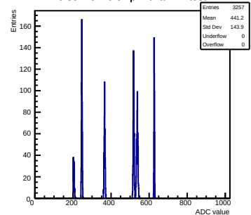
Pulse mcm 0 chip 2 chan 11 test1
