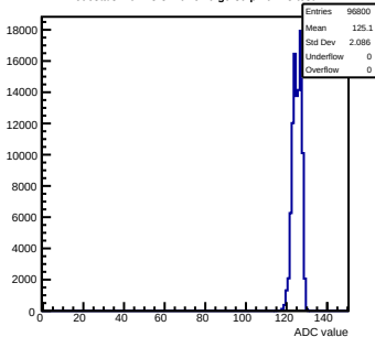
Pedestals mcm43-3410-refV0-g0-s0-p1 ch 73 test1
