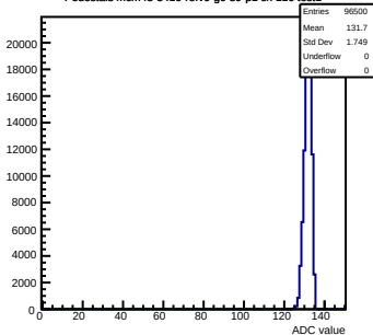
Pedestals mcm43-3410-refV0-g0-s0-p1 ch 116 test1
