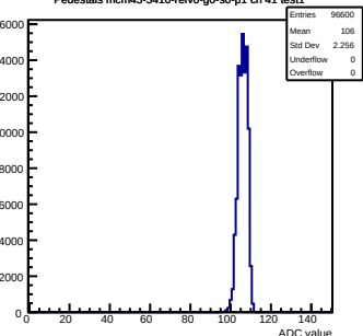
Pedestals mcm43-3410-refV0-g0-s0-p1 ch 41 test1
