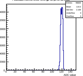
Pedestals mcm43-3410-refV0-g0-s0-p1 ch 33 test1
