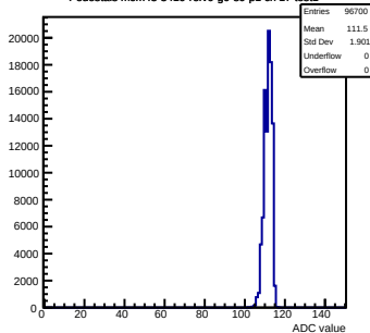
Pedestals mcm43-3410-refV0-g0-s0-p1 ch 17 test1
