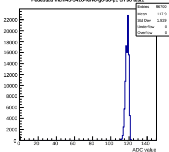
Pedestals mcm43-3410-refV0-g0-s0-p1 ch 90 test1
