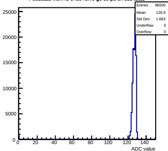
Pedestals mcm43-3410-refV0-g0-s0-p1 ch 118 test1
