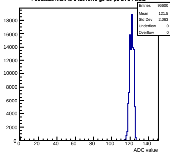
Pedestals mcm43-3410-refV0-g0-s0-p1 ch 34 test1
