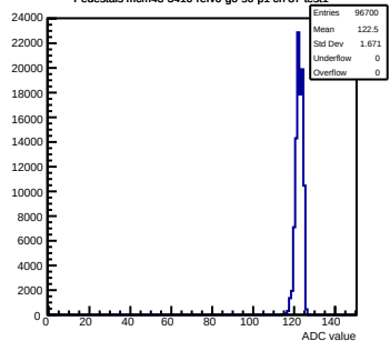
Pedestals mcm43-3410-refV0-g0-s0-p1 ch 87 test1
