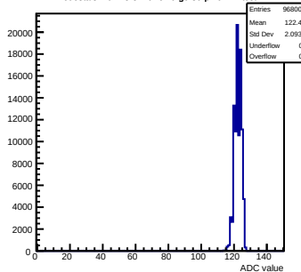
Pedestals mcm43-3410-refV0-g0-s0-p1 ch 74 test1
