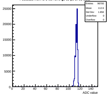
Pedestals mcm43-3410-refV0-g0-s0-p1 ch 93 test1
