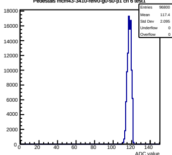
Pedestals mcm43-3410-refv0-g0-s0-p1 ch 6 test1
