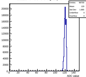
Pedestals mcm43-3410-refV0-g0-s0-p1 ch 28 test1
