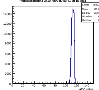
Pedestals mcm43-3410-refv0-g0-s0-p1 ch 15 test1
