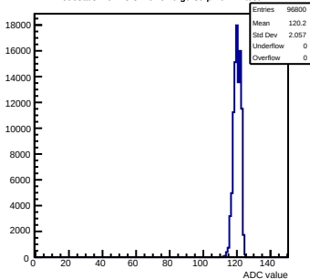
Pedestals mcm43-3410-refV0-g0-s0-p1 ch 77 test1
