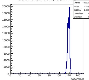
Pedestals mcm43-3410-refV0-g0-s0-p1 ch 70 test1
