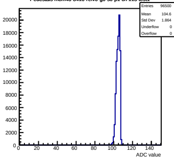
Pedestals mcm43-3410-refV0-g0-s0-p1 ch 115 test1
