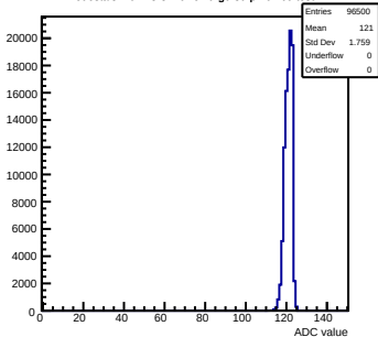
Pedestals mcm43-3410-refV0-g0-s0-p1 ch 60 test1
