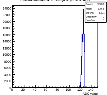
Pedestals mcm43-3410-refV0-g0-s0-p1 ch 89 test1
