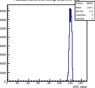
Pedestals mcm43-3410-refV0-g0-s0-p1 ch 37 test1
