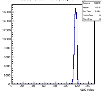
Pedestals mcm43-3410-refV0-g0-s0-p1 ch 101 test1
