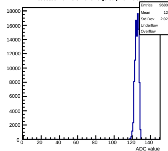
Pedestals mcm43-3410-refV0-g0-s0-p1 ch 75 test1
