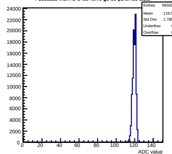
Pedestals mcm43-3410-refV0-g0-s0-p1 ch 51 test1
