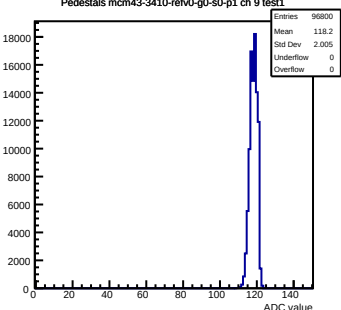
Pedestals mcm43-3410-refv0-g0-s0-p1 ch 9 test1
