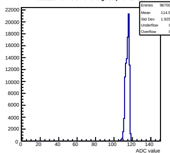
Pedestals mcm43-3410-refV0-g0-s0-p1 ch 30 test1
