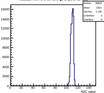
Pedestals mcm43-3410-refV0-g0-s0-p1 ch 68 test1
