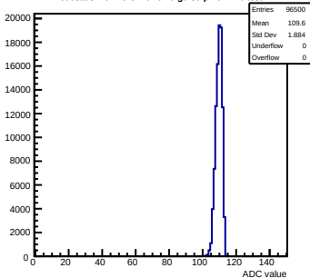
Pedestals mcm43-3410-refV0-g0-s0-p1 ch 126 test1
