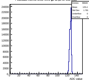
Pedestals mcm43-3410-refV0-g0-s0-p1 ch 113 test1
