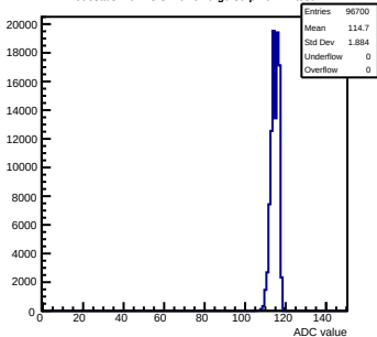
Pedestals mcm43-3410-refV0-g0-s0-p1 ch 24 test1
