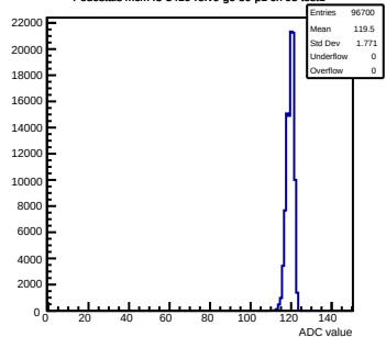
Pedestals mcm43-3410-refV0-g0-s0-p1 ch 95 test1
