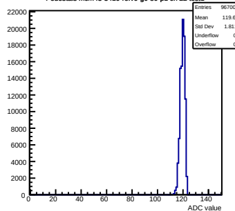
Pedestals mcm43-3410-refV0-g0-s0-p1 ch 22 test1
