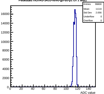
Pedestals mcm43-3410-refv0-g0-s0-p1 ch 1 test1
