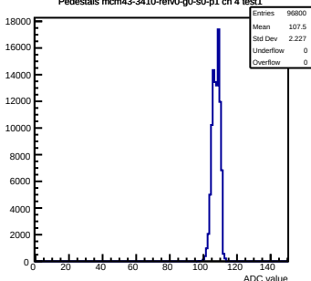
Pedestals mcm43-3410-refv0-g0-s0-p1 ch 4 test1
