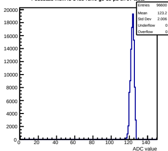
Pedestals mcm43-3410-refV0-g0-s0-p1 ch 97 test1
