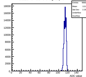
Pedestals mcm43-3410-refV0-g0-s0-p1 ch 111 test1
