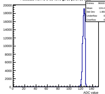
Pedestals mcm43-3410-refV0-g0-s0-p1 ch 50 test1
