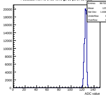
Pedestals mcm43-3410-refV0-g0-s0-p1 ch 18 test1
