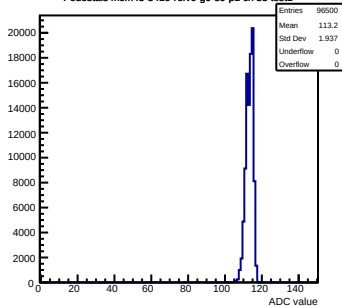
Pedestals mcm43-3410-refV0-g0-s0-p1 ch 53 test1
