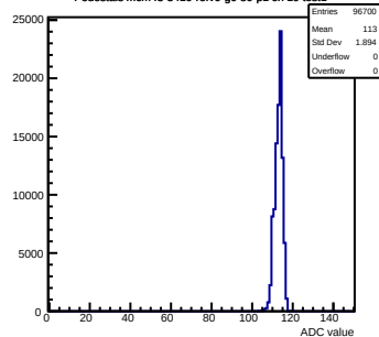
Pedestals mcm43-3410-refV0-g0-s0-p1 ch 19 test1
