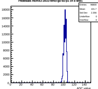
Pedestals mcm43-3410-refv0-g0-s0-p1 ch 8 test1
