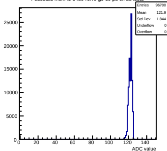
Pedestals mcm43-3410-refV0-g0-s0-p1 ch 21 test1
