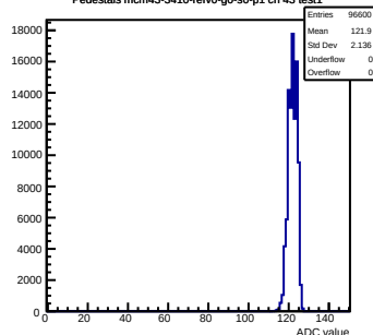
Pedestals mcm43-3410-refV0-g0-s0-p1 ch 43 test1
