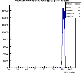
Pedestals mcm43-3410-refv0-g0-s0-p1 ch 10 test1
