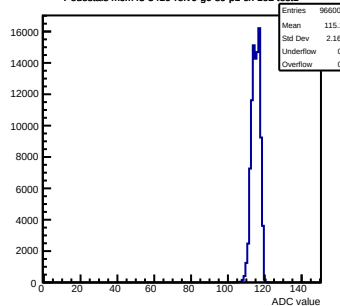
Pedestals mcm43-3410-refV0-g0-s0-p1 ch 102 test1
