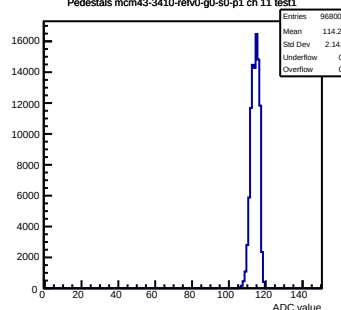
Pedestals mcm43-3410-refv0-g0-s0-p1 ch 11 test1
