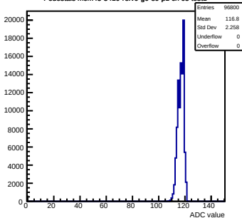
Pedestals mcm43-3410-refV0-g0-s0-p1 ch 65 test1
