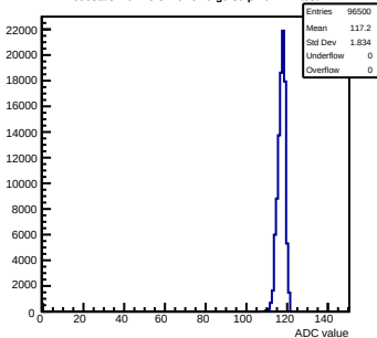
Pedestals mcm43-3410-refV0-g0-s0-p1 ch 127 test1
