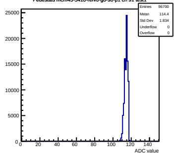
Pedestals mcm43-3410-refV0-g0-s0-p1 ch 91 test1
