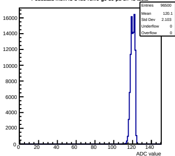
Pedestals mcm43-3410-refV0-g0-s0-p1 ch 48 test1
