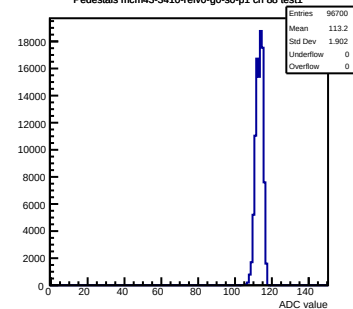
Pedestals mcm43-3410-refV0-g0-s0-p1 ch 88 test1
