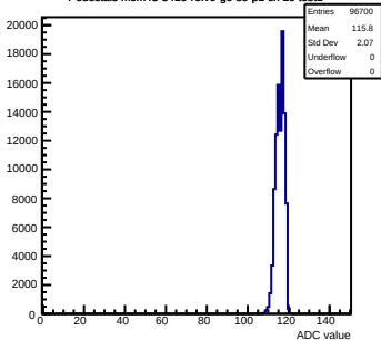
Pedestals mcm43-3410-refV0-g0-s0-p1 ch 20 test1
