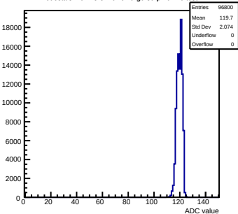
Pedestals mcm43-3410-refV0-g0-s0-p1 ch 76 test1
