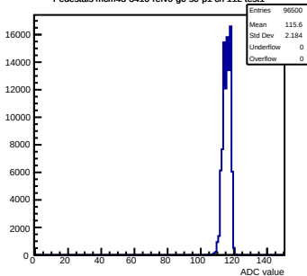
Pedestals mcm43-3410-refV0-g0-s0-p1 ch 112 test1
