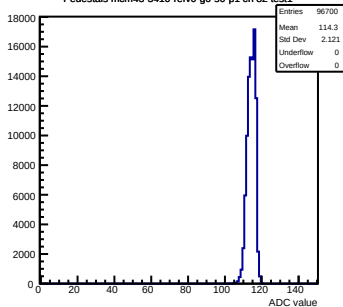
Pedestals mcm43-3410-refV0-g0-s0-p1 ch 82 test1
