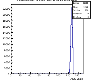
Pedestals mcm43-3410-refV0-g0-s0-p1 ch 83 test1
