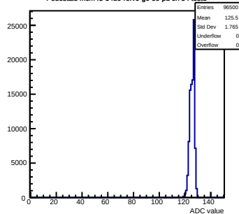
Pedestals mcm43-3410-refV0-g0-s0-p1 ch 54 test1
