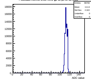
Pedestals mcm43-3410-refV0-g0-s0-p1 ch 80 test1
