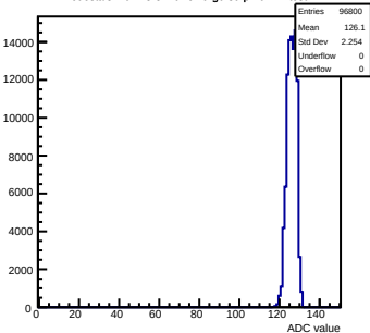
Pedestals mcm43-3410-refV0-g0-s0-p1 ch 72 test1
