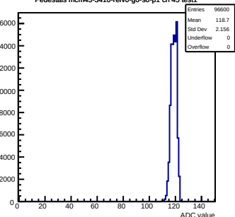
Pedestals mcm43-3410-refV0-g0-s0-p1 ch 45 test1
