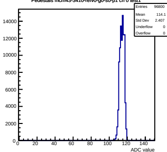
Pedestals mcm43-3410-refv0-g0-s0-p1 ch 0 test1
