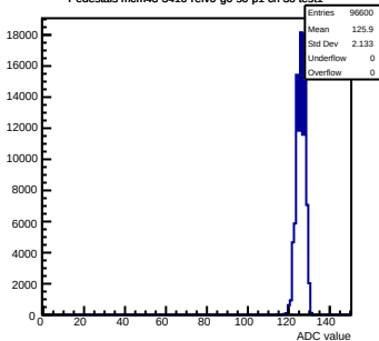
Pedestals mcm43-3410-refV0-g0-s0-p1 ch 36 test1
