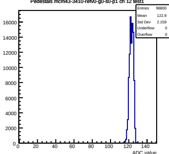
Pedestals mcm43-3410-refv0-g0-s0-p1 ch 12 test1
