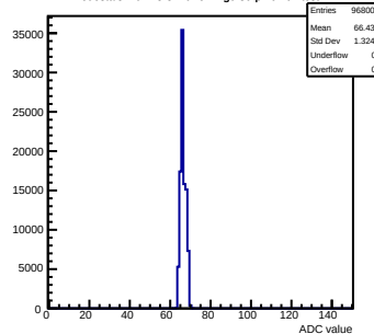
Pedestals mcm43-3410-refv2-g0-s0-p1 ch 67 test1
