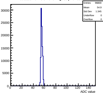
Pedestals mcm43-3410-refv2-g0-s0-p1 ch 68 test1
