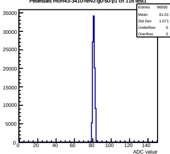
Pedestals mcm43-3410-refv2-g0-s0-p1 ch 116 test1
