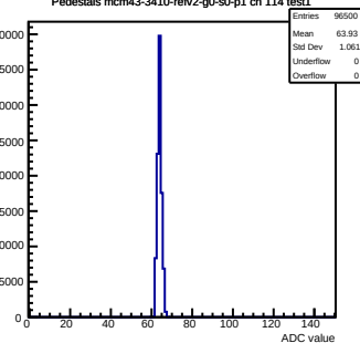
Pedestals mcm43-3410-refv2-g0-s0-p1 ch 114 test1
