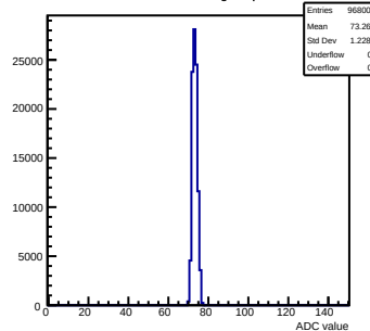
Pedestals mcm43-3410-refv2-g0-s0-p1 ch 75 test1
