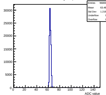
Pedestals mcm43-3410-refv2-g0-s0-p1 ch 79 test1
