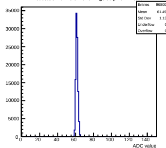
Pedestals mcm43-3410-refv2-g0-s0-p1 ch 71 test1
