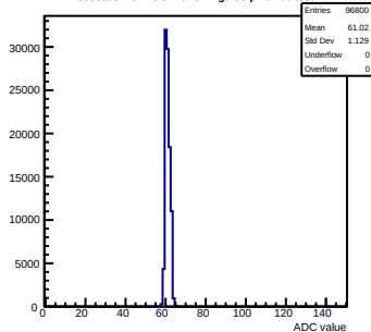
Pedestals mcm43-3410-refv2-g0-s0-p1 ch 66 test1
