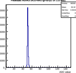
Pedestals mcm43-3410-refv2-g0-s0-p1 ch 115 test1
