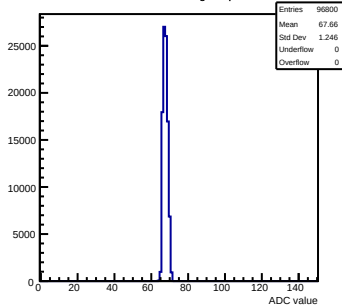
Pedestals mcm43-3410-refv2-g0-s0-p1 ch 77 test1
