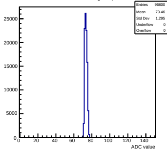
Pedestals mcm43-3410-refv2-g0-s0-p1 ch 73 test1
