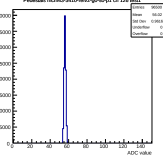
Pedestals mcm43-3410-refv2-g0-s0-p1 ch 126 test1
