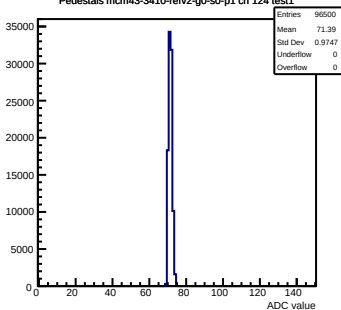
Pedestals mcm43-3410-refv2-g0-s0-p1 ch 124 test1
