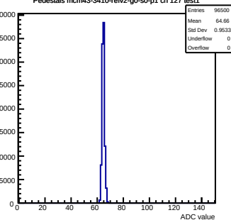
Pedestals mcm43-3410-refv2-g0-s0-p1 ch 127 test1
