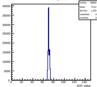
Pedestals mcm43-3410-refv2-g0-s0-p1 ch 74 test1
