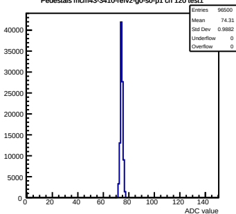
Pedestals mcm43-3410-refv2-g0-s0-p1 ch 120 test1
