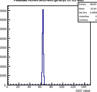
Pedestals mcm43-3410-refv2-g0-s0-p1 ch 122 test1
