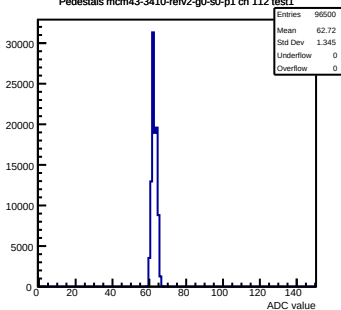
Pedestals mcm43-3410-refv2-g0-s0-p1 ch 112 test1
