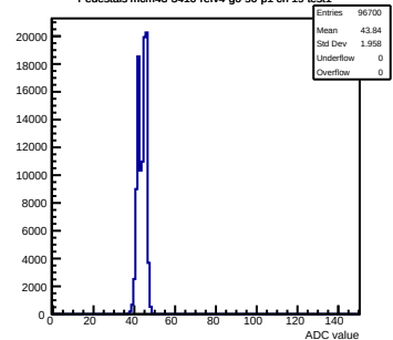
Pedestals mcm43-3410-refv4-g0-s0-p1 ch 19 test1
