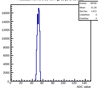
Pedestals mcm43-3410-refv4-g0-s0-p1 ch 28 test1
