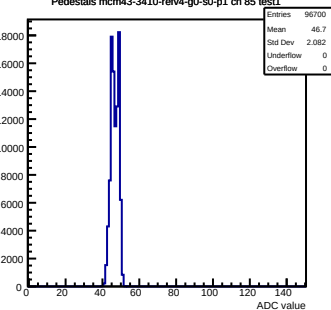
Pedestals mcm43-3410-refv4-g0-s0-p1 ch 85 test1
