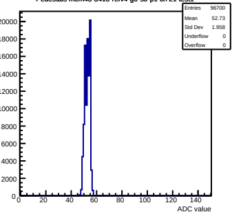
Pedestals mcm43-3410-refv4-g0-s0-p1 ch 21 test1
