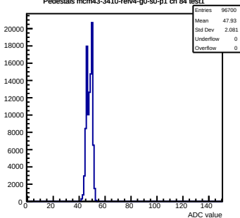
Pedestals mcm43-3410-refv4-g0-s0-p1 ch 84 test1
