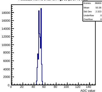
Pedestals mcm43-3410-refv4-g0-s0-p1 ch 70 test1
