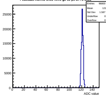
Pedestals mcm43-3410- rev6-g0-s0-p1 ch 70 test1
