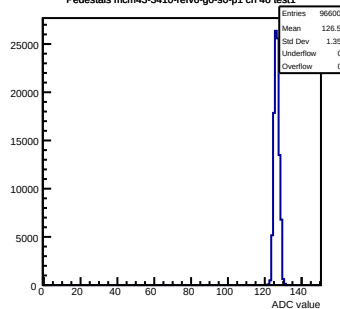
Pedestals mcm43-3410-rlv6-g0-s0-p1 ch 46 test1
