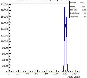
Pedestals mcm43-3410-rlv6-g0-s0-p1 ch 96 test1
