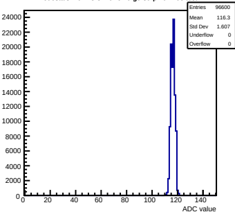
Pedestals mcm43-3410-rlv6-g0-s0-p1 ch 108 test1
