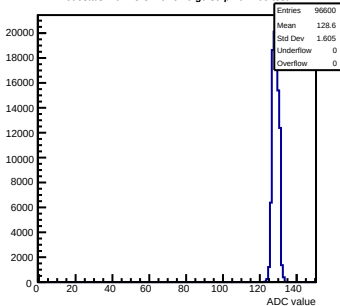
Pedestals mcm43-3410-rlv6-g0-s0-p1 ch 109 test1
