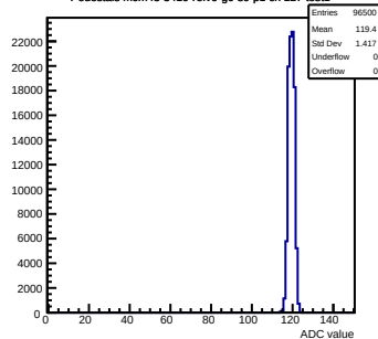
Pedestals mcm43-3410-refv6-g0-s0-p1 ch 127 test1
