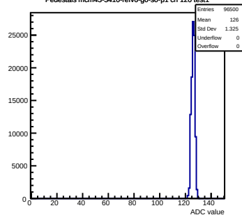
Pedestals mcm43-3410-refv6-g0-s0-p1 ch 120 test1
