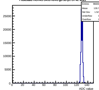
Pedestals mcm43-3410-rlv6-g0-s0-p1 ch 42 test1
