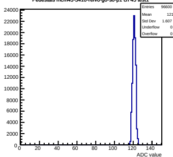
Pedestals mcm43-3410-rlv6-g0-s0-p1 ch 45 test1
