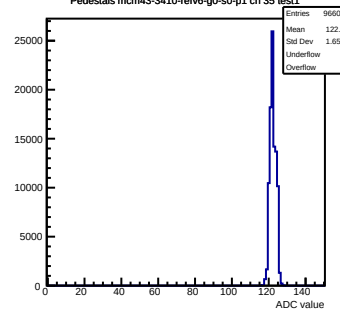
Pedestals mcm43-3410-rlv6-g0-s0-p1 ch 35 test1
