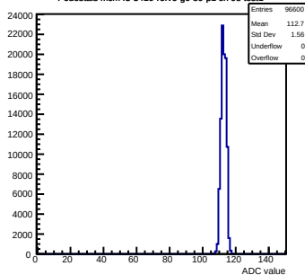
Pedestals mcm43-3410-rlv6-g0-s0-p1 ch 98 test1
