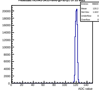
Pedestals mcm43-3410-rlv6-g0-s0-p1 ch 33 test1
