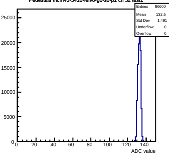
Pedestals mcm43-3410-rlv6-g0-s0-p1 ch 32 test1
