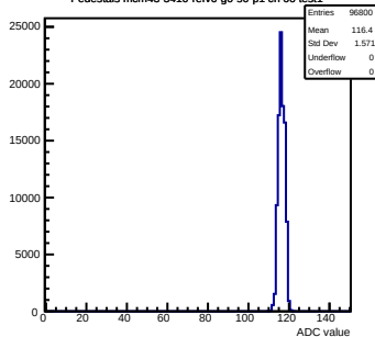
Pedestals mcm43-3410- rev6-g0-s0-p1 ch 66 test1
