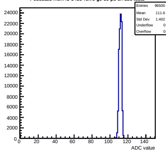
Pedestals mcm43-3410-refv6-g0-s0-p1 ch 126 test1
