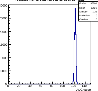
Pedestals mcm43-3410-refv6-g0-s0-p1 ch 117 test1
