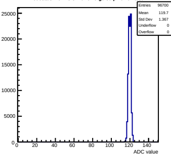
Pedestals mcm43-3410- rev6 -g0-s0-p1 ch 92 test1
