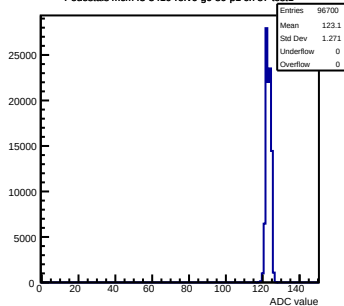
Pedestals mcm43-3410- rev6 -g0-s0-p1 ch 87 test1
