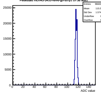
Pedestals mcm43-3410-rlv6-g0-s0-p1 ch 38 test1
