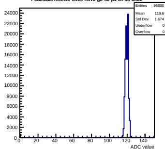
Pedestals mcm43-3410- rev6-g0-s0-p1 ch 65 test1
