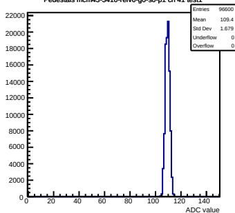
Pedestals mcm43-3410-rlv6-g0-s0-p1 ch 41 test1
