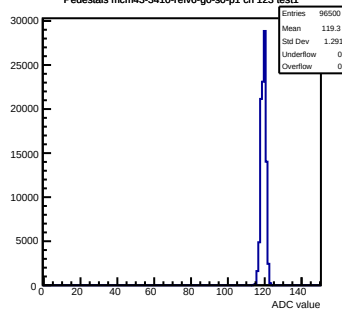
Pedestals mcm43-3410-refv6-g0-s0-p1 ch 123 test1
