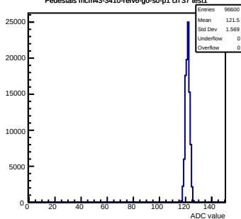
Pedestals mcm43-3410-rlv6-g0-s0-p1 ch 37 test1
