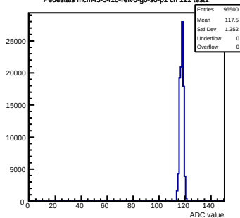
Pedestals mcm43-3410-refv6-g0-s0-p1 ch 122 test1
