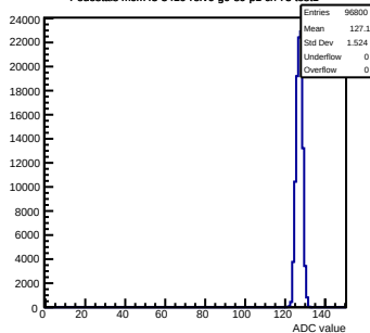
Pedestals mcm43-3410- rev6-g0-s0-p1 ch 73 test1
