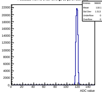
Pedestals mcm43-3410-rlv6-g0-s0-p1 ch 101 test1
