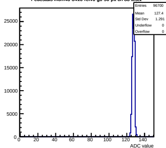
Pedestals mcm43-3410- rev6 -g0-s0-p1 ch 83 test1
