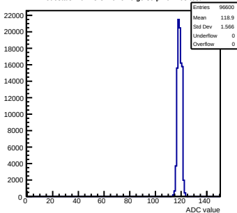
Pedestals mcm43-3410-rlv6-g0-s0-p1 ch 105 test1
