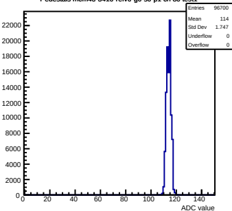
Pedestals mcm43-3410- rev6 -g0-s0-p1 ch 80 test1
