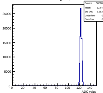
Pedestals mcm43-3410-rlv6-g0-s0-p1 ch 106 test1
