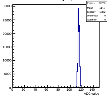
Pedestals mcm43-3410- rev6 -g0-s0-p1 ch 93 test1
