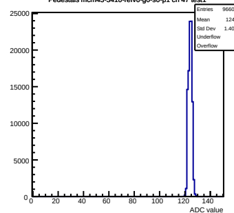
Pedestals mcm43-3410-rlv6-g0-s0-p1 ch 47 test1
