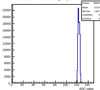
Pedestals mcm43-3410-rlv6-g0-s0-p1 ch 110 test1
