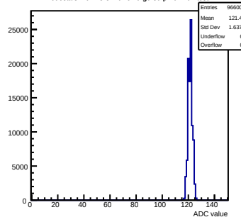
Pedestals mcm43-3410-rlv6-g0-s0-p1 ch 107 test1
