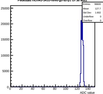
Pedestals mcm43-3410-rlv6-g0-s0-p1 ch 36 test1
