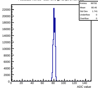
Pedestals mcm50-4812-rv1-g0-s0-p1 ch 93 test1
