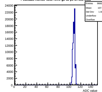
Pedestals mcm50-4812-refv1-g0-s0-p1 ch 103 test1
