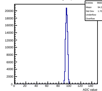
Pedestals mcm50-4812-refv1-g0-s0-p1 ch 47 test1
