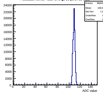
Pedestals mcm50-4812-refv1-g0-s0-p1 ch 98 test1
