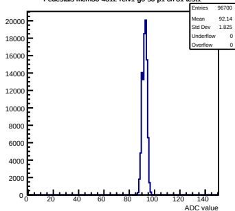
Pedestals mcm50-4812-rv1-g0-s0-p1 ch 81 test1
