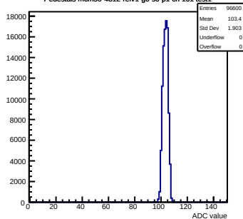
Pedestals mcm50-4812-refv1-g0-s0-p1 ch 101 test1
