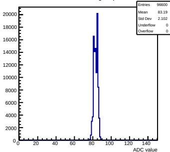
Pedestals mcm50-4812-refv1-g0-s0-p1 ch 40 test1
