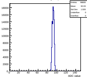
Pedestals mcm50-4812-refv1-g0-s0-p1 ch 44 test1
