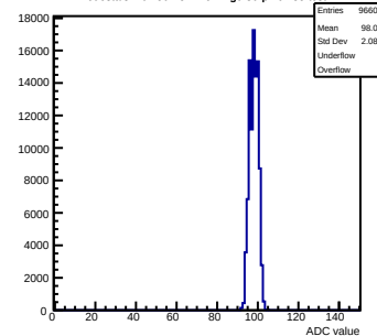
Pedestals mcm50-4812-refv1-g0-s0-p1 ch 35 test1
