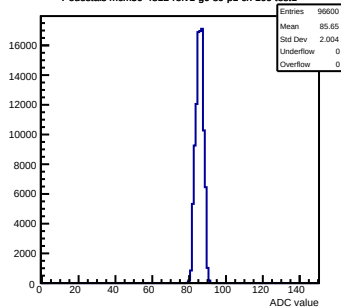
Pedestals mcm50-4812-refv1-g0-s0-p1 ch 109 test1
