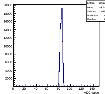
Pedestals mcm50-4812-refv1-g0-s0-p1 ch 42 test1
