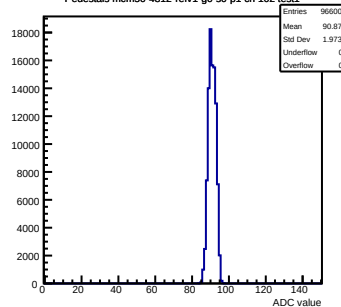
Pedestals mcm50-4812-refv1-g0-s0-p1 ch 102 test1
