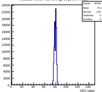
Pedestals mcm50-4812-rv1-g0-s0-p1 ch 94 test1
