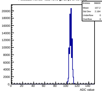
Pedestals mcm50-4812-refv1-g0-s0-p1 ch 96 test1
