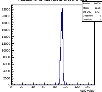
Pedestals mcm50-4812-rv1-g0-s0-p1 ch 84 test1
