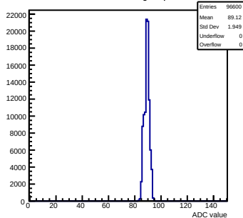
Pedestals mcm50-4812-refv1-g0-s0-p1 ch 41 test1
