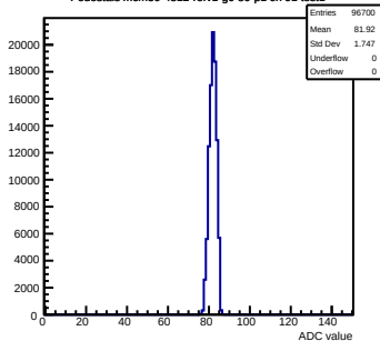
Pedestals mcm50-4812-rv1-g0-s0-p1 ch 91 test1
