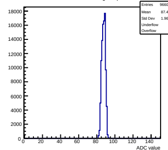
Pedestals mcm50-4812-refv1-g0-s0-p1 ch 43 test1
