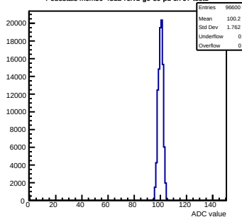
Pedestals mcm50-4812-refv1-g0-s0-p1 ch 97 test1
