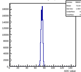
Pedestals mcm50-4812-refv1-g0-s0-p1 ch 45 test1
