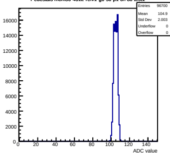
Pedestals mcm50-4812-rv1-g0-s0-p1 ch 80 test1
