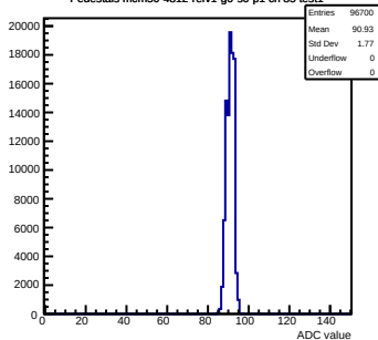
Pedestals mcm50-4812-rv1-g0-s0-p1 ch 85 test1
