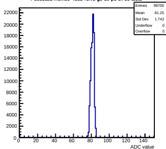
Pedestals mcm50-4812-rv1-g0-s0-p1 ch 89 test1
