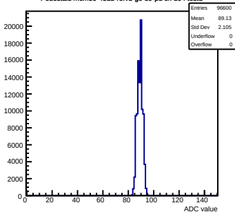
Pedestals mcm50-4812-refv1-g0-s0-p1 ch 104 test1
