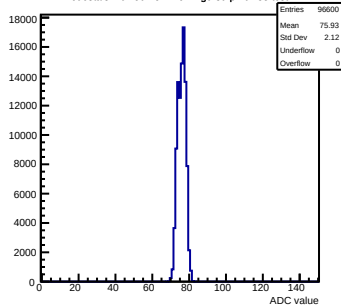
Pedestals mcm50-4812-refv1-g0-s0-p1 ch 33 test1
