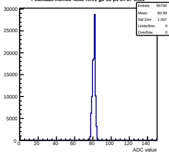
Pedestals mcm50-4812-rv1-g0-s0-p1 ch 87 test1
