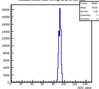
Pedestals mcm50-4812-refv1-g0-s0-p1 ch 100 test1
