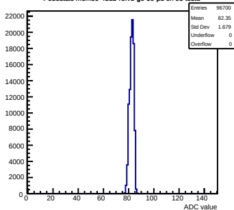
Pedestals mcm50-4812-rv1-g0-s0-p1 ch 95 test1
