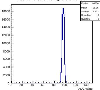
Pedestals mcm50-4812-refv1-g0-s0-p1 ch 108 test1
