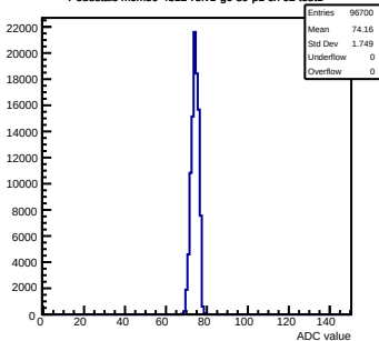
Pedestals mcm50-4812-rv1-g0-s0-p1 ch 92 test1
