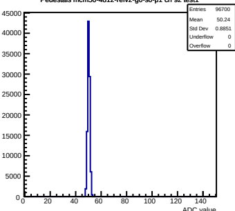
Pedestals mcm50-4812-refV2-g0-s0-p1 ch 92 test1
