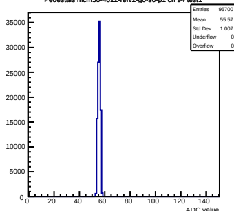
Pedestals mcm50-4812-refV2-g0-s0-p1 ch 94 test1
