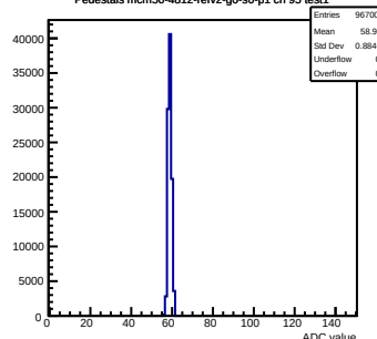
Pedestals mcm50-4812-refV2-g0-s0-p1 ch 95 test1
