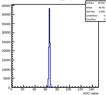
Pedestals mcm50-4812-refv2-g0-s0-p1 ch 25 test1
