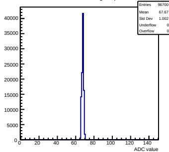
Pedestals mcm50-4812-refv2-g0-s0-p1 ch 26 test1
