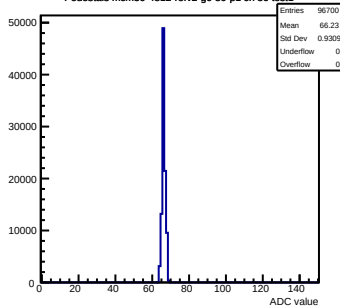
Pedestals mcm50-4812-refV2-g0-s0-p1 ch 86 test1
