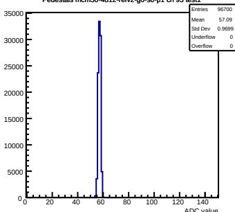
Pedestals mcm50-4812-refV2-g0-s0-p1 ch 93 test1
