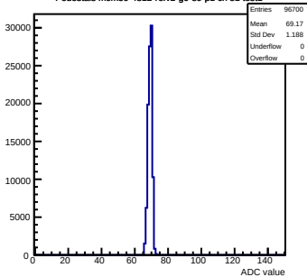
Pedestals mcm50-4812-refV2-g0-s0-p1 ch 81 test1
