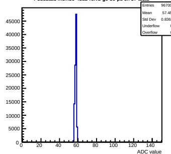
Pedestals mcm50-4812-refV2-g0-s0-p1 ch 87 test1
