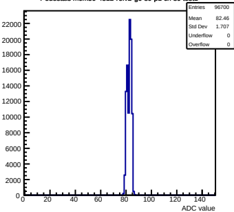
Pedestals mcm50-4812-refV2-g0-s0-p1 ch 80 test1
