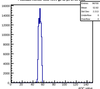
Pedestals mcm50-4812-refv4-g0-s0-p1 ch 20 test1
