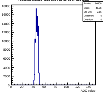
Pedestals mcm50-4812-refv4-g0-s0-p1 ch 116 test1
