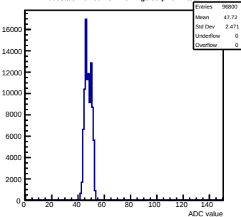
Pedestals mcm50-4812-refv4-g0-s0-p1 ch 4 test1
