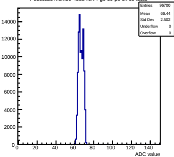
Pedestals mcm50-4812-refv4-g0-s0-p1 ch 80 test1
