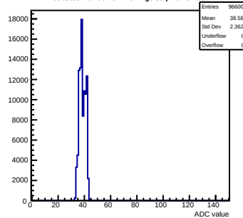
Pedestals mcm50-4812-refv4-g0-s0-p1 ch 34 test1
