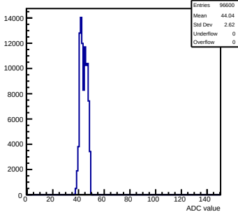
Pedestals mcm50-4812-refv4-g0-s0-p1 ch 40 test1
