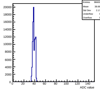
Pedestals mcm50-4812-refv4-g0-s0-p1 ch 46 test1
