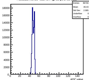
Pedestals mcm50-4812-refv4-g0-s0-p1 ch 30 test1
