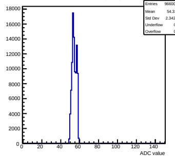
Pedestals mcm50-4812-refv4-g0-s0-p1 ch 38 test1
