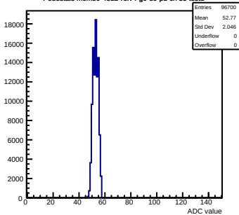
Pedestals mcm50-4812-refv4-g0-s0-p1 ch 85 test1
