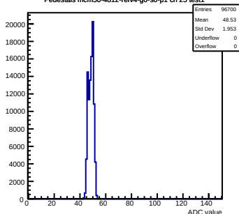
Pedestals mcm50-4812-refv4-g0-s0-p1 ch 25 test1
