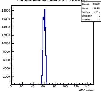
Pedestals mcm50-4812-refv4-g0-s0-p1 ch 124 test1
