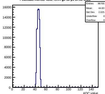
Pedestals mcm50-4812-refv4-g0-s0-p1 ch 22 test1
