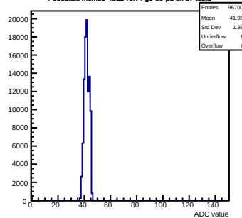
Pedestals mcm50-4812-refv4-g0-s0-p1 ch 87 test1
