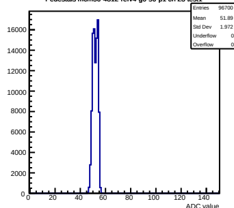
Pedestals mcm50-4812-refv4-g0-s0-p1 ch 23 test1
