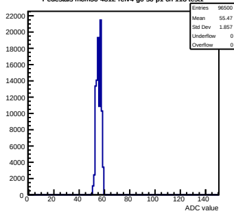
Pedestals mcm50-4812-refv4-g0-s0-p1 ch 118 test1
