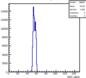
Pedestals mcm50-4812-refv4-g0-s0-p1 ch 8 test1
