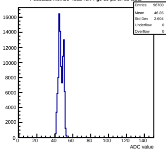
Pedestals mcm50-4812-refv4-g0-s0-p1 ch 16 test1
