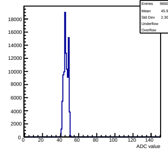
Pedestals mcm50-4812-refv4-g0-s0-p1 ch 39 test1
