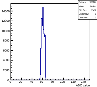
Pedestals mcm50-4812-refv4-g0-s0-p1 ch 36 test1
