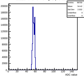
Pedestals mcm50-4812-refv4-g0-s0-p1 ch 88 test1
