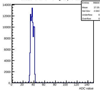
Pedestals mcm50-4812-refv4-g0-s0-p1 ch 33 test1
