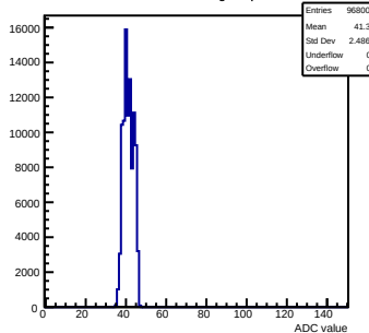
Pedestals mcm50-4812-refv4-g0-s0-p1 ch 10 test1
