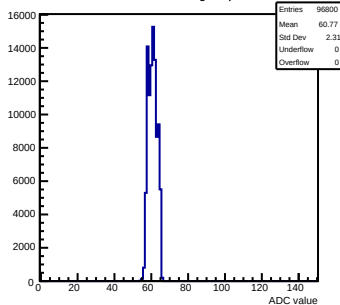
Pedestals mcm50-4812-refv4-g0-s0-p1 ch 13 test1
