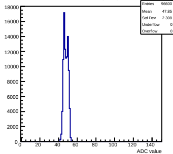
Pedestals mcm50-4812-refv4-g0-s0-p1 ch 37 test1
