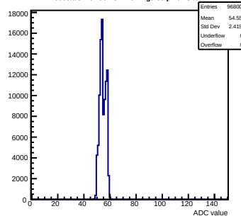
Pedestals mcm50-4812-refv4-g0-s0-p1 ch 3 test1
