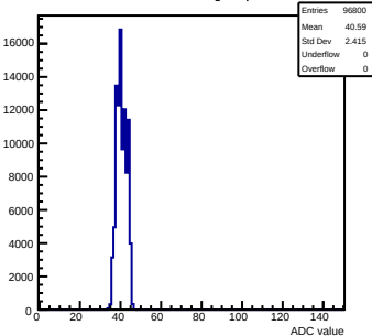
Pedestals mcm50-4812-refv4-g0-s0-p1 ch 12 test1
