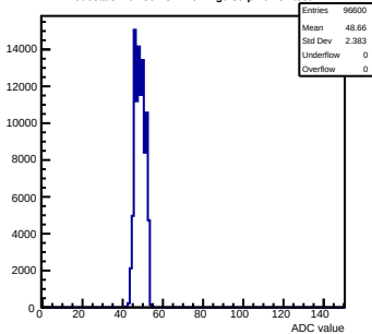
Pedestals mcm50-4812-refv4-g0-s0-p1 ch 32 test1
