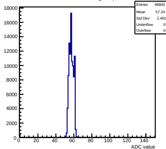
Pedestals mcm50-4812-refv4-g0-s0-p1 ch 9 test1
