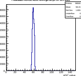
Pedestals mcm50-4812-refv4-g0-s0-p1 ch 121 test1
