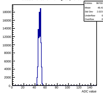
Pedestals mcm50-4812-refv4-g0-s0-p1 ch 90 test1
