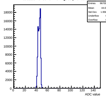
Pedestals mcm50-4812-refv4-g0-s0-p1 ch 95 test1
