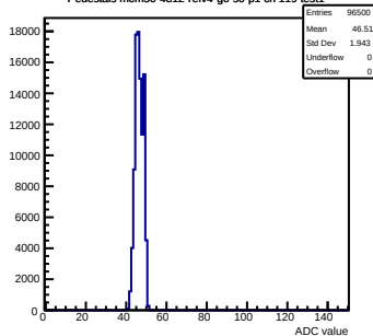
Pedestals mcm50-4812-refv4-g0-s0-p1 ch 119 test1
