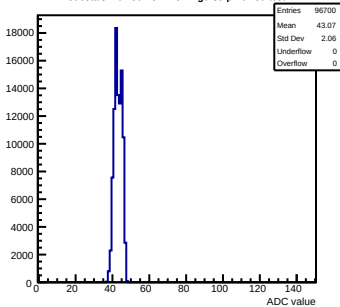
Pedestals mcm50-4812-refv4-g0-s0-p1 ch 89 test1
