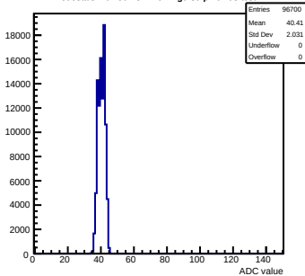
Pedestals mcm50-4812-refv4-g0-s0-p1 ch 93 test1
