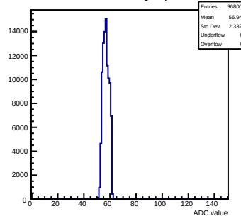
Pedestals mcm50-4812-refv4-g0-s0-p1 ch 15 test1
