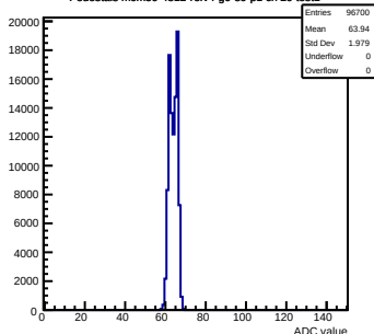
Pedestals mcm50-4812-refv4-g0-s0-p1 ch 29 test1
