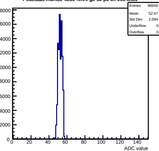
Pedestals mcm50-4812-refv4-g0-s0-p1 ch 113 test1
