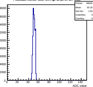
Pedestals mcm50-4812-refv4-g0-s0-p1 ch 117 test1
