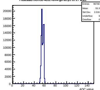
Pedestals mcm50-4812-refv4-g0-s0-p1 ch 27 test1
