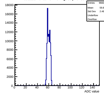
Pedestals mcm50-4812-refv4-g0-s0-p1 ch 35 test1
