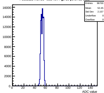
Pedestals mcm50-4812-refv4-g0-s0-p1 ch 18 test1
