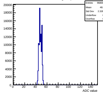
Pedestals mcm50-4812-refv4-g0-s0-p1 ch 11 test1
