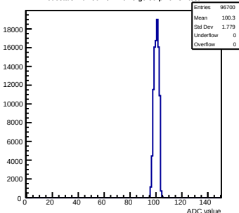
Pedestals mcm50-4812-refV5-g0-s0-p1 ch 31 test1
