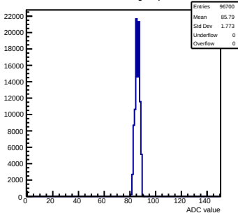
Pedestals mcm50-4812-refv5-g0-s0-p1 ch 88 test1
