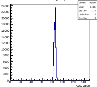
Pedestals mcm50-4812-refv5-g0-s0-p1 ch 85 test1
