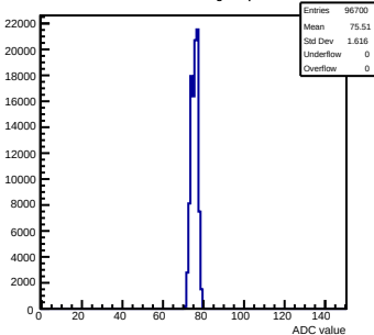
Pedestals mcm50-4812-refv5-g0-s0-p1 ch 95 test1
