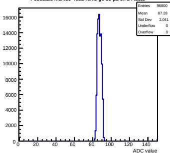
Pedestals mcm50-4812-rtv5-g0-s0-p1 ch 14 test1
