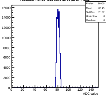
Pedestals mcm50-4812-rtv5-g0-s0-p1 ch 4 test1
