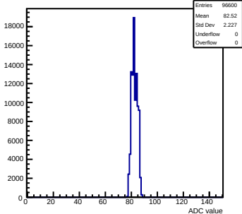
Pedestals mcm50-4812-refV5-g0-s0-p1 ch 104 test1
