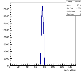
Pedestals mcm50-4812-refV5-g0-s0-p1 ch 107 test1
