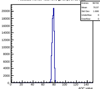
Pedestals mcm50-4812-refV5-g0-s0-p1 ch 22 test1
