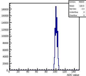
Pedestals mcm50-4812-refV5-g0-s0-p1 ch 96 test1
