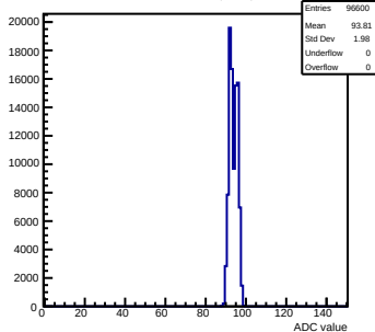
Pedestals mcm50-4812-refV5-g0-s0-p1 ch 97 test1
