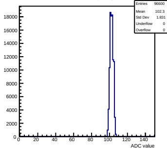
Pedestals mcm50-4812-refV5-g0-s0-p1 ch 98 test1
