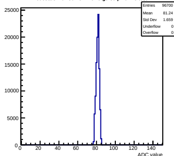
Pedestals mcm50-4812-refV5-g0-s0-p1 ch 21 test1
