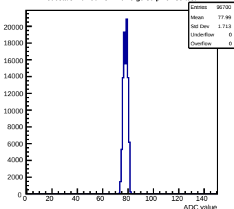
Pedestals mcm50-4812-refV5-g0-s0-p1 ch 30 test1
