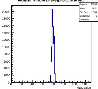
Pedestals mcm50-4812-refV5-g0-s0-p1 ch 39 test1
