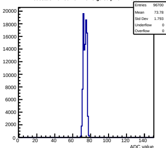
Pedestals mcm50-4812-refV5-g0-s0-p1 ch 20 test1
