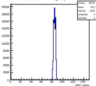
Pedestals mcm50-4812-refV5-g0-s0-p1 ch 26 test1
