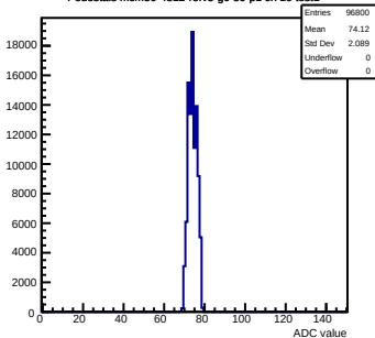
Pedestals mcm50-4812-rtv5-g0-s0-p1 ch 10 test1
