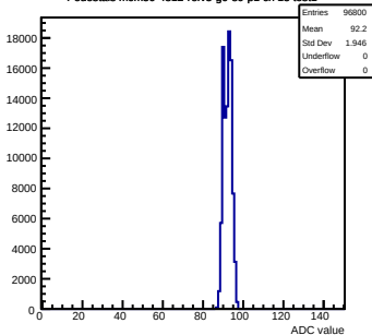
Pedestals mcm50-4812-rtv5-g0-s0-p1 ch 13 test1
