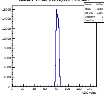
Pedestals mcm50-4812-refV5-g0-s0-p1 ch 43 test1
