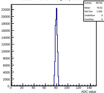
Pedestals mcm50-4812-refv5-g0-s0-p1 ch 83 test1
