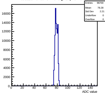
Pedestals mcm50-4812-refV5-g0-s0-p1 ch 16 test1
