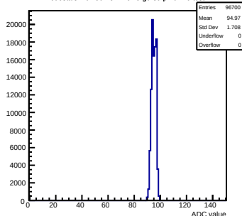
Pedestals mcm50-4812-refV5-g0-s0-p1 ch 29 test1
