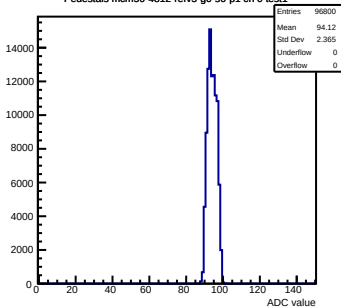
Pedestals mcm50-4812-rtv5-g0-s0-p1 ch 0 test1
