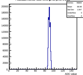
Pedestals mcm50-4812-rtv5-g0-s0-p1 ch 1 test1
