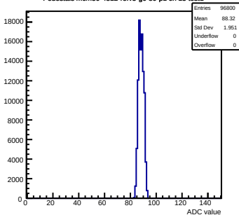
Pedestals mcm50-4812-rtv5-g0-s0-p1 ch 15 test1
