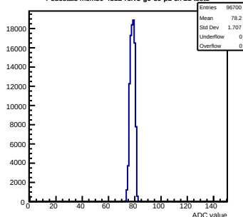
Pedestals mcm50-4812-refV5-g0-s0-p1 ch 17 test1
