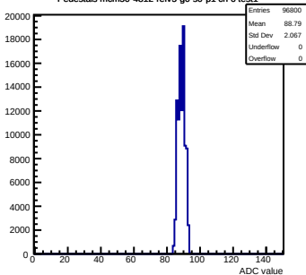
Pedestals mcm50-4812-rtv5-g0-s0-p1 ch 6 test1
