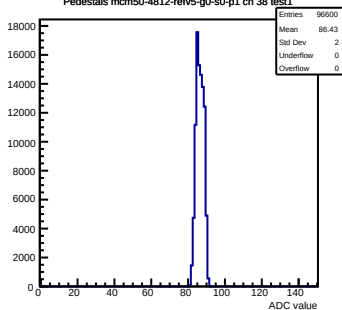
Pedestals mcm50-4812-refV5-g0-s0-p1 ch 38 test1
