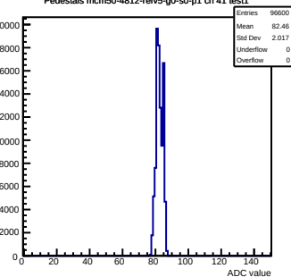
Pedestals mcm50-4812-refV5-g0-s0-p1 ch 41 test1
