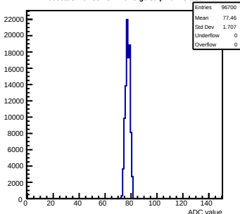
Pedestals mcm50-4812-refV5-g0-s0-p1 ch 28 test1
