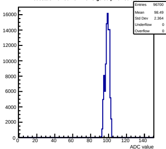
Pedestals mcm50-4812-refv5-g0-s0-p1 ch 80 test1
