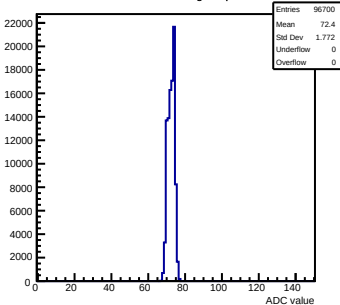
Pedestals mcm50-4812-refv5-g0-s0-p1 ch 94 test1
