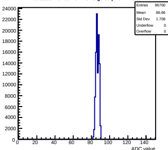
Pedestals mcm50-4812-refV5-g0-s0-p1 ch 27 test1
