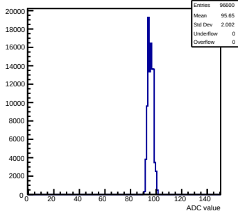
Pedestals mcm50-4812-refV5-g0-s0-p1 ch 105 test1
