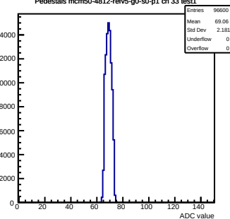
Pedestals mcm50-4812-refV5-g0-s0-p1 ch 33 test1
