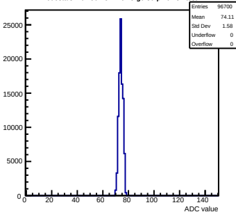
Pedestals mcm50-4812-refv5-g0-s0-p1 ch 87 test1
