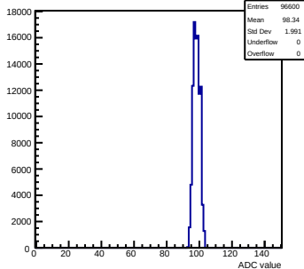
Pedestals mcm50-4812-refV5-g0-s0-p1 ch 110 test1
