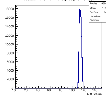
Pedestals mcm50-4812-refv6-g0-s0-p1 ch 107 test1
