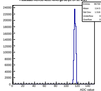
Pedestals mcm50-4812-refv6-g0-s0-p1 ch 91 test1
