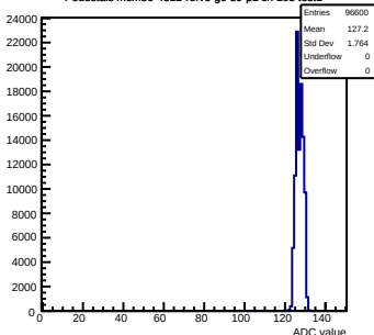
Pedestals mcm50-4812-refv6-g0-s0-p1 ch 108 test1
