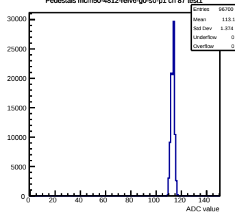
Pedestals mcm50-4812-refv6-g0-s0-p1 ch 87 test1
