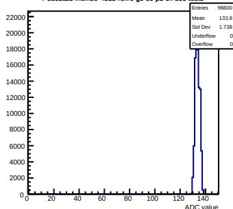
Pedestals mcm50-4812-refv6-g0-s0-p1 ch 105 test1
