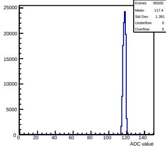
Pedestals mcm50-4812-refv6-g0-s0-p1 ch 119 test1
