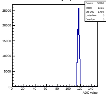
Pedestals mcm50-4812- rev6-g0-s0-p1 ch 28 test1
