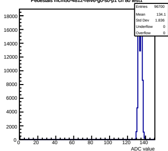
Pedestals mcm50-4812-refv6-g0-s0-p1 ch 80 test1
