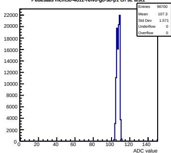
Pedestals mcm50-4812-refv6-g0-s0-p1 ch 92 test1
