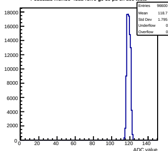
Pedestals mcm50-4812-refv6-g0-s0-p1 ch 109 test1
