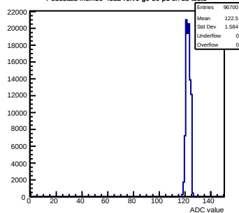
Pedestals mcm50-4812- rev6-g0-s0-p1 ch 18 test1
