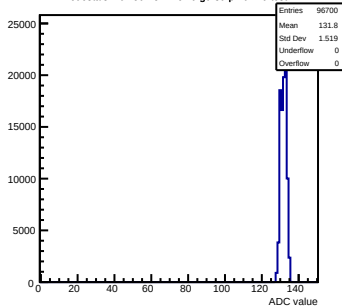
Pedestals mcm50-4812- rev6-g0-s0-p1 ch 29 test1
