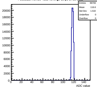
Pedestals mcm50-4812- rev6-g0-s0-p1 ch 21 test1
