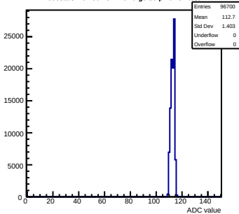
Pedestals mcm50-4812-refV0-g0-s0-p1 ch 87 test1
