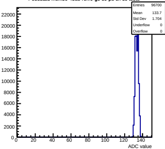
Pedestals mcm50-4812-refV0-g0-s0-p1 ch 80 test1
