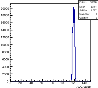
Pedestals mcm50-4812-refV0-g0-s0-p1 ch 32 test1
