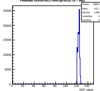
Pedestals mcm50-4812-rev0-g0-s0-p1 ch 7 test1
