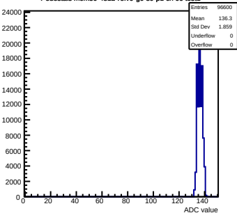
Pedestals mcm50-4812-refV0-g0-s0-p1 ch 96 test1
