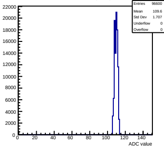
Pedestals mcm50-4812-refV0-g0-s0-p1 ch 34 test1
