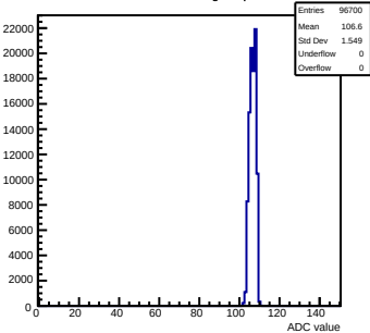
Pedestals mcm50-4812-refV0-g0-s0-p1 ch 92 test1
