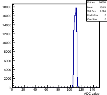
Pedestals mcm50-4812-refV0-g0-s0-p1 ch 33 test1
