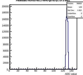
Pedestals mcm50-4812-rev0-g0-s0-p1 ch 5 test1
