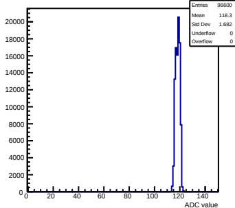
Pedestals mcm50-4812-refV0-g0-s0-p1 ch 43 test1
