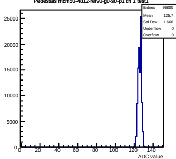
Pedestals mcm50-4812-rev0-g0-s0-p1 ch 1 test1
