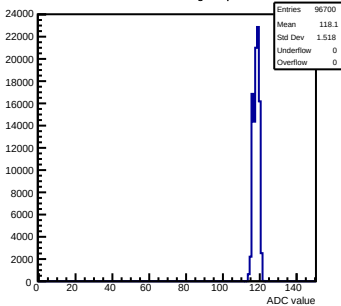
Pedestals mcm50-4812-refV0-g0-s0-p1 ch 90 test1
