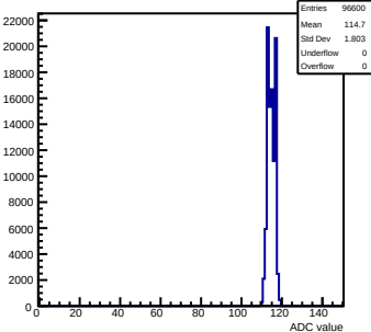
Pedestals mcm50-4812-refV0-g0-s0-p1 ch 40 test1
