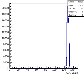
Pedestals mcm50-4812-refV0-g0-s0-p1 ch 35 test1
