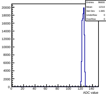
Pedestals mcm50-4812-refV0-g0-s0-p1 ch 38 test1
