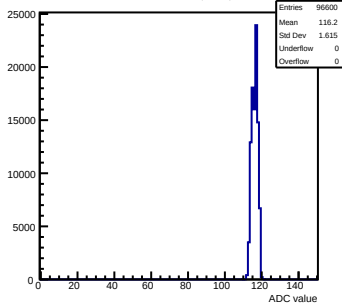
Pedestals mcm50-4812-refV0-g0-s0-p1 ch 39 test1
