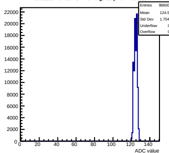
Pedestals mcm50-4812-refV0-g0-s0-p1 ch 106 test1
