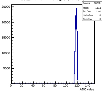
Pedestals mcm50-4812-refV0-g0-s0-p1 ch 83 test1
