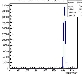
Pedestals mcm50-4812-refV0-g0-s0-p1 ch 102 test1
