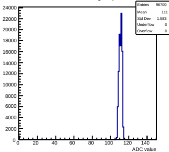
Pedestals mcm50-4812-refV0-g0-s0-p1 ch 94 test1
