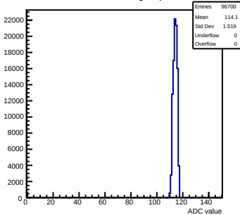
Pedestals mcm50-4812-refV0-g0-s0-p1 ch 91 test1
