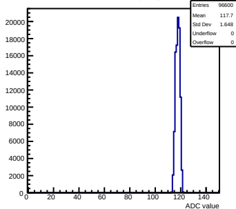
Pedestals mcm50-4812-refV0-g0-s0-p1 ch 37 test1
