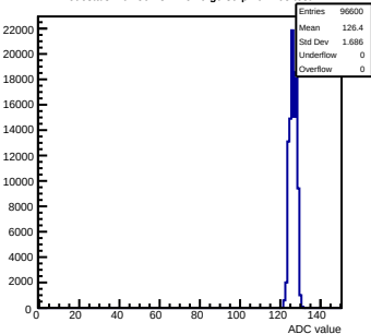
Pedestals mcm50-4812-refV0-g0-s0-p1 ch 108 test1
