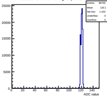
Pedestals mcm50-4812-refV0-g0-s0-p1 ch 86 test1
