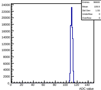
Pedestals mcm50-4812-refV0-g0-s0-p1 ch 46 test1
