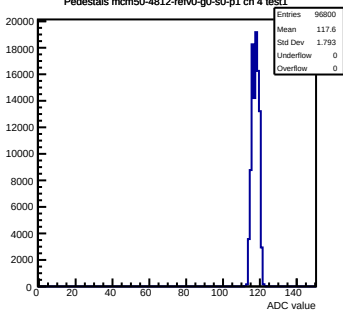
Pedestals mcm50-4812-rev0-g0-s0-p1 ch 4 test1
