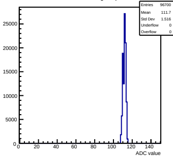
Pedestals mcm50-4812-refV0-g0-s0-p1 ch 93 test1
