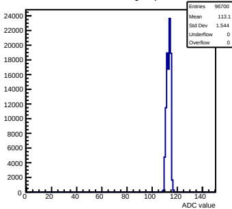
Pedestals mcm50-4812-refV0-g0-s0-p1 ch 89 test1
