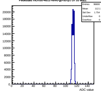
Pedestals mcm50-4812-rev0-g0-s0-p1 ch 10 test1
