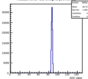
Pedestals mcm50-4812-ref2-g0-s0-p1 ch 98 test1
