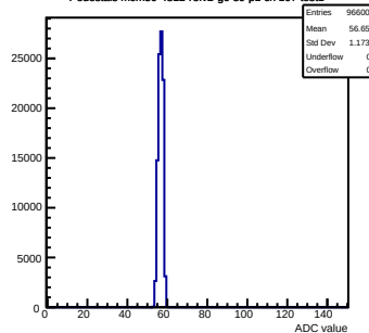
Pedestals mcm50-4812-ref2-g0-s0-p1 ch 107 test1
