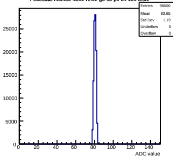
Pedestals mcm50-4812-ref2-g0-s0-p1 ch 101 test1
