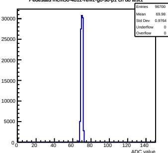
Pedestals mcm50-4812-refV2-g0-s0-p1 ch 88 test1
