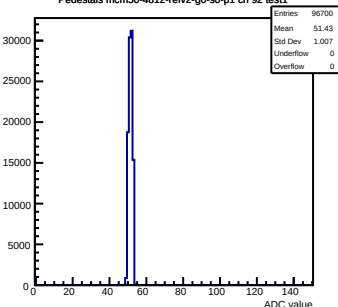
Pedestals mcm50-4812-refV2-g0-s0-p1 ch 92 test1
