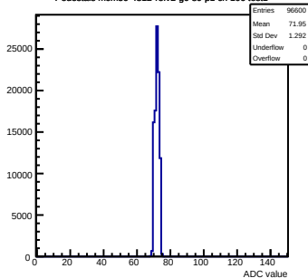
Pedestals mcm50-4812-ref2-g0-s0-p1 ch 102 test1
