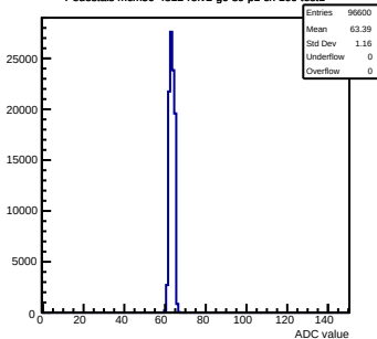
Pedestals mcm50-4812-ref2-g0-s0-p1 ch 109 test1
