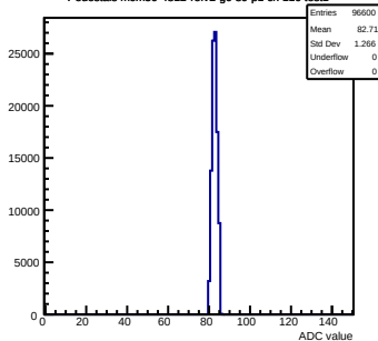
Pedestals mcm50-4812-ref2-g0-s0-p1 ch 110 test1
