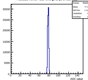
Pedestals mcm50-4812-ref2-g0-s0-p1 ch 111 test1
