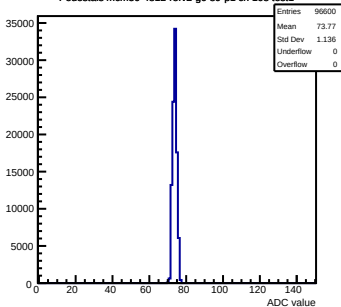
Pedestals mcm50-4812-ref2-g0-s0-p1 ch 108 test1
