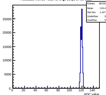
Pedestals mcm50-4812- rev6-g0-s0-p1 ch 90 test1
