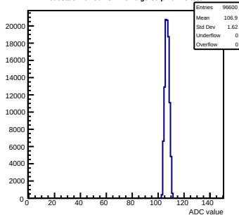
Pedestals mcm50-4812- rev6-g0-s0-p1 ch 45 test1
