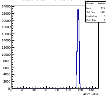
Pedestals mcm50-4812- rev6-g0-s0-p1 ch 89 test1
