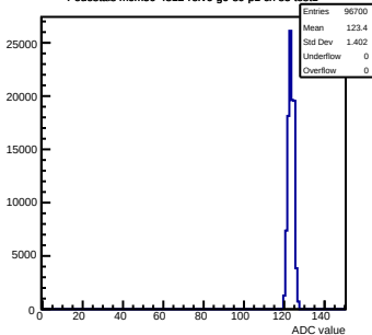
Pedestals mcm50-4812- rev6-g0-s0-p1 ch 85 test1
