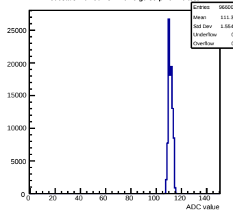
Pedestals mcm50-4812- rev6-g0-s0-p1 ch 46 test1
