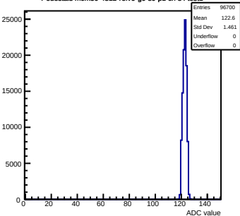
Pedestals mcm50-4812- rev6-g0-s0-p1 ch 84 test1
