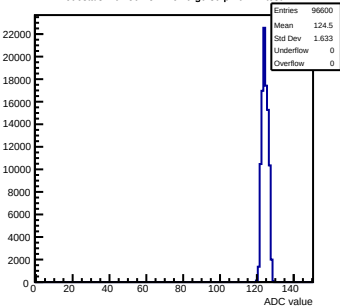
Pedestals mcm50-4812- rev6-g0-s0-p1 ch 44 test1
