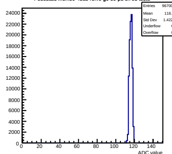
Pedestals mcm50-4812- rev6-g0-s0-p1 ch 95 test1
