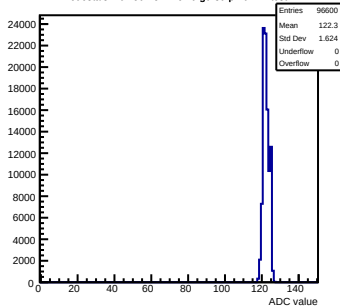
Pedestals mcm50-4812- rev6-g0-s0-p1 ch 41 test1
