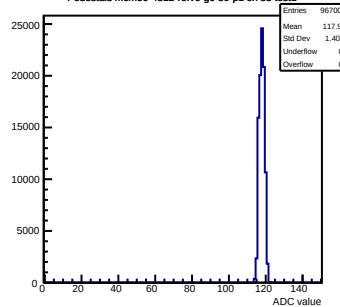
Pedestals mcm50-4812- rev6-g0-s0-p1 ch 83 test1
