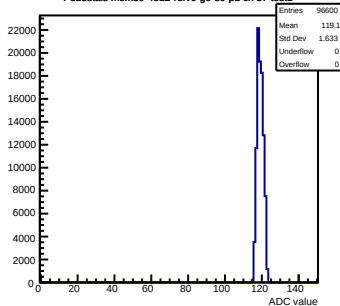
Pedestals mcm50-4812- rev6-g0-s0-p1 ch 37 test1
