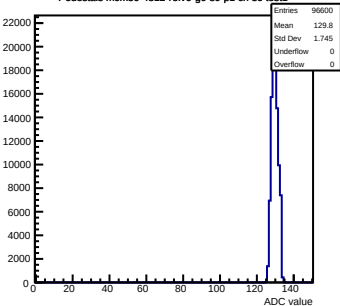
Pedestals mcm50-4812- rev6-g0-s0-p1 ch 36 test1
