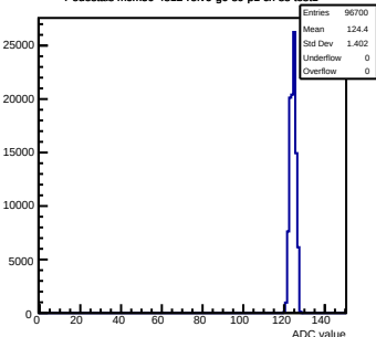
Pedestals mcm50-4812- rev6-g0-s0-p1 ch 88 test1
