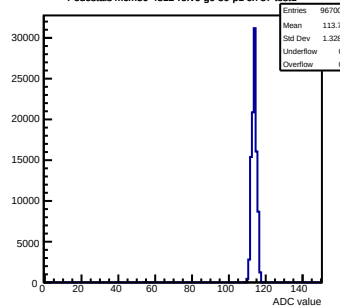
Pedestals mcm50-4812- rev6-g0-s0-p1 ch 87 test1
