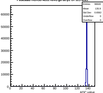
Pedestals mcm50-4812-refV0-g0-s0-p1 ch 125 test1
