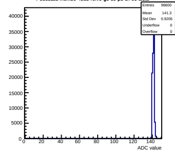
Pedestals mcm50-4812-refV0-g0-s0-p1 ch 96 test1
