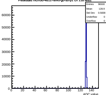
Pedestals mcm50-4812-refV0-g0-s0-p1 ch 118 test1
