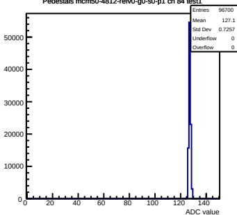
Pedestals mcm50-4812-refV0-g0-s0-p1 ch 84 test1
