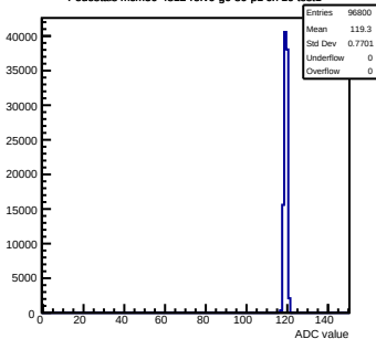
Pedestals mcm50-4812-refv0-g0-s0-p1 ch 10 test1
