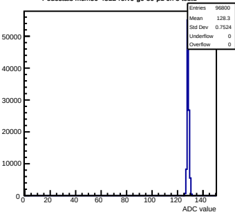
Pedestals mcm50-4812-refv0-g0-s0-p1 ch 8 test1
