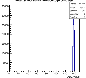
Pedestals mcm50-4812-refV0-g0-s0-p1 ch 80 test1
