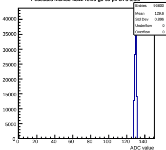
Pedestals mcm50-4812-refv0-g0-s0-p1 ch 3 test1
