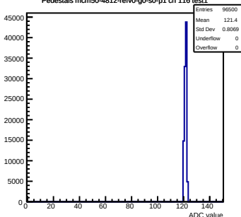
Pedestals mcm50-4812-refV0-g0-s0-p1 ch 116 test1
