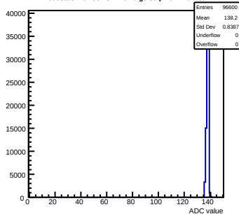
Pedestals mcm50-4812-refV0-g0-s0-p1 ch 110 test1
