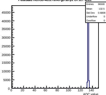
Pedestals mcm50-4812-refV0-g0-s0-p1 ch 127 test1
