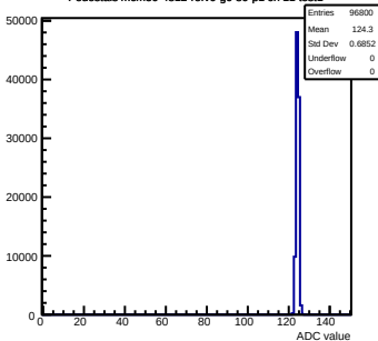
Pedestals mcm50-4812-refv0-g0-s0-p1 ch 11 test1
