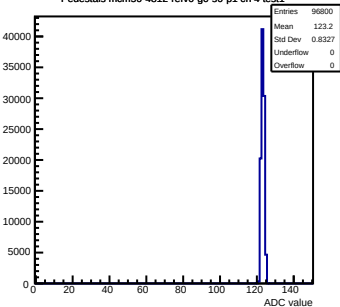
Pedestals mcm50-4812-refv0-g0-s0-p1 ch 4 test1
