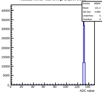
Pedestals mcm50-4812-refv0-g0-s0-p1 ch 9 test1
