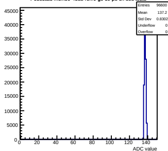
Pedestals mcm50-4812-refV0-g0-s0-p1 ch 101 test1
