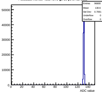
Pedestals mcm50-4812-refv0-g0-s0-p1 ch 15 test1
