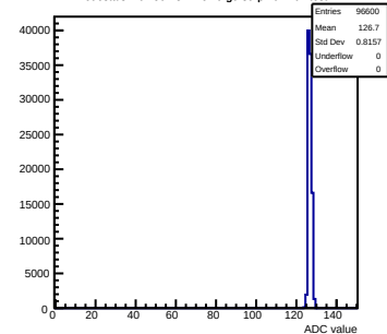
Pedestals mcm50-4812-refV0-g0-s0-p1 ch 104 test1
