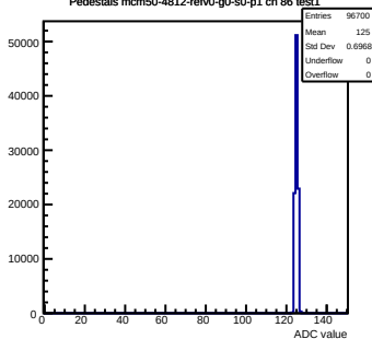
Pedestals mcm50-4812-refV0-g0-s0-p1 ch 86 test1
