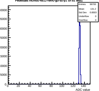
Pedestals mcm50-4812-refV0-g0-s0-p1 ch 81 test1
