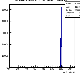
Pedestals mcm50-4812-refV0-g0-s0-p1 ch 94 test1
