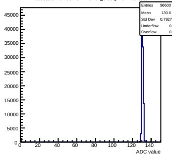
Pedestals mcm50-4812-refV0-g0-s0-p1 ch 106 test1
