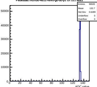
Pedestals mcm50-4812-refV0-g0-s0-p1 ch 121 test1
