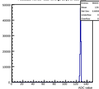
Pedestals mcm50-4812-refV0-g0-s0-p1 ch 102 test1
