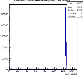
Pedestals mcm50-4812-refV0-g0-s0-p1 ch 115 test1
