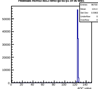
Pedestals mcm50-4812-refV0-g0-s0-p1 ch 90 test1
