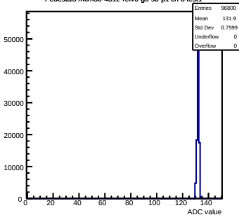
Pedestals mcm50-4812-refv0-g0-s0-p1 ch 6 test1
