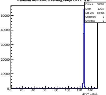
Pedestals mcm50-4812-refV0-g0-s0-p1 ch 117 test1
