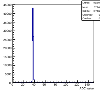
Pedestals mcm50-4812-refv3-g0-s0-p1 ch 90 test1
