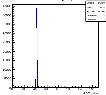
Pedestals mcm50-4812-refv3-g0-s0-p1 ch 85 test1
