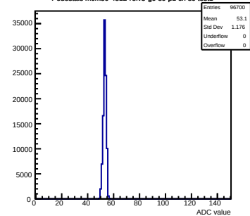
Pedestals mcm50-4812-refv3-g0-s0-p1 ch 80 test1
