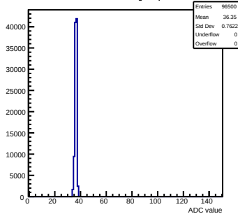
Pedestals mcm50-4812-refv3-g0-s0-p1 ch 126 test1
