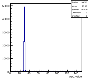
Pedestals mcm50-4812-refv3-g0-s0-p1 ch 93 test1
