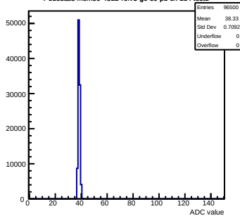
Pedestals mcm50-4812-refv3-g0-s0-p1 ch 114 test1
