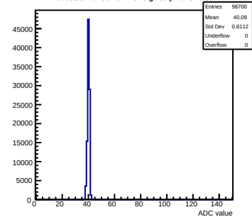
Pedestals mcm50-4812-refv3-g0-s0-p1 ch 84 test1
