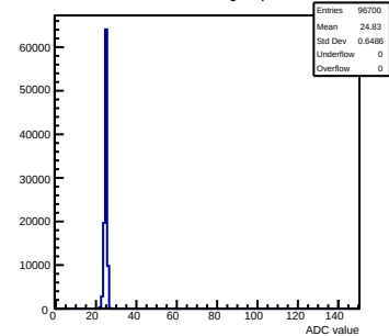
Pedestals mcm50-4812-refv3-g0-s0-p1 ch 92 test1
