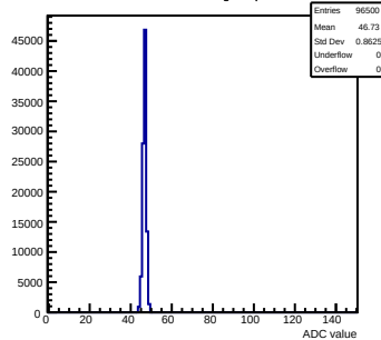
Pedestals mcm50-4812-refv3-g0-s0-p1 ch 127 test1
