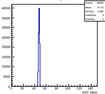
Pedestals mcm50-4812-refv3-g0-s0-p1 ch 124 test1
