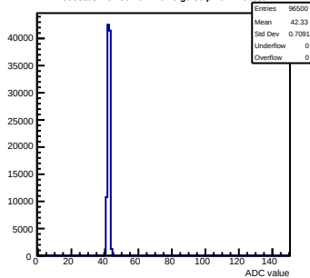
Pedestals mcm50-4812-refv3-g0-s0-p1 ch 118 test1
