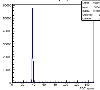
Pedestals mcm50-4812-refv3-g0-s0-p1 ch 119 test1
