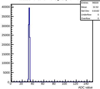
Pedestals mcm50-4812-refv3-g0-s0-p1 ch 116 test1
