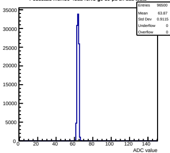
Pedestals mcm50-4812-refv3-g0-s0-p1 ch 112 test1
