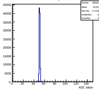
Pedestals mcm50-4812-refv3-g0-s0-p1 ch 123 test1
