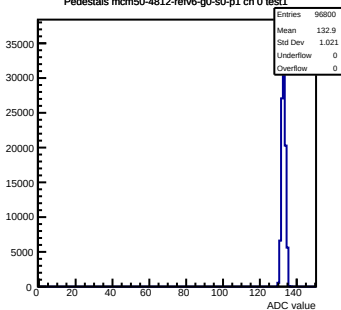
Pedestals mcm50-4812-rlv6-g0-s0-p1 ch 0 test1
