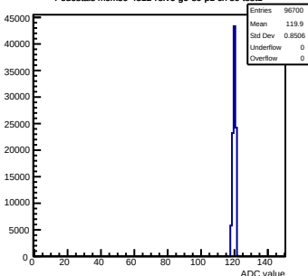
Pedestals mcm50-4812- refv6-g0-s0-p1 ch 89 test1
