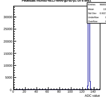
Pedestals mcm50-4812-rlv6-g0-s0-p1 ch 6 test1
