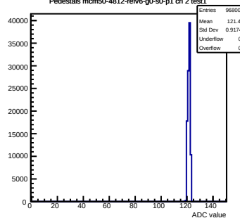
Pedestals mcm50-4812-rlv6-g0-s0-p1 ch 2 test1
