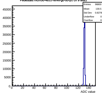
Pedestals mcm50-4812-rlv6-g0-s0-p1 ch 9 test1
