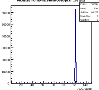
Pedestals mcm50-4812-refv6-g0-s0-p1 ch 116 test1
