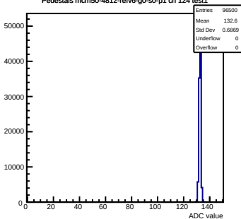
Pedestals mcm50-4812-refv6-g0-s0-p1 ch 124 test1
