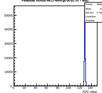
Pedestals mcm50-4812-rlv6-g0-s0-p1 ch 7 test1
