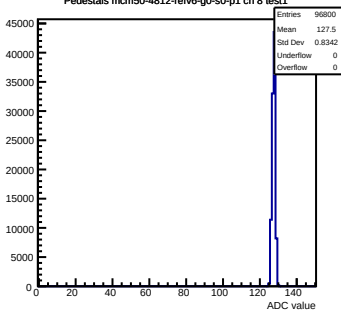
Pedestals mcm50-4812-rlv6-g0-s0-p1 ch 8 test1
